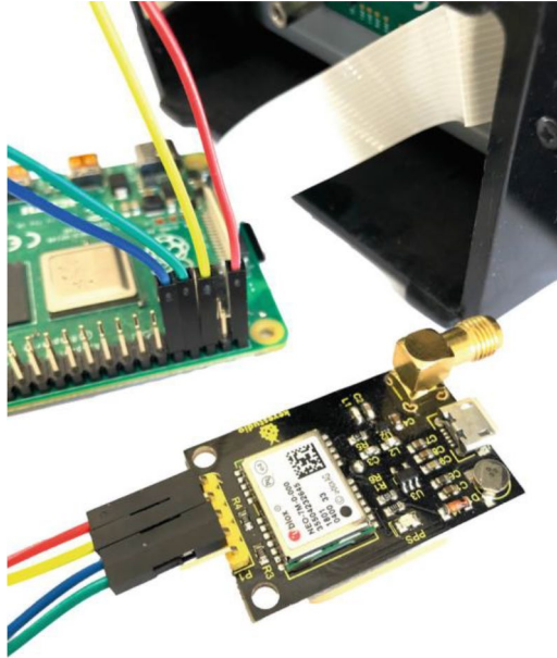
Figure 12-14. GPS and Raspberry Pi 4 Model B GPIO connection
