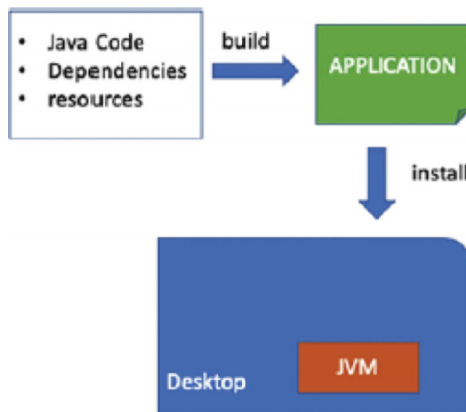
Figure 10-3. Legacy development process
