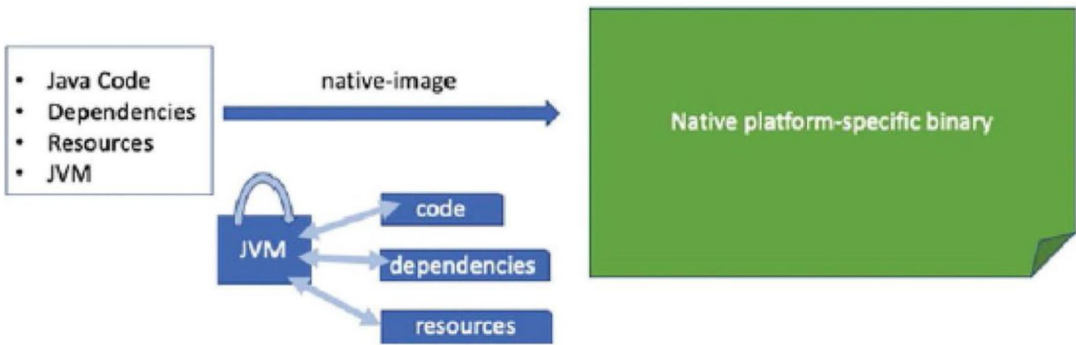
Figure 10-11. Native Image development process
