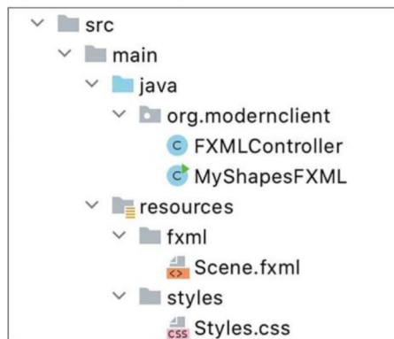
Figure 2-10. MyShapesFXML with FXML and CSS
