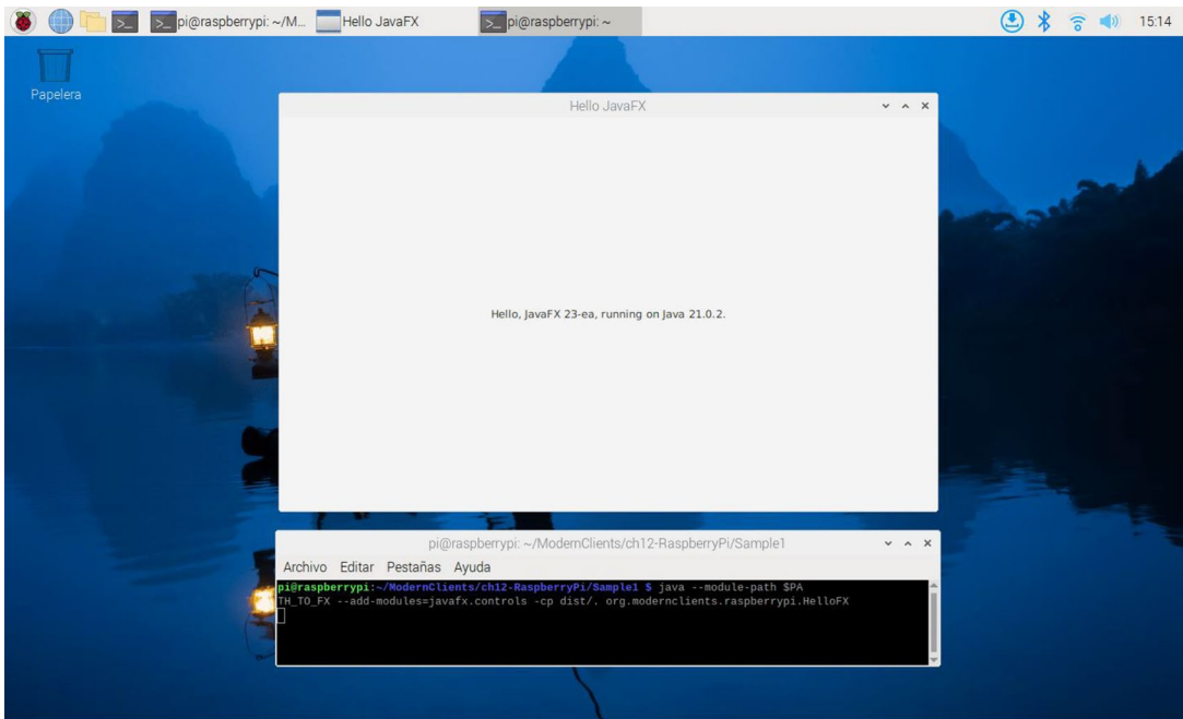
Figure 12-6. Running JavaFX on Wayland
