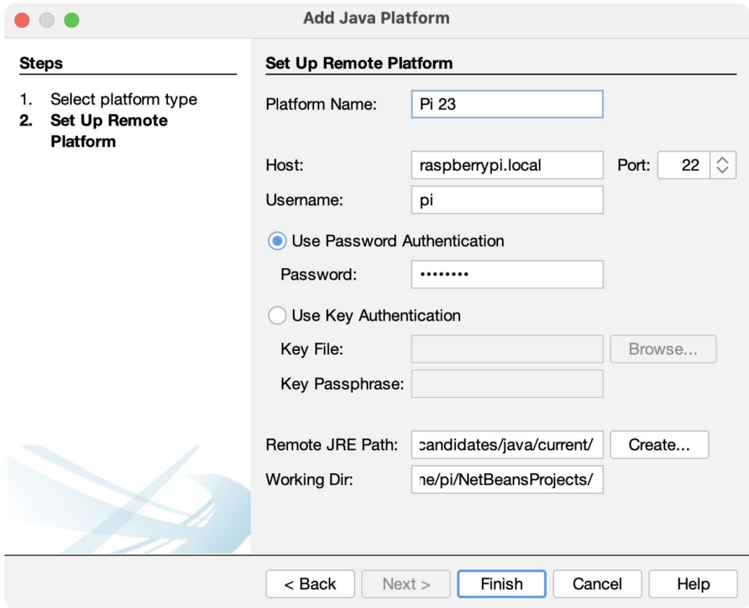
Figure 12-8. Remote platform configuration
