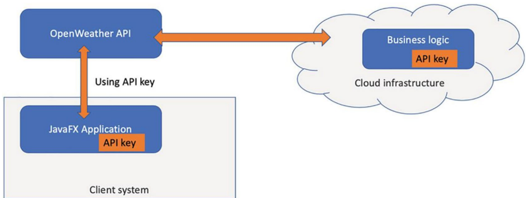
Figure 9-8. The JavaFX application looks similar to code in a backend that accesses external APIs
