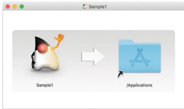
Figure 10-9. Customized installer
