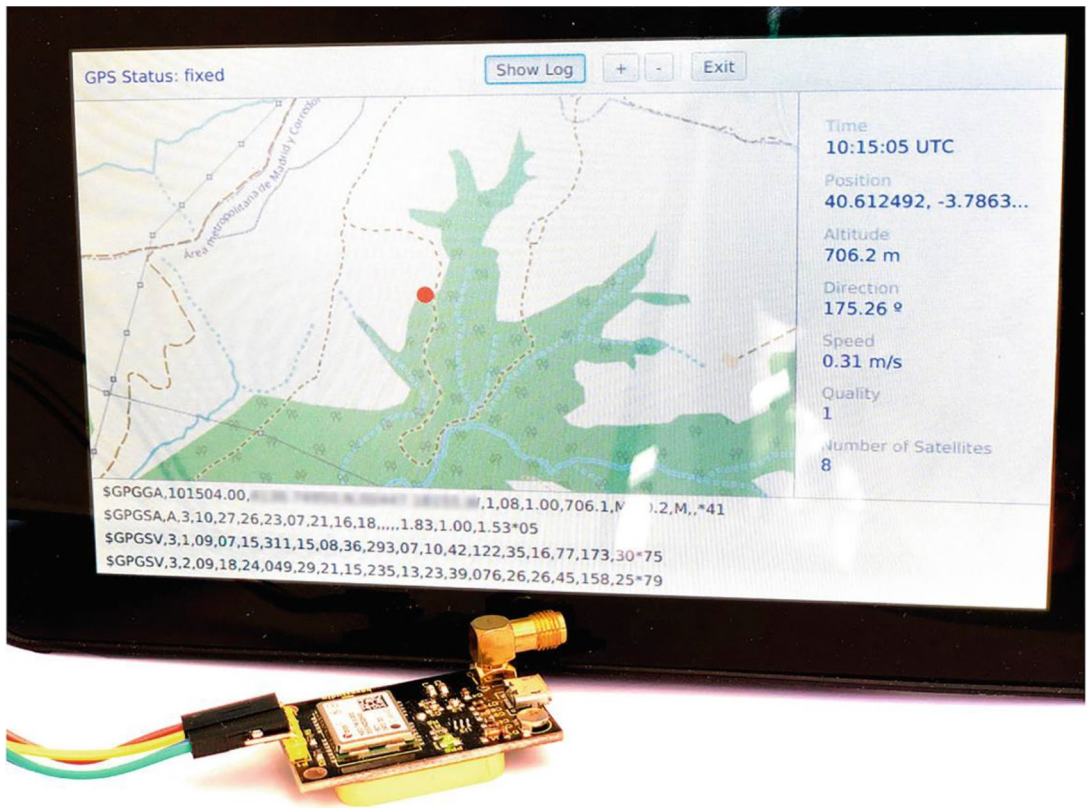
Figure 12-19. DIY in-car navigation system running
