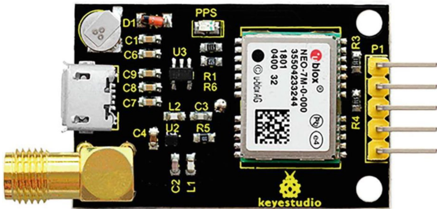
Figure 12-12. UART Serial GPS Neo-7M. Image from http://wiki.keyestudio.com/File:KS0319.png
