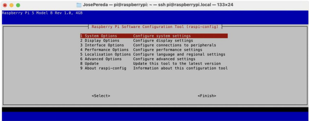
Figure 12-2. Running raspi-config
