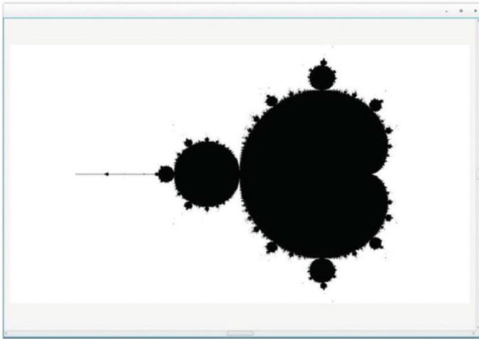
Figure 6-9. Simplest Mandelbrot set
