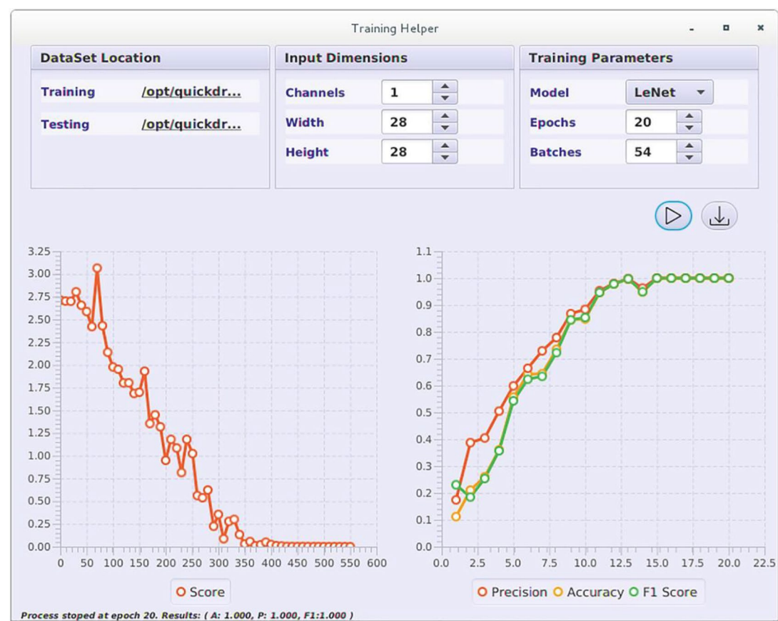
Figure 13-4. A JavaFX application that visualizes the progress of a neural network training process
