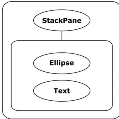
Figure 2-3. MyShapes scene graph
