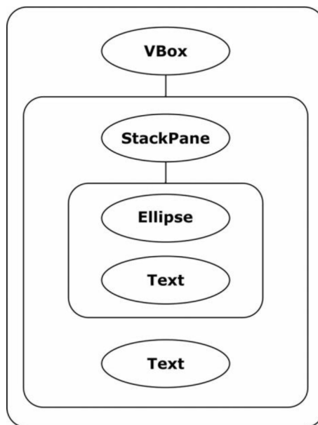
Figure 2-6. MyShapesProperties scene graph
