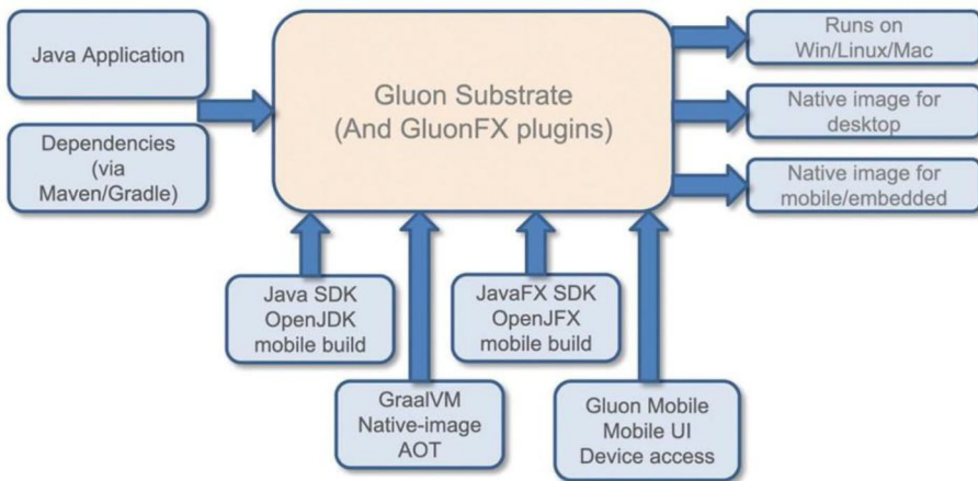
Figure 11-8. Native application workflow
