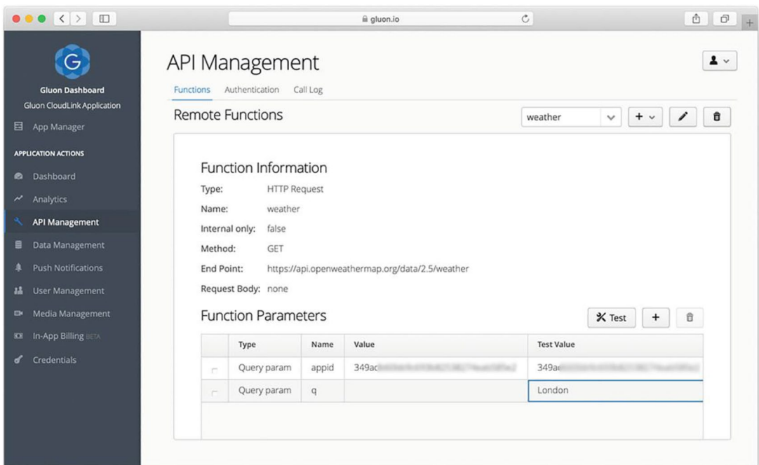
Figure 9-10. Testing the function from the Gluon Dashboard
