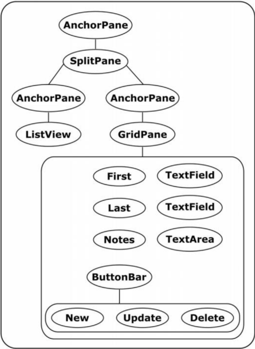
Figure 2-13. Person UI scene graph hierarchy
