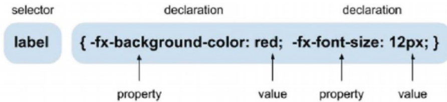
Figure 5-1. Properties and values, the building blocks of CSS
