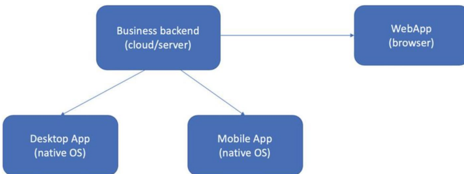
Figure 11-1. Business backend serving different channels
