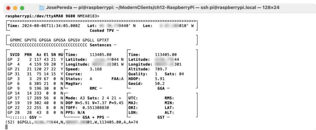
Figure 12-16. gpsd service active and running
