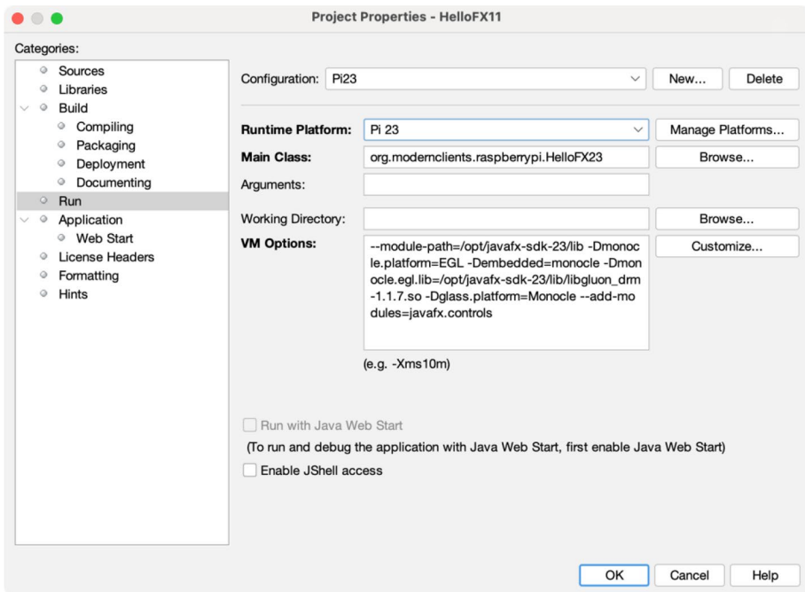
Figure 12-10. Set project properties to run with a remote platform
