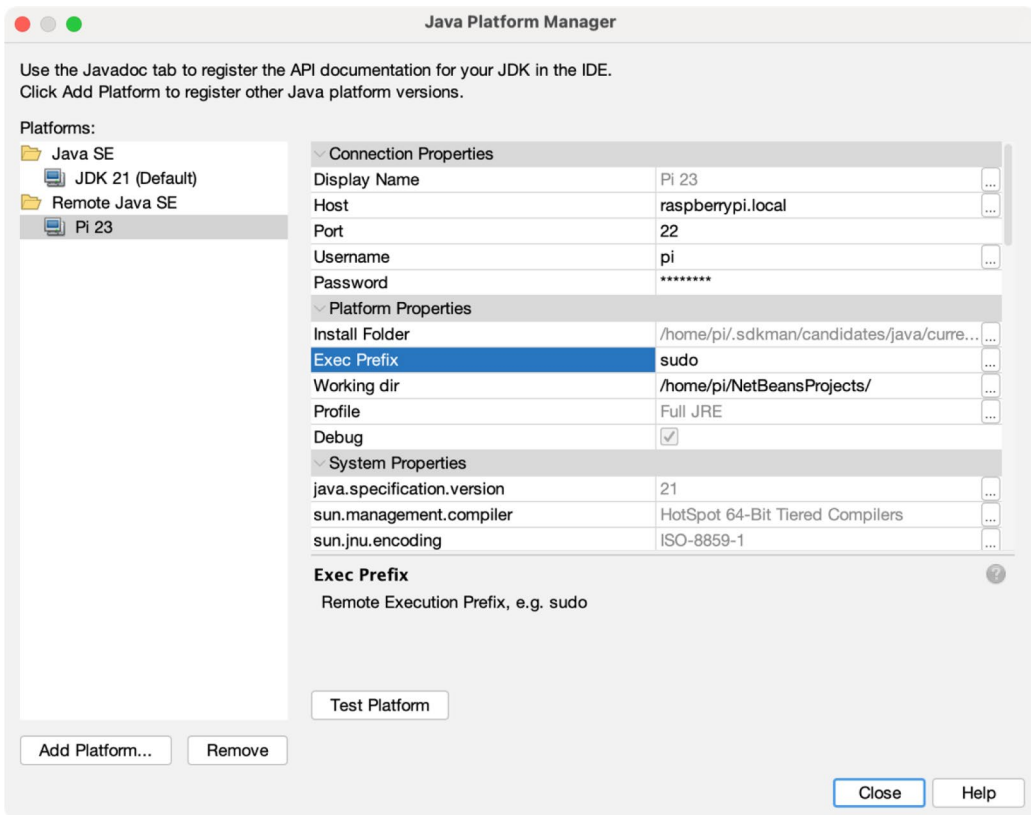
Figure 12-9. Adding exec prefix to the remote platform
