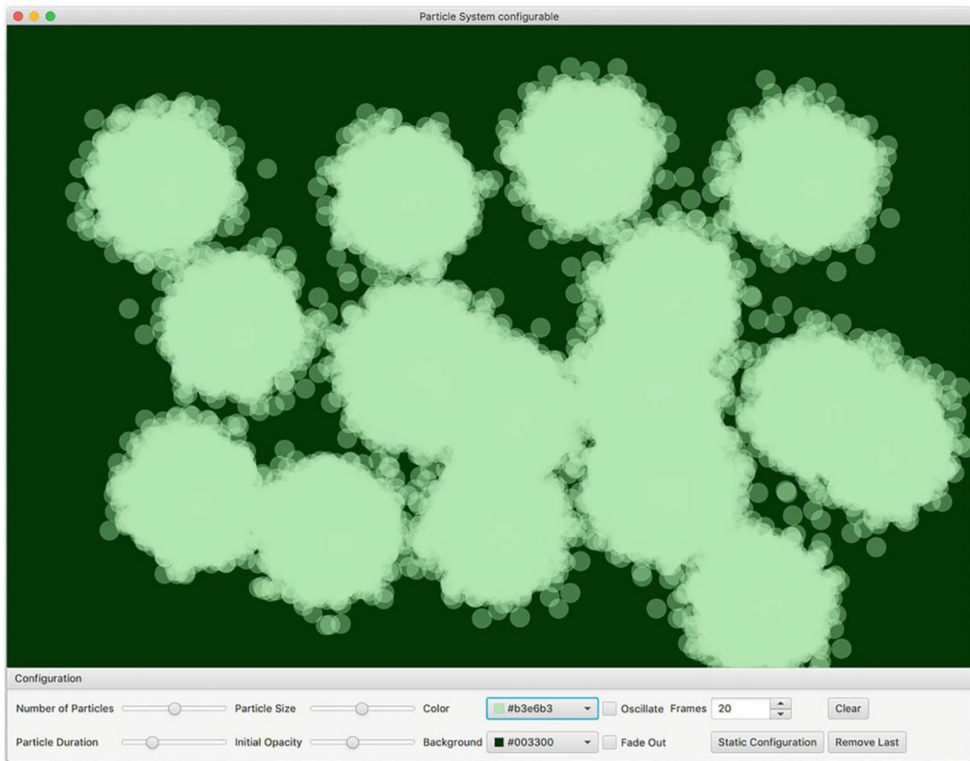
Figure 6-8. Configurable particle system
