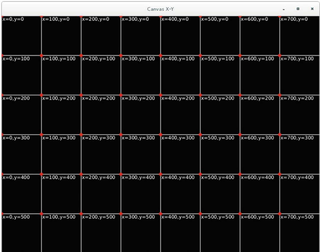
Figure 6-2. This application shows how x and y positions work in a JavaFX canvas
