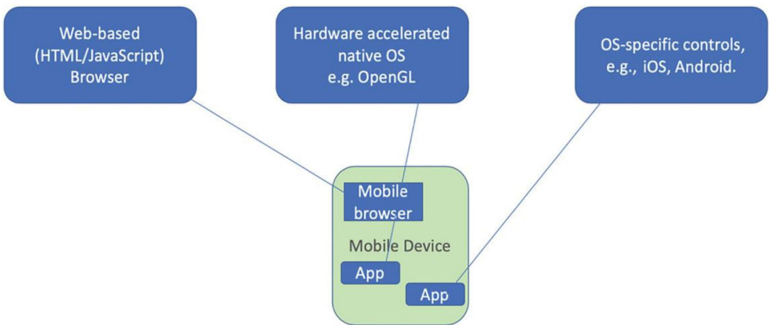
Figure 11-2. Three possible approaches for mobile apps
