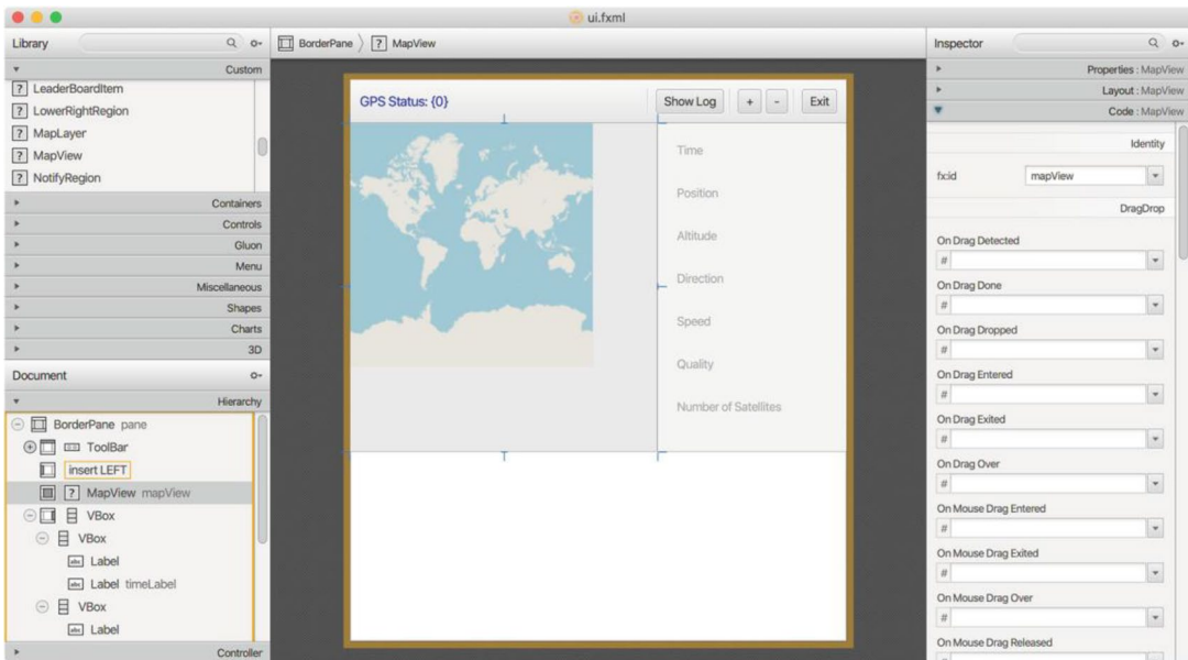
Figure 12-18. Designing the UI in Scene Builder
