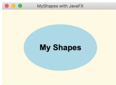
Figure 2-2. MyShapes application
