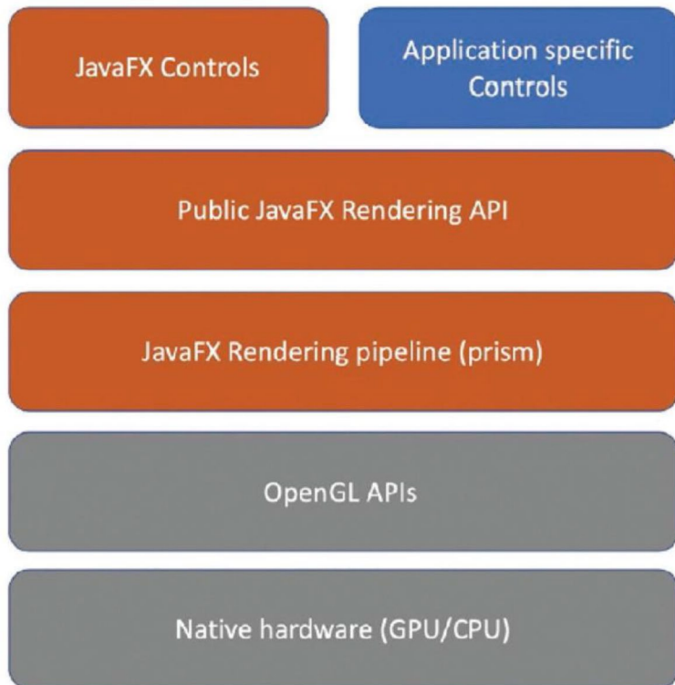
Figure 11-3. JavaFX stack
