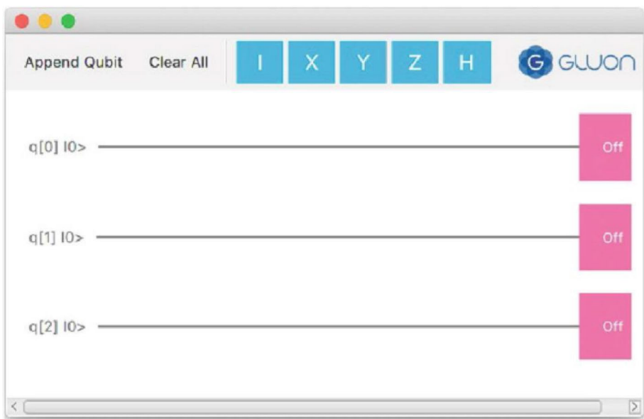
Figure 14-2. StrangeFX allows developers to drag quantum gates onto qubit wires
