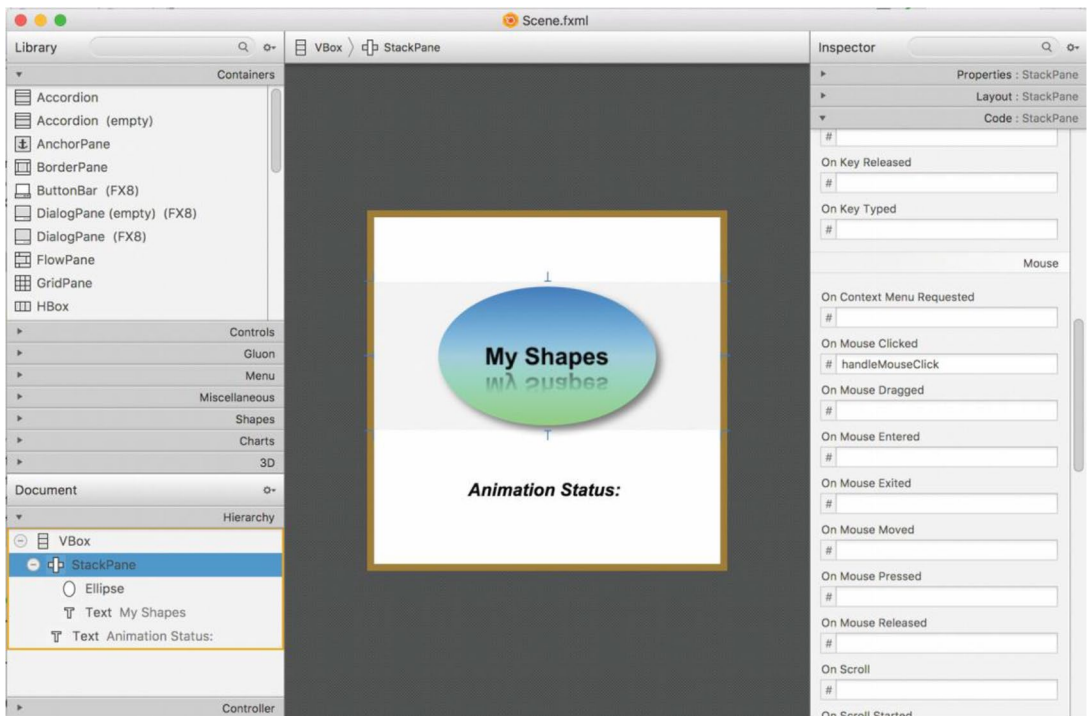
Figure 2-11. FXML file with Scene Builder for MyShapesFXML
