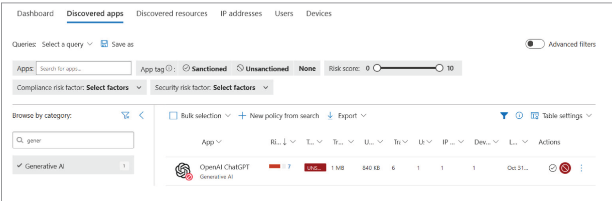
Figure 5.5: Discovered apps
