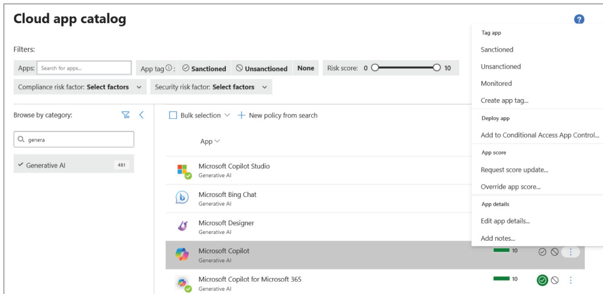
Figure 5.8: Manage application
