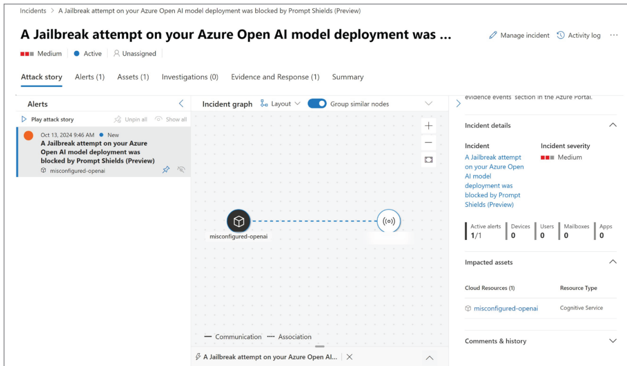
Figure 5.16: Incident view
