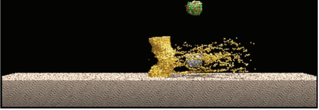
Figure 3.4 Snapshot of a Material Point Method simulation of a ping-pong ball going through a pop can. Grayscale as well as color reveal pressure differences.
