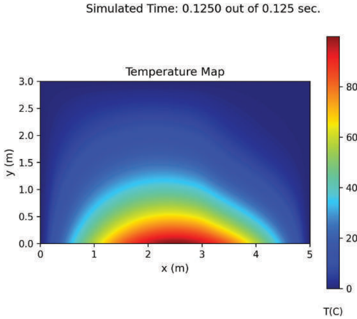
Figure 6.6 Thermal conduction in a rectangular plate on its way toward equilibrium as visualized from frames from an animation created with native Python graphics. Note the asymmetry (present in transient-state) resulting from nonuniform thermal conductivity. Simulation parameters can be found in the examples in the online appendix and POV renderings (not shown here) for the bar are similar.
