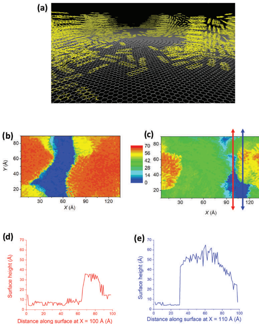
Figure 3.16 Analysis of the fascinating and complicated terrain offered when pentacene condenses out of the gas phase onto a graphene surface including visuals (a), height maps (b,c), and terrain cross sections (d,e). Grayscale as well as color can help delineate information. (He et al. [13]).
