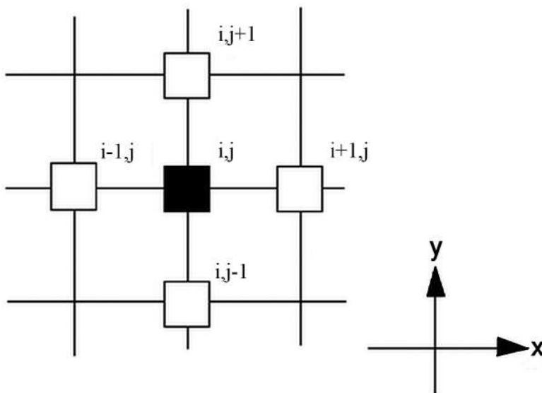
Figure 5.9 Detail of 2D Cartesian finite-difference indexing.
