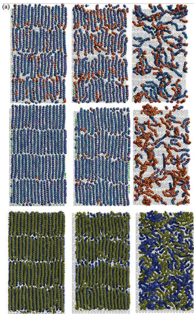
Figure 3.11 (a) Snapshots of the top and bottom layers of Molecular Dynamics simulations of tetracosane on graphite, respectively, at various temperatures. Can you identify the solid, intermediate smectic, and liquid phase? Grayscale as well as color help delineate the following aspects. In the upper two panels, atoms colored red signify that they are significantly higher off the surface relative to their respective layer, and in the bottom panel, upper (green) and lower (blue) layers together (Roth et al. [10]). (b) Initial conditions for the nanoscale Molecular Dynamics rotating disk simulations. Grayscale as well as color help delineate the following aspects. The blue to green gradient color scale represents closest to farthest initial noble gas atom distance from the central fullerene. The purple line of atoms is used to help understand the system's rotational dynamics. (c) Snapshots of final configurations in our orbiting noble gas simulations at low temperature for He (top), Ne (middle), and Ar (bottom) (Maldonado and Roth [12]).
