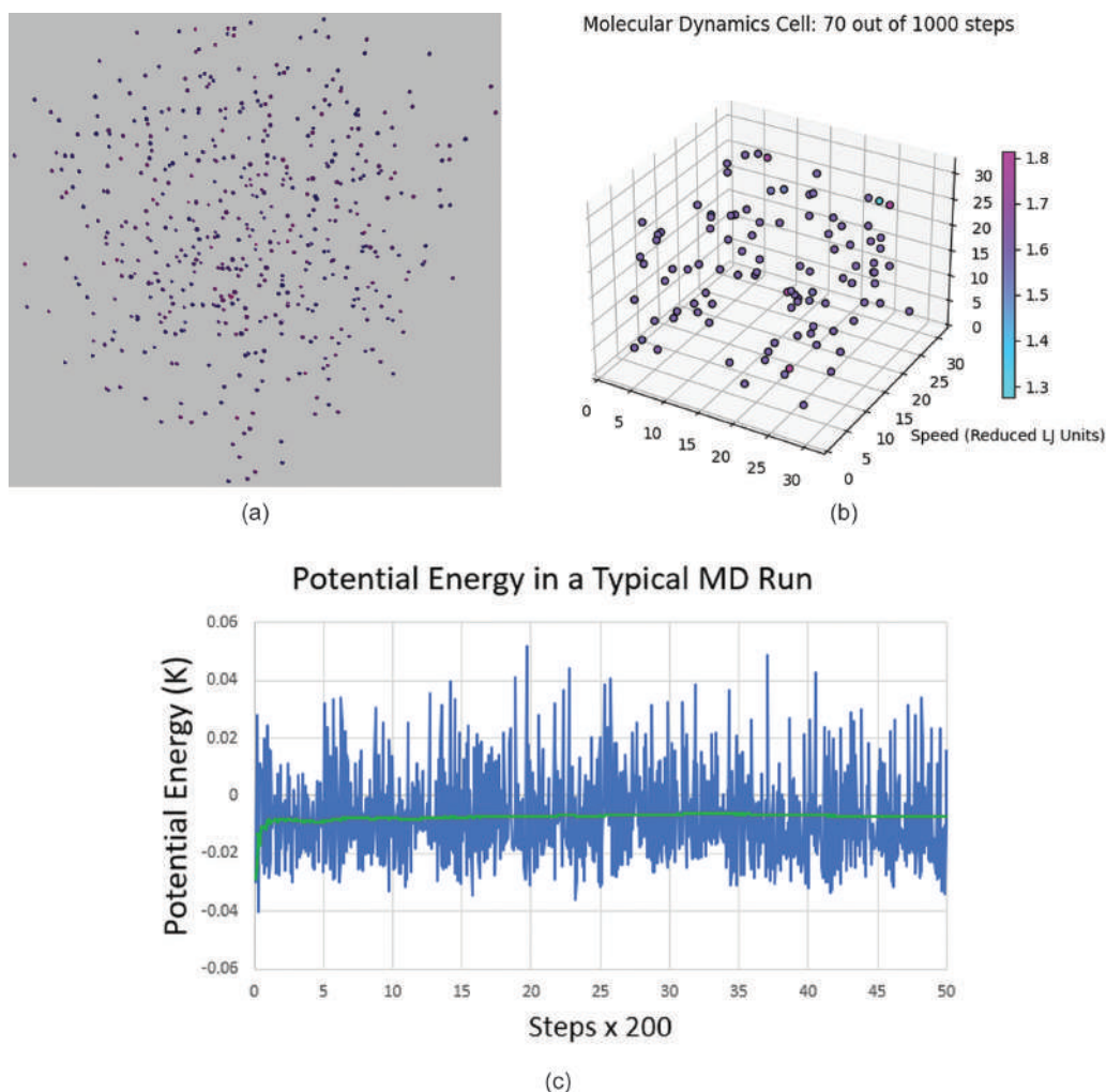
Figure 8.2 (a–c) Visuals of initial MD configurations for (a) C++ and (b) Python versions of the MD code a few steps into the runs so velocity distributions are present. The atoms are color-scaled to speed. Typical energy fluctuations (c) for 10,000 step short example run. (Screenshots by the author.)
