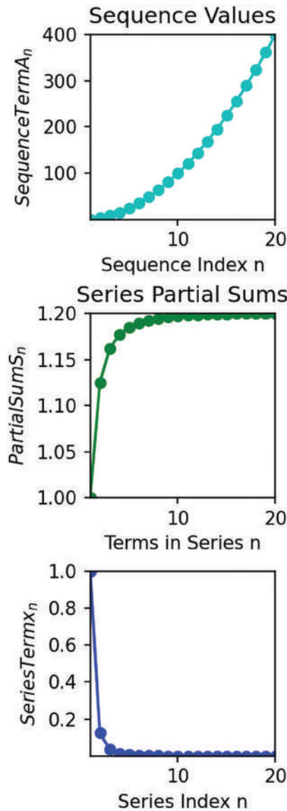
Figure 2.5 Graphical output from Sequences_And_Series_Python_Plot.py for 20 elements in the sequence x_n = n^2 and 20 in the partial series sum x_n = n^{-3} . (Screen capture by the author.)
