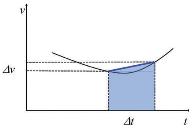
Figure 3.7 Typical velocity vs. time plot with illustrations of slope and area under the curve that lead toward concepts of derivatives and integrals.
