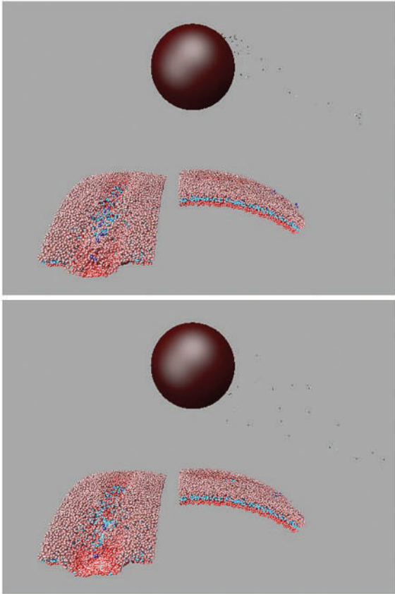
Figure 7.7 Typical configurations from the intermediate stage of impact (upper), after the rapidly moving horizontal ejecta has left, and the late phase of impact where the trench has been carved out, and the forward momentum of objects inside the trench continues to carve it out to some extent (lower). The impacting body as well as Martian topsoil, ice layer, and subsoil (progressively deeper), are delineated by grayscale or color. (Massina et al. [40].)
