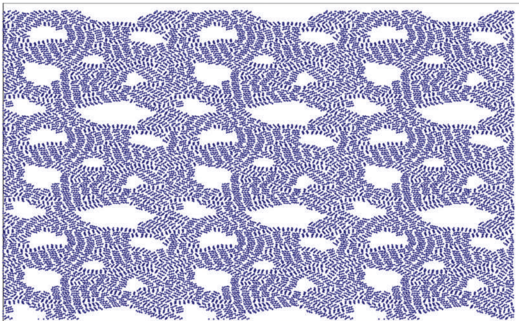
Figure 1.9 Large-scale simulation of hexane on graphite, showing two distinctly different length scales: the molecule–molecule spacing and then the width of domains in the superlattice.
