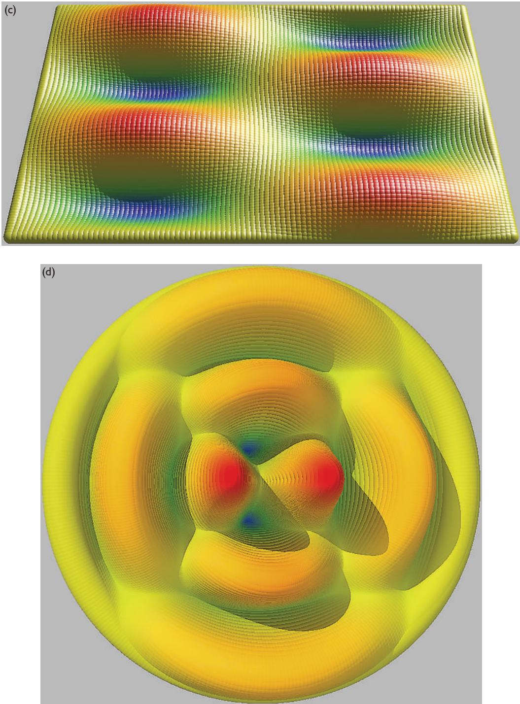
Figure 5.10 (Continued) (a–d). Initial conditions for finite-difference treatments of the rectangular sheet (a) and circular membrane (b), generated by native Python graphics. Corresponding POV visuals are shown in (c) and (d). When the Fourier eigenfunction solution is included, the POV-generating codes will show both the finite-difference and Fourier eigenfunction treatments for comparison. Further results, including simulation parameters, can be found in the online appendix.
