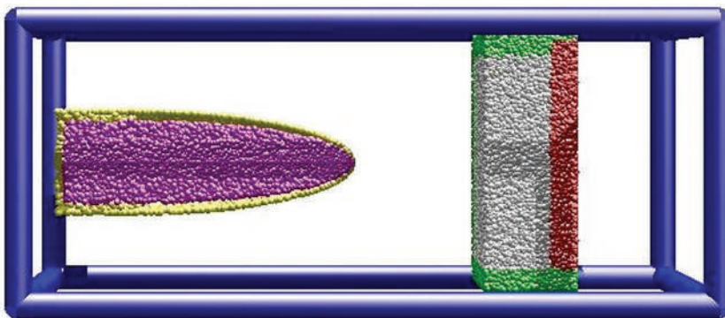
Figure 4.7 Initial configuration of the bullet/vest system (cutaway view showing bullet and vest structure). Grayscale as well as color help delineate various aspects. Purple particles show the core of the bullet, yellow is the outer copper shell, white indicates the ceramic component of the vest, red shows the spider web component, and green particles anchor the vest to the computational box (blue frame).
