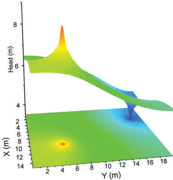
Figure 3.3 Potentiometric head surface and contour plots for a groundwater system with an injection and pumping well (Roth et al. [4]). Grayscale as well as color reveal head differences.
