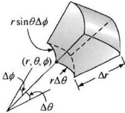
Figure 6.9 3D finite-difference volume element in spherical polar coordinates. (Adopted from https://www.taylorfrancis.com/books/mono/10.1201/b22157/heat-conduction-fifth-edition-yaman-yener-carolin-a-naveira-cotta-sad%C4%B1k-kakac .)
