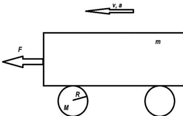
Figure 3.6 Cart with four wheels subject to a constant force and the effective (reduced) system we discuss here.
