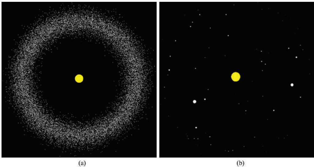
Figure 9.4 Distribution of 20,000 particles for a Barnes-Hut planetary aggregation simulation (a) initially and (b) after 98,289 time steps where 159 particles remain. The difference between the uniform radial distribution in Figure 9.1b and the Gaussian distribution in (a) here is clearly visually apparent. Note: Many particles are not visible due to their small size and the Sun’s radius has been exaggerated for graphical purposes. (Courtesy Christopher Stark [15].)
