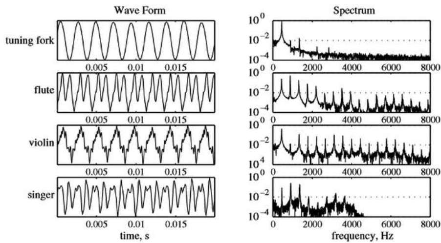
Figure 5.4 Wave forms and frequency spectra for the middle A note produced by various sound sources (adapted from Petersen [4]).
