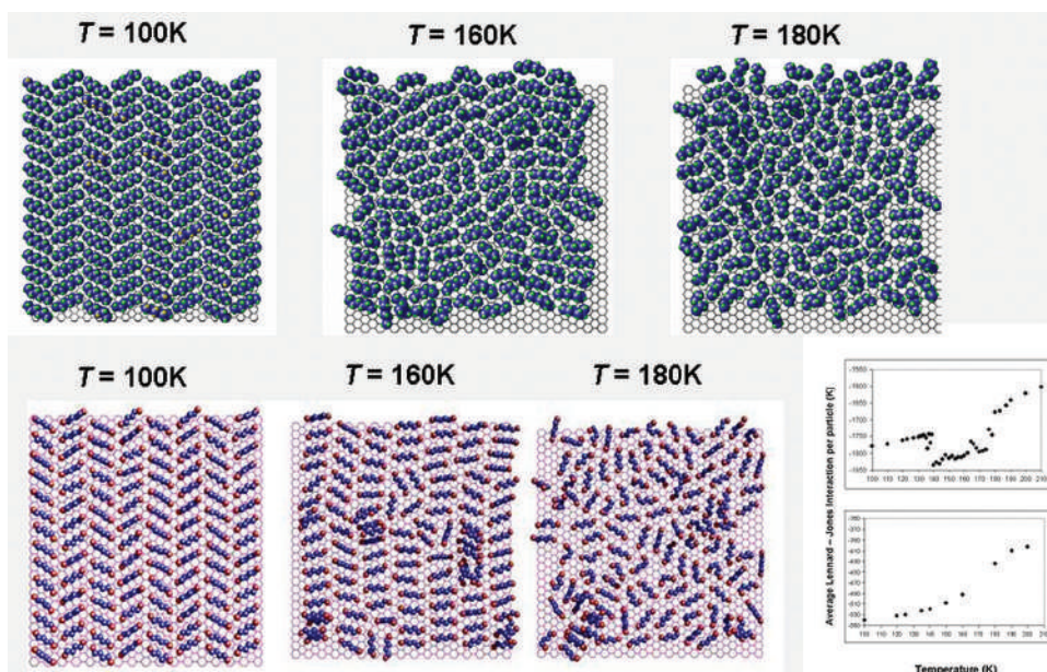
Figure 8.3 Final snapshots of hexane (C6) on graphite at various temperatures in the united atom model (bottom) and with explicit hydrogens (top). With hydrogens in place, molecular rolling agrees well with the experiment and the nematic mesophase (not seen in the experiment) is suppressed. Moreover, the artificial drop in the molecular interaction energy (top panel of lower right-hand plot) is not seen with explicit hydrogens (bottom panel of the same graph). (Connolly et al. [41].)
