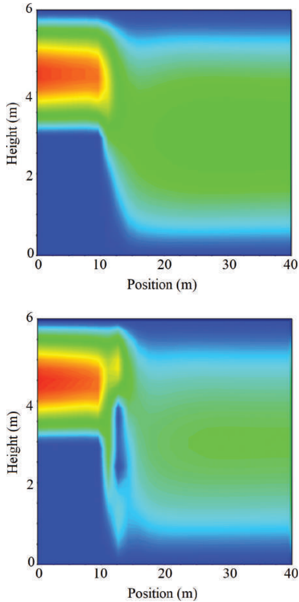
Figure 3.18 Wind speed maps for the case without any deflection fin in place (top) and with a deflection fin in place (bottom) as calculated from a finite difference solution to the Navier–Stokes equations. Grayscale and color can both delineate speed: the color scale ranges from red areas representing the highest speeds to blue regions for zero speed and uniform color mixing in between (Maldonado and Roth [15]).
