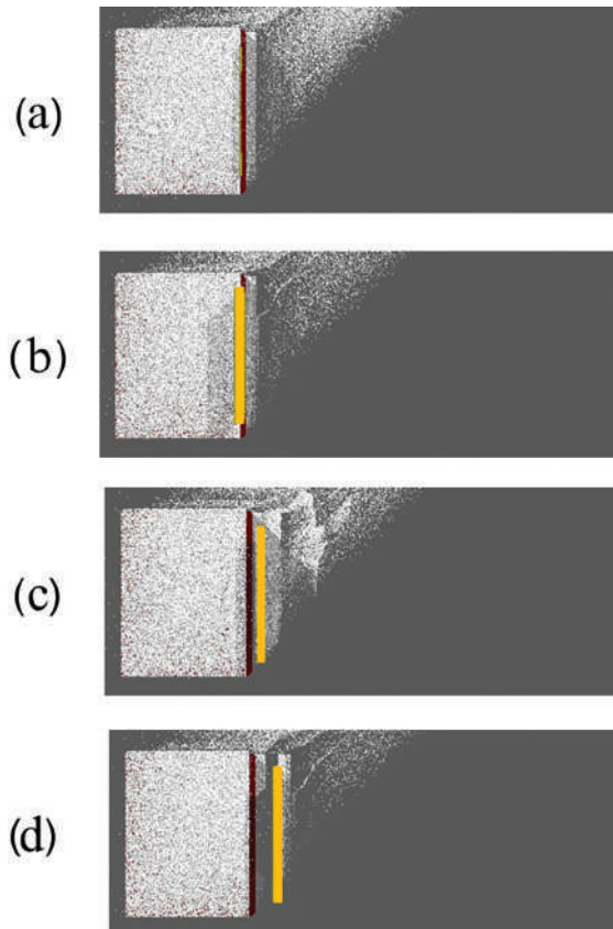
Figure A1.3 Visual renderings for final snowfall patterns resulting from side winds.
