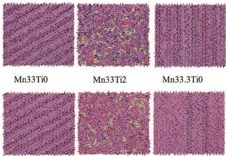
Figure 3.20 Final spatial and magnetic configuration snapshots from Monte Carlo simulations of mixed Mn/Ti layers. Grayscale as well as color can help delineate various aspects. Mn is purple, Ti is yellow, and the magnetic moments are represented by bars placed through the Mn atoms with black (N) and red (S) ends (Roth et al. [17]).
