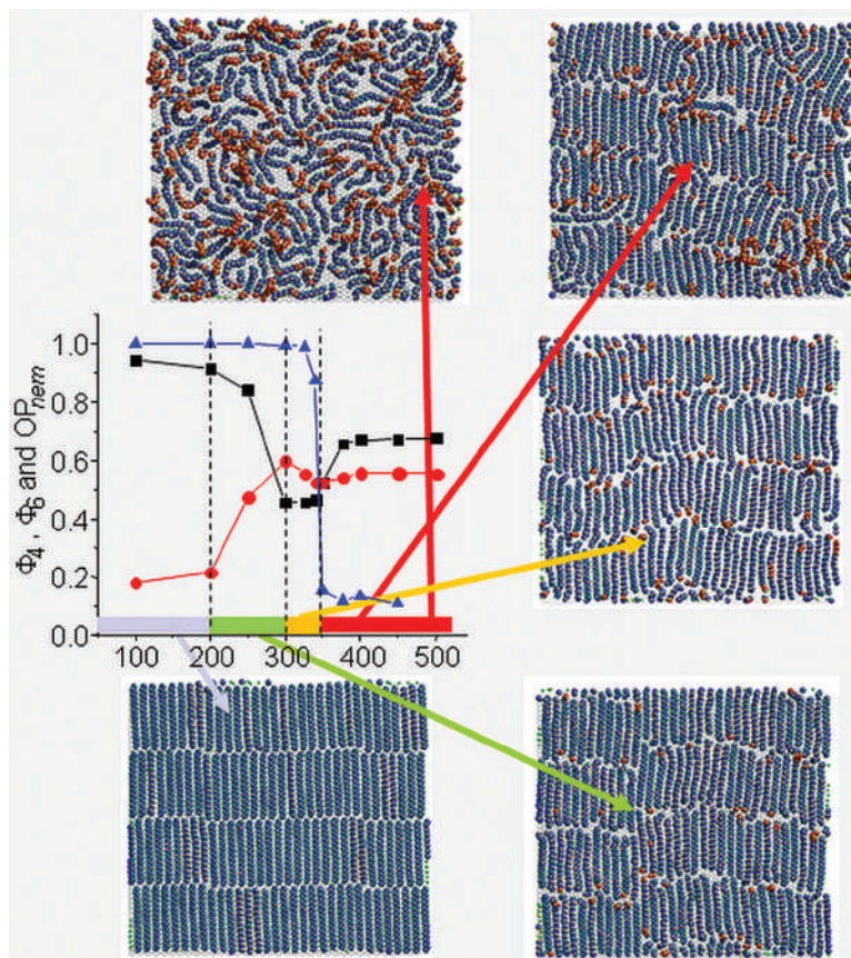
Figure 8.4 Final snapshots of all hydrogen tetracosane (C24) on graphite. Two-order parameters change slightly above T=200 K when the system enters the nematic phase, and another order parameter drops at around T=350 K, indicating melting. (Firlej et al. [42].)
