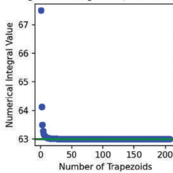
Numerical Integral Convergence (Green Line is Exact Value)
