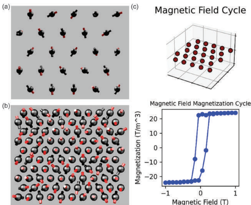
Figure 8.6 POV-generated visual for the system for (a) 5 \times 5 and (b) 10 \times 10 magnetic systems. Snapshot (c) of a native Python animation for that Ising magnetic field hysteresis cycle. In the POV-generated images, magnetic poles are represented by colored bars, and in the Python animation, they are visualized as scaled color (jet colormap). All parameters are in the program that generated the animation and can be found in the online appendix. (Screenshots by the author.)
