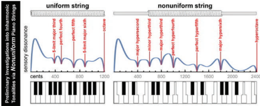
Figure 5.6 Comparison of the musical structures of the piano and hyperpiano (adapted from Hobby and Sethares [7]).
