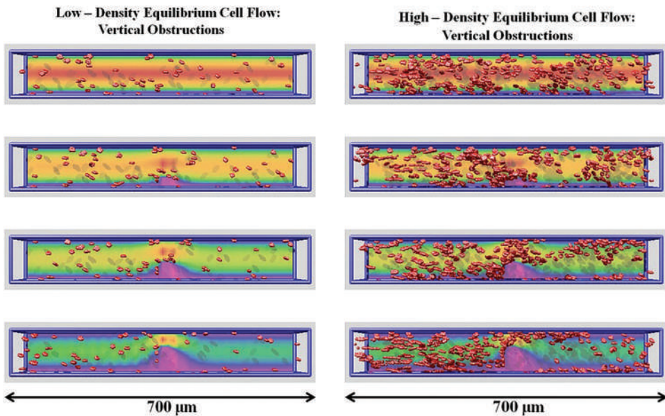
Figure 7.4 Snapshots of equilibrium erythrocyte flow for low-density (left panel) and high-density (right panel) simulations with vertical barriers. The background shows the plasma velocity field, illustrating the effects of the boundaries and barriers. Grayscale as well as color reveal the velocity profile on the back wall.
