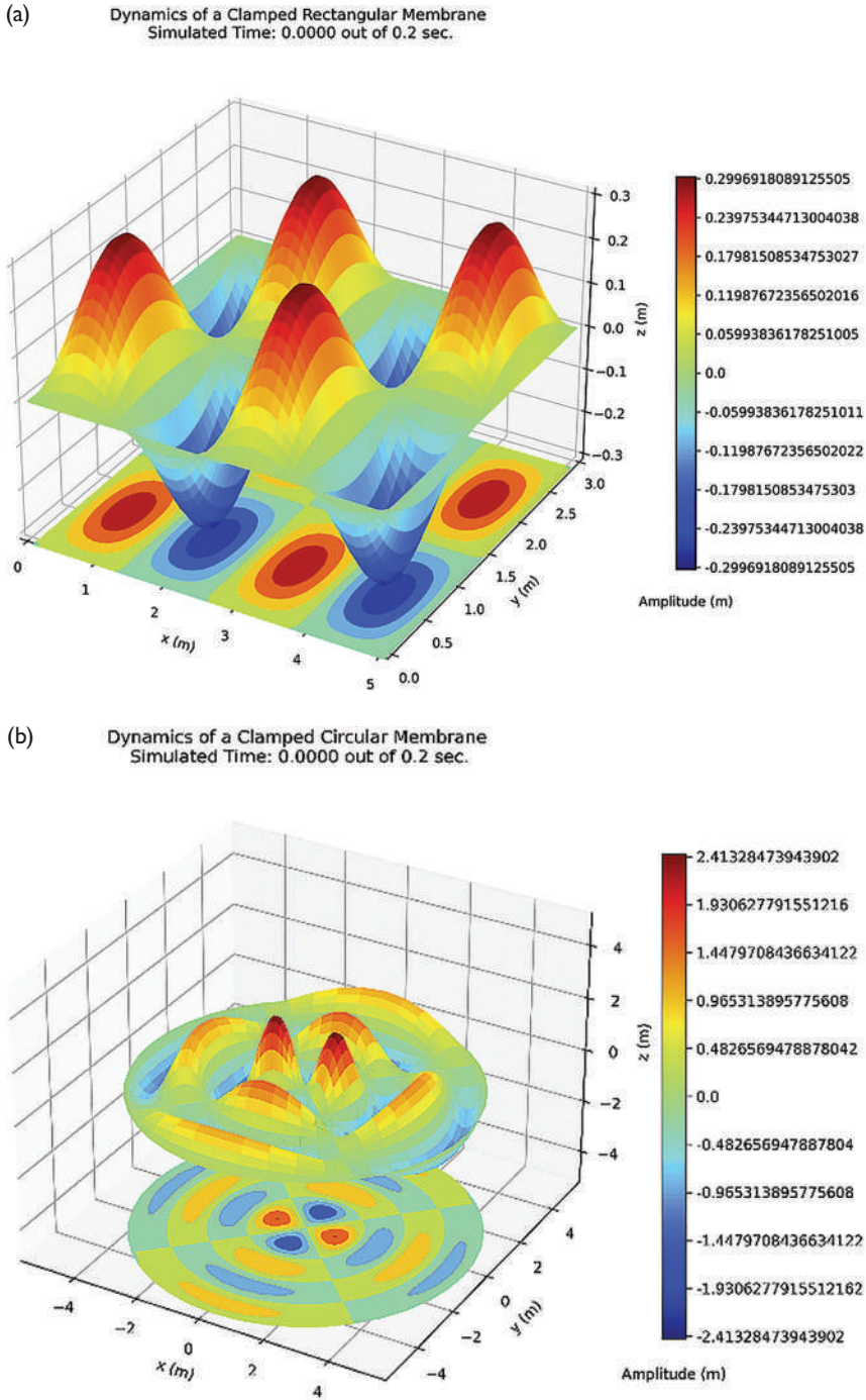
Figure 5.10 (a–d). Initial conditions for finite-difference treatments of the rectangular sheet (a) and circular membrane (b), generated by native Python graphics. Corresponding POV visuals are shown in (c) and (d). When the Fourier eigenfunction solution is included, the POV-generating codes will show both the finite-difference and Fourier eigenfunction treatments for comparison. Further results, including simulation parameters, can be found in the online appendix.
