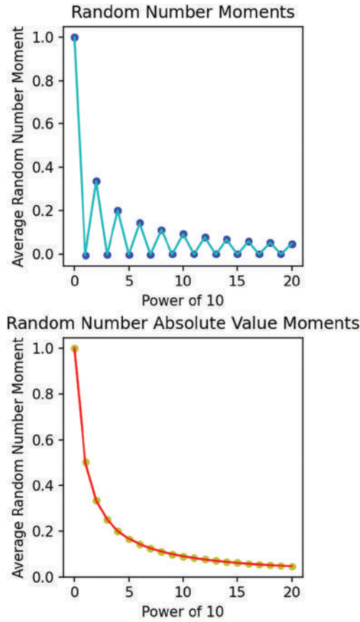
Figure 2.4 Graphical output from Math_Survey_Program_Python_Plot.py for a sample size of 10,000 and covering 21 powers of 10. (Screen capture by the author.)
