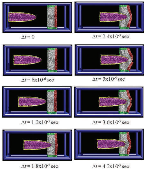
Figure 4.8 Evolution of a typical bullet impact simulation with time. Grayscale as well as color help delineate various aspects as in Figure 4.7.
