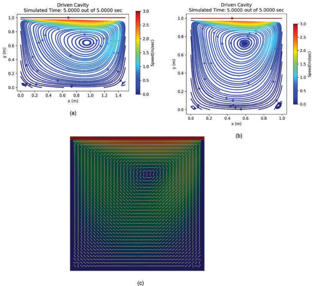
Figure 6.3 Visualizing driven fluid flow in a 1.5 \text{ m} \times 1 \text{ m} cavity with a frame taking from a native-Python-generated animation (a), a similar snapshot for a square 1 \text{ m} \times 1 \text{ m} cavity (b) and POV-rendered snapshot for the same square cavity (c). All show streamlines, with the POV rendering showing fluid speed visualized as a color gradient. Note the presence of small vortices in the lower corners as well as the large one upper right of center. Simulation parameters chosen for demonstration purposes can be found in the examples in the online appendix.
