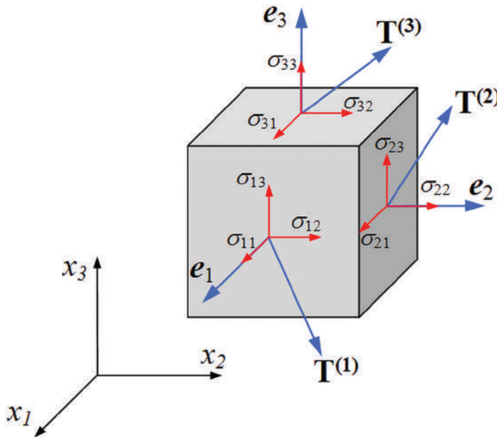
Figure 7.2 Visualization of material stress. (Adapted from Ref. [12].) The \mathbf{e}_i are unit outward normals to the cube of material, and the elements of the stress tensor \sigma_{ij} are the stresses in direction j acting on the face of the cube spanned by the tangent vectors \mathbf{T}^{(i)} normal to the unit vectors \mathbf{e}_i with coordinate x_i = \text{const.}
