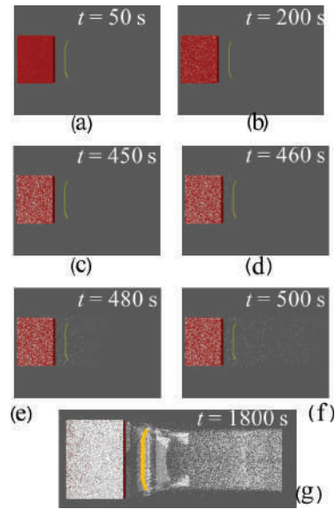
Figure A1.2 Progression of the simulated snow storm, with snow falling vertically on the roof (a–c), the wind picking up and spreading the snow (d–f) and example final configuration with the deflection fin emphasized (g).
