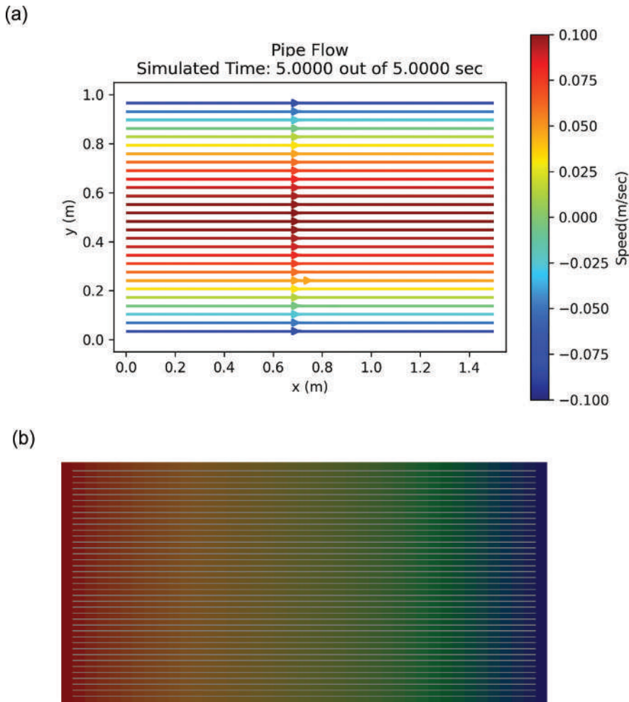
Figure 6.2 Visualizing fluid flow through a 1.5 \text{ m} \times 1 \text{ m} section of pipe with a frame taken from the native Python-generated animation (a) and POV-rendered snapshot (b). Both show streamlines, with the latter showing pressure field is visualized as a color gradient. Simulation parameters are chosen for demonstration purposes and can be found in the examples in the online appendix.
