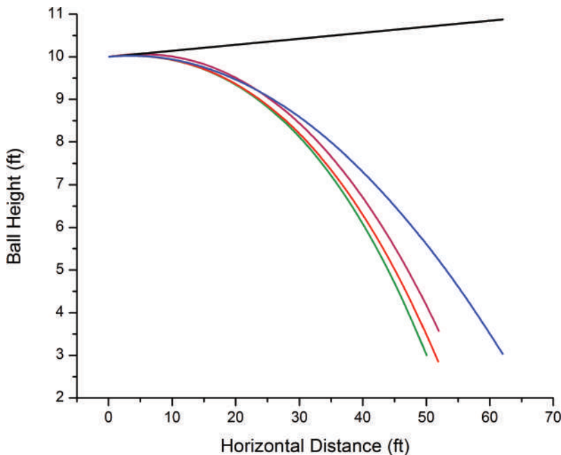
Figure 4.2 Plots of ball trajectories throughout the validation sequence for no forces (curve 1), adding gravity (curve 2), adding drag at sea level (curve 3), changing drag at sea level to drag at mountain elevations (curve 4), and adding backspin at mountain elevations (curve 5). Curves 1–5 are colored black, blue, green, red, and wine, respectively.
