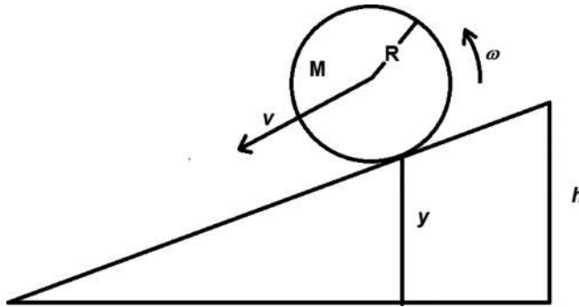
Figure 3.5 Object rolling down a ramp and the effective (reduced) system we discuss here.
