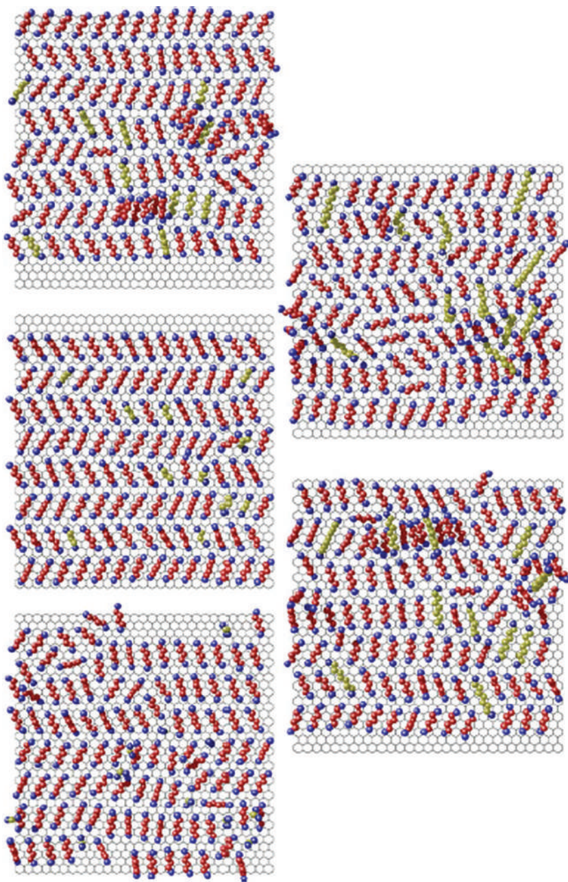
Figure 3.19 Snapshots of Molecular Dynamics studies of various alkane impurity molecules placed in a hexane on graphite system. Grayscale as well as color can help delineate impurities and host lattice atoms. (Pint and Roth [16]).
