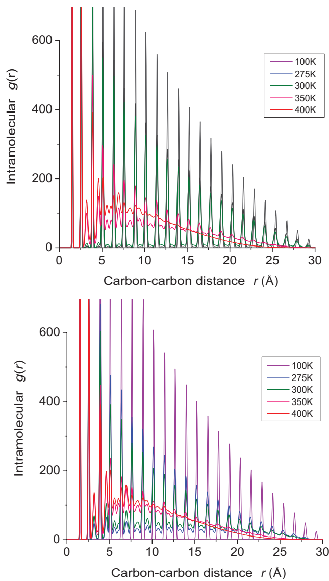
Figure 3.15 Intramolecular pair correlation functions for both layers of the tetracosane bilayer system. Grayscale as well as color help delineate behavior at different temperatures. (Roth et al. [11]).
