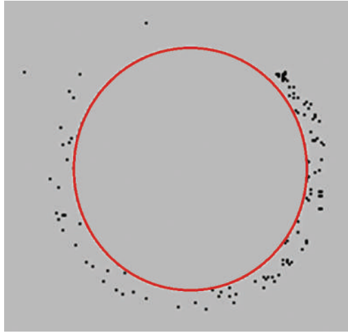
Figure 7.8 Some simulations yielded a partial ring of debris during the intermediate stage of impact. The outer boundary of the planet is shown. (Massina et al. [40].)
