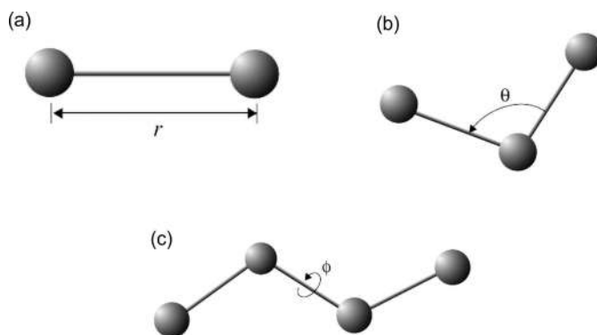
Figure 8.1 Illustration of bond length stretching (a), bond angle bending (b), and dihedral angle torsion (c) degrees of freedom.
