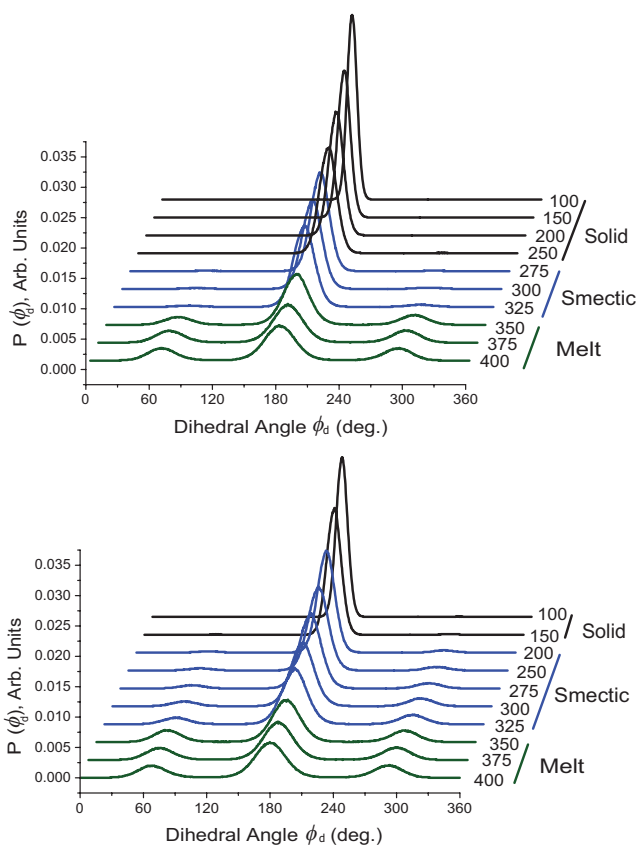
Figure 3.14 Dihedral angle distributions plotted for the upper layer (upper panel) and lower layer (lower panel) of the tetracosane on graphite bilayer for various temperatures. Grayscale as well as color help delineate different phases (Roth et al. [11]).
