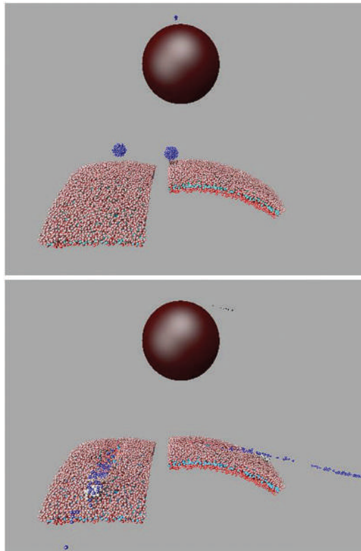
Figure 7.6 Initial configuration for a grazing impact simulation (upper) and a typical configuration shortly after impact (lower). The view of the whole planet (upper) shows particles only governed by classical Newtonian planetary dynamics, and so the impacting body disappears after impact, and the surface patch is never visible. The impacting body as well as Martian topsoil, ice layer, and subsoil (progressively deeper) are delineated by grayscale or color. (Massina et al. [40].)
