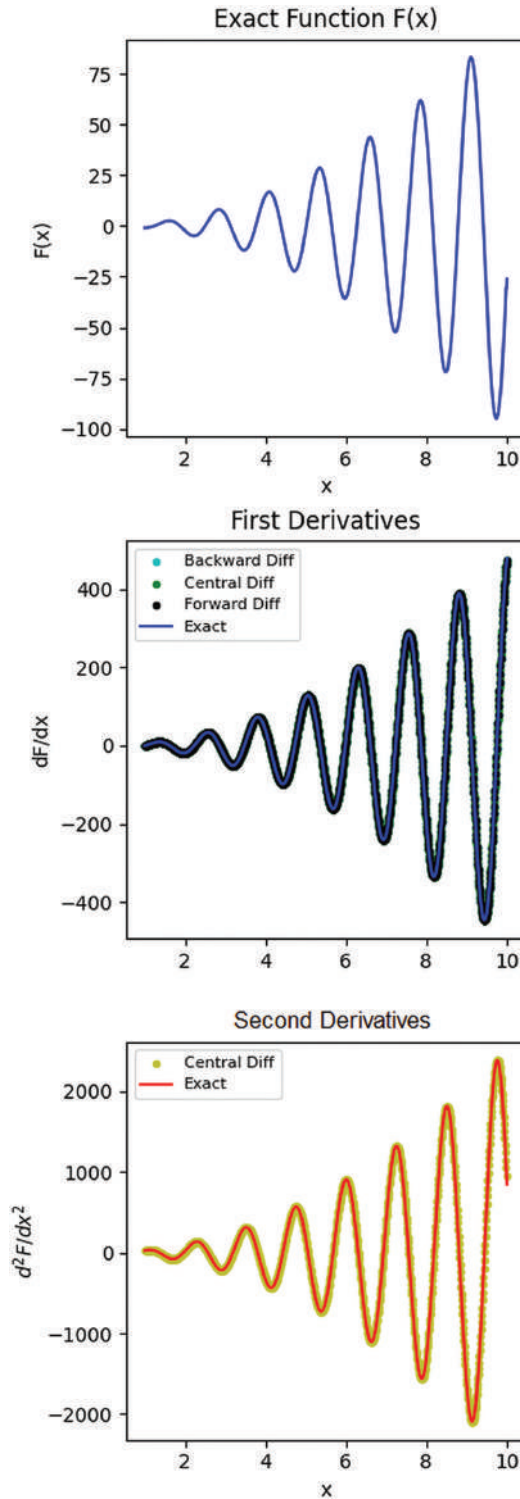
Figure 2.6 Graphical output from First_And_Second_Derivatives_Python_Plot.py for the derivatives of f(x)=x^2\sin(5x) on [1,10] using 1000 intervals.
