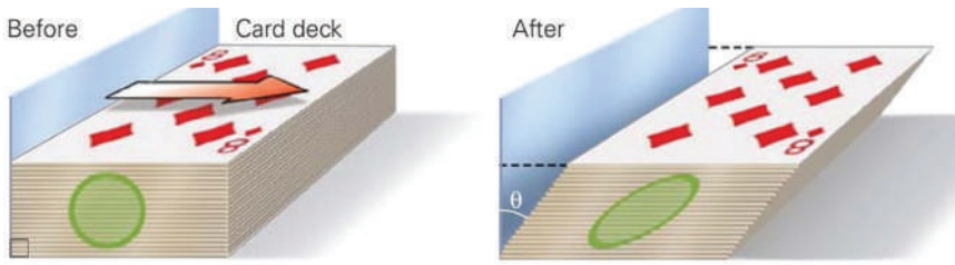
Figure 6.1 Deck of cards sliding, illustrating the effects of viscosity in fluids.
