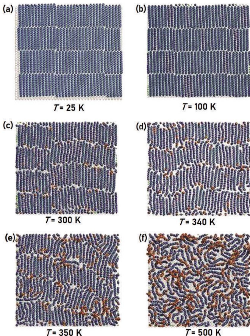
Figure 1.1 Final snapshots from a Molecular Dynamics computer simulation of a long hydrocarbon, \text{C}_{24}\text{H}_{50} (tetracosane) on graphite. The simulation gives us fairly reliable information that an experiment can't: as temperature is increased, the ends of the molecules flip up (red atoms); then the molecules remain stiff but the rows start to shift; and, at last, the system melts. Also, the effects of motion on two distinctly different timescales are visible. (Reprinted with permission from Ref. [1], Copyright 2008, American Chemical Society.)
