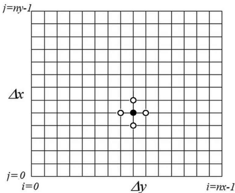
Figure 5.8 2D Cartesian IBVP and finite-difference grid used, for example in the solution of Equation 5.12.
