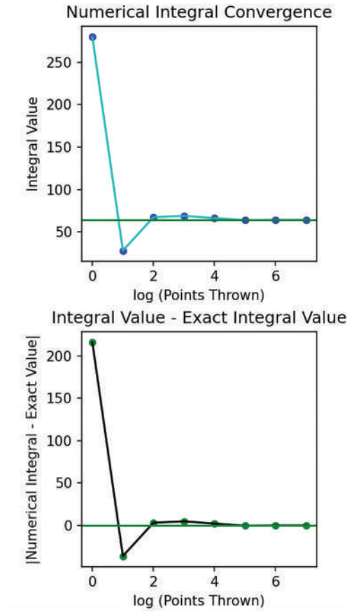
Figure 2.8 Graphical output from MC_Integration_Python_Plot.py for \int_0^4 x^3 dx using 10^n Monte Carlo steps where n=0,1,2,3,4,5,6,7 .
