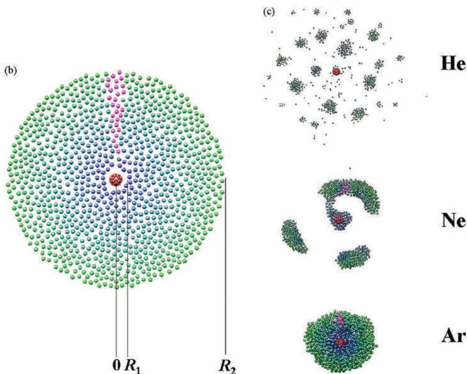
Figure 3.11 (Continued) (a) Snapshots of the top and bottom layers of Molecular Dynamics simulations of tetracosane on graphite, respectively, at various temperatures. Can you identify the solid, intermediate smectic, and liquid phase? Grayscale as well as color help delineate the following aspects. In the upper two panels, atoms colored red signify that they are significantly higher off the surface relative to their respective layer, and in the bottom panel, upper (green) and lower (blue) layers together (Roth et al. [10]). (b) Initial conditions for the nanoscale Molecular Dynamics rotating disk simulations. Grayscale as well as color help delineate the following aspects. The blue to green gradient color scale represents closest to farthest initial noble gas atom distance from the central fullerene. The purple line of atoms is used to help understand the system's rotational dynamics. (c) Snapshots of final configurations in our orbiting noble gas simulations at low temperature for He (top), Ne (middle), and Ar (bottom) (Maldonado and Roth [12]).
