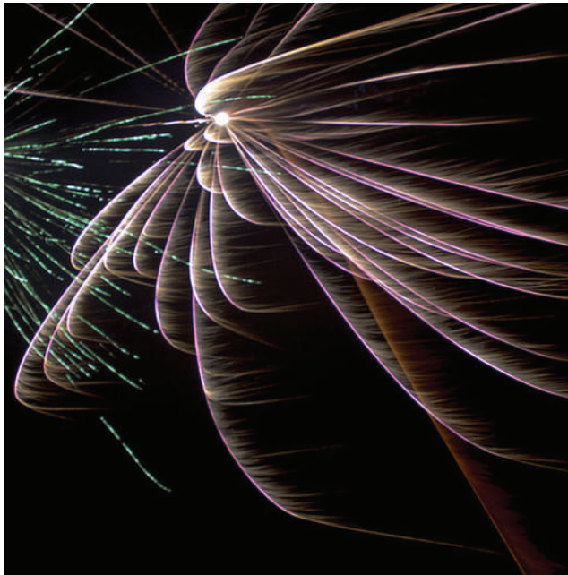
Figure 3.1 Centering, spread, and trend in a data set are exhibited by fireworks, and each aspect of the data set has a physical origin in this case (Bigstock 85787186 https:// www.bigstockphoto.com/licensing-tos.html ).
