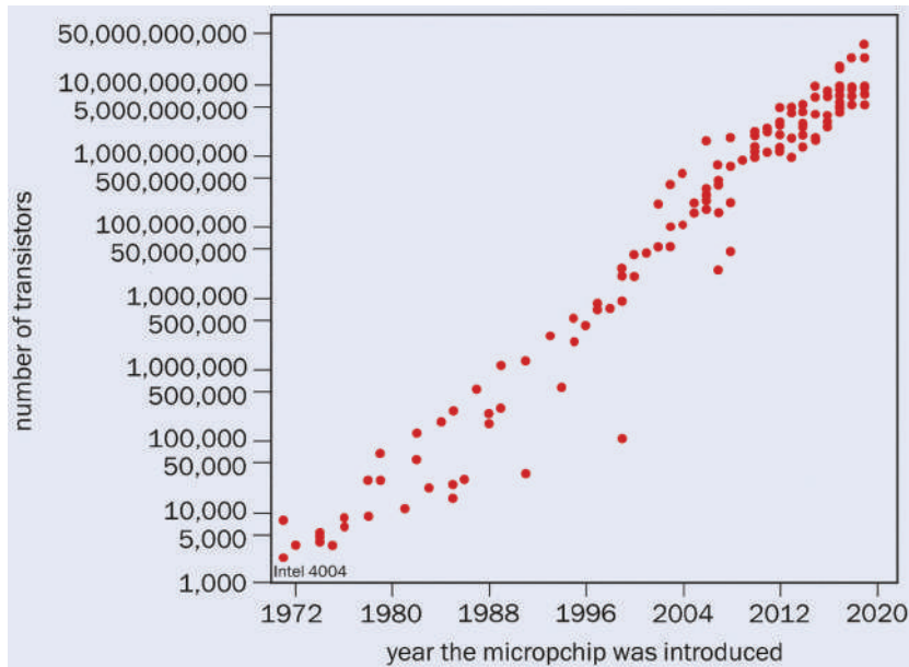
Figure 1.7 Moore's law, graphed on a semilogarithmic axis. The linear correlation indicates exponential behavior [13]. (Courtesy IOP Publishing.)
