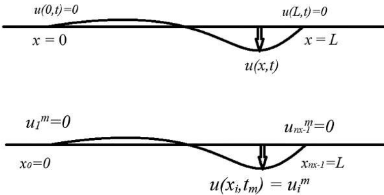
Figure 5.1 Illustration of the uniform string boundary value problem (top) and the discretized problem (bottom). Here the superscript m is the time index.
