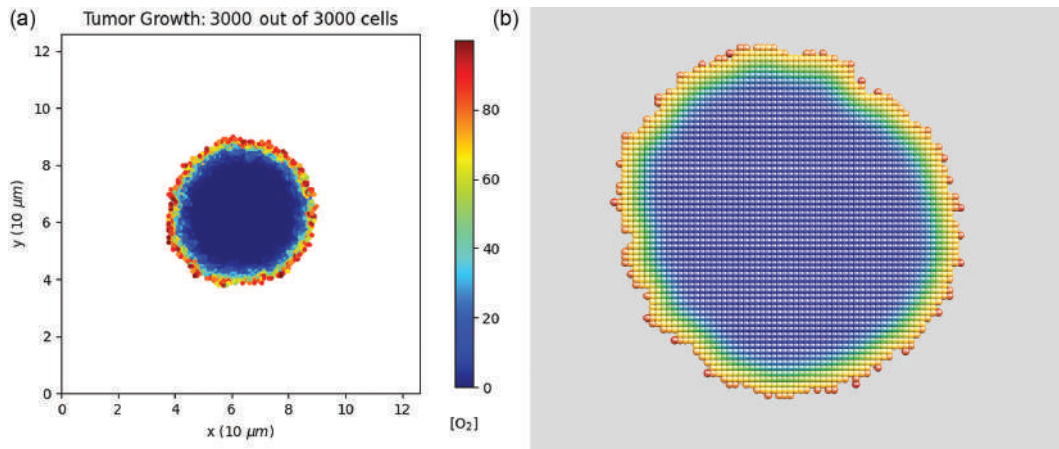
Figure 4.9 Visual representation of a tumor after 3000 growth steps generated by (a) the program shown above and (b) rendering a *.pov file generated by the C++ code or, equivalently, any of its translations. Grayscale as well as color help delineate oxygen concentrations. Distance scales are order-of-magnitude.
