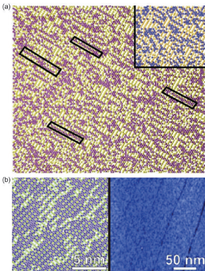
Figure 8.7 Results (a) of equilibrated Monte Carlo simulations of intercalated \text{TiS}_2 for a 200 \times 200 system showing positions of intercalated Ti ions (lighter shading) and Mn ions (darker shading) in one layer for an Mn concentration of 9% and a Ti concentration of 10%. The layer shown is the middle layer in a three-layer system. The inset shows the results for a 72 \times 72 system. In the electronic color version, gold circles represent Ti ions and purple/blue circles denote Mn ions. Examples of linear structures formed by the Mn ions are surrounded by rectangles [33]. (b) Comparison of simulated results to experimental, prompting the smiley face e-mail (Stollenwerk et al., [34].)
