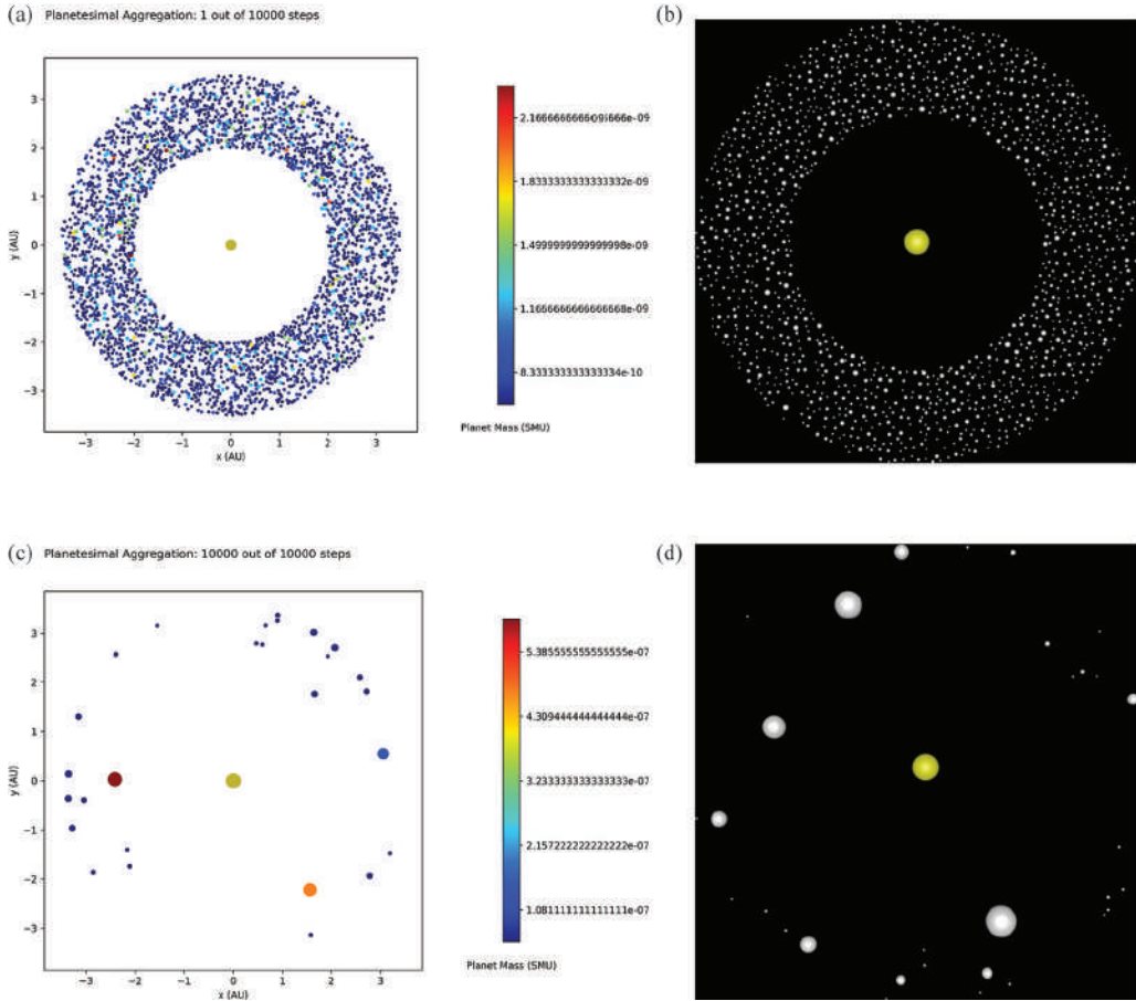
Figure 9.1 Visualization of an initial condition for the N=4,000 planetesimal simulation generated by (a) native Python graphics in the program above and (b) POV renderings from files generated by C++/Python/FORTRAN programs in the online appendix. Visualizations in the same formats but after considerable aggregation are shown in (c) and (d). The visual radii of the Sun and planetesimals have been scaled with visual aesthetics in mind. All relevant parameters can be found in the Python code. (Screenshots by the author.)
