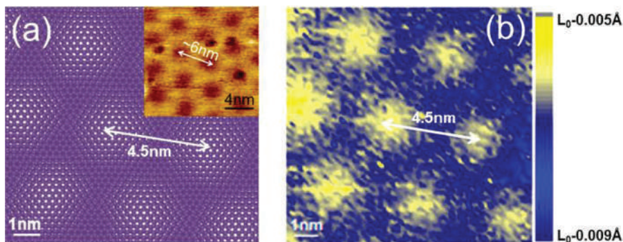
Figure 8.5 (a) Simulated Moire patterns of graphene on Cu single crystal (111). The periodicity is labeled. The inset shows an STM image of the Moire pattern in graphene on Cu (111). (b) Simulated nearest C–C bond length of graphene on Cu (111) surface. For the vertical scale bar, L_0 is the equilibrium bond length of graphene without any substrate. (He et al., [25].)
