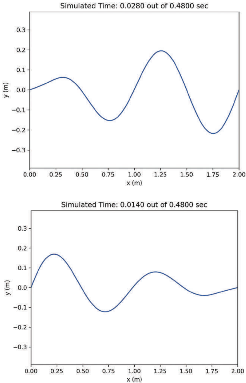
Figure 5.7 (Continued) (a–c). Snapshots of initial configuration (a) and configurations at selected times for systems varying density (b) and varying tension, (c) generated by native Python graphics. The times for (b) and (c) are chosen so that it is easy to see the effects of varying physical properties (density or tension) increasing to the right. Increasing density reduces frequency, which has the opposite effect of increasing tension. Further results, including simulation parameters and density/tension expressions, can be found in the online appendix.
