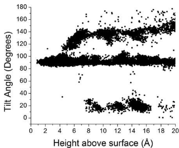
Figure 3.13 An account of how pentacene clusters with increasing height off the graphene surface at room temperature Molecular Dynamics simulations (He et al. [13]).
