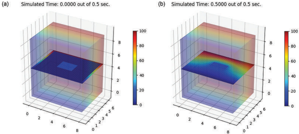
Figure 11.1 Initial(a) and end-run(b) snapshots of the Cartesian Dirichlet heat transfer problem using MPI with spatial decomposition. Parameters can be found in the demo program in the online appendix. (Screenshots by the author.)
