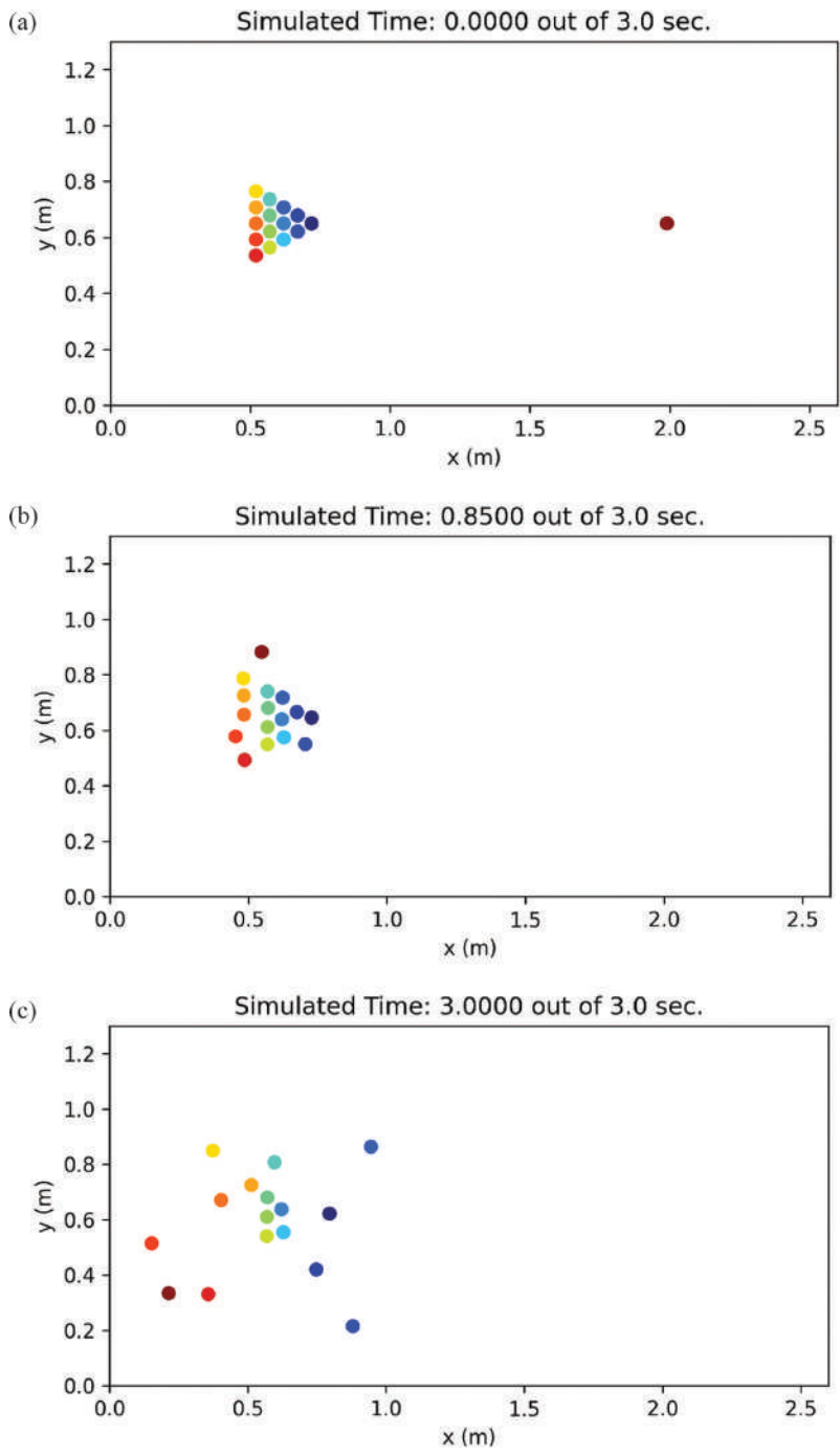
Figure 4.5 (a–c). Plots of pool ball positions for a break (a) initially, (b) near contact, and (c) at the end of the simulation. Parameters used in the simulation can be found in the example programs in the same folder as the animations and sample numerical results (online appendix). (Screenshots from native Python animations by the author.)
