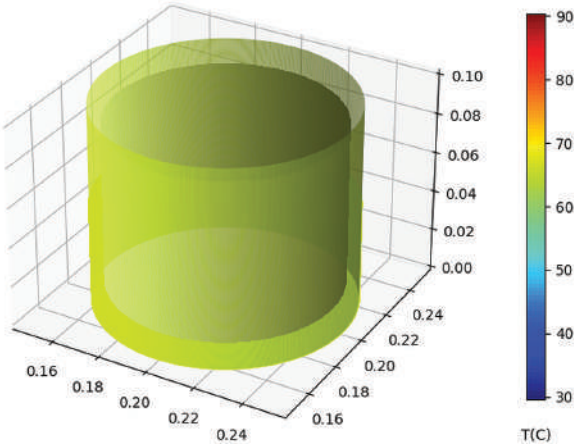
Figure 3.9 Coffee cup cooling at time t=160\text{ s} using the demo parameters suggested in the user interface ( T_i=90\text{ C} , T_s=20\text{ C} , T_{\text{quit}}=30\text{ C} and r=0.002/\text{s} ) visualized by (a) POV Raytracer and (b) native Python surface rendering. Related programs along with Bink video animations of the POV sequence and animated *.mp4 files generated from native Python applications can be found in the online appendix. (Screenshots by the author.)
