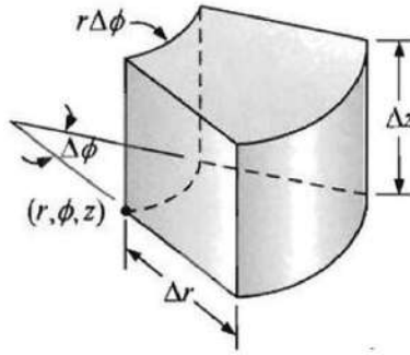
Figure 6.7 3D finite-difference volume element in circular cylindrical coordinates. (Adopted from https://www.taylorfrancis.com/books/mono/10.1201/b22157/heat-conduction-fifth-edition-yaman-yener-carolina-naveira-cotta-sad%C4%B1k-kakac .)
