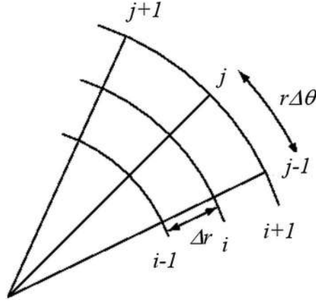
Figure 5.11 Details of the 2D plane polar IBVP and finite-difference scheme, as used in the numerical solution of the spherical drumhead problem.
