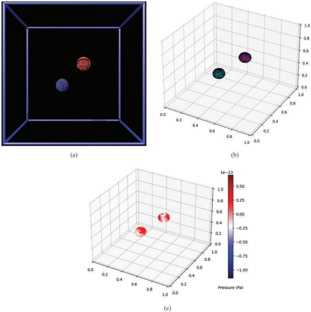
Figure 7.3 Snapshots from MPM elastic sphere collision simulation initial conditions (a) using POV visualization and colored by composition (ElementNum), (b) native Python graphics colored by composition, and (c) native Python graphics colored by pressure. Full details and extensive example results can be found in the online appendix. (Screenshots by the author.)
