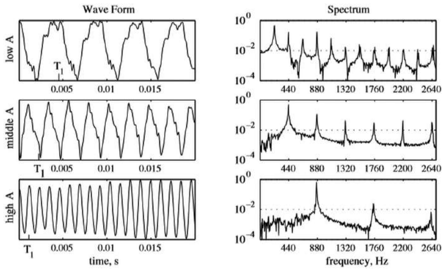
Figure 5.3 Wave forms and frequency spectra for three octaves of the A note on a piano (adapted from Petersen [4]).
