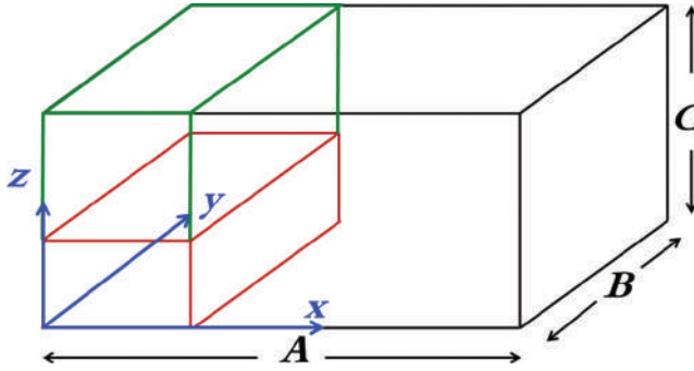
Figure A1.1 The computational cell of dimensions (A,B,C) used in the 3D snow simulations. The Cartesian coordinate system is blue, the building outline is red, and the region where snow is created is outlined in green. Not drawn to scale.
