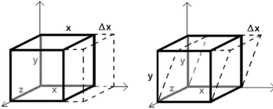
Figure 7.1 Different types of material deformation. Normal compression or extension (left) results in a volume change for the material and is related to diagonal elements of the strain tensor; shear strain (right) conserves volume and relates to off-diagonal elements. (Adapted from Ref. [11].)
