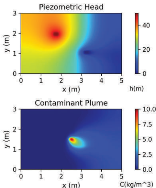
Figure 6.4 Piezometric head and contaminant concentration profile taken from an animation generated using native Python graphics. Simulation parameters chosen for demonstration purposes can be found in the examples in the online appendix.
