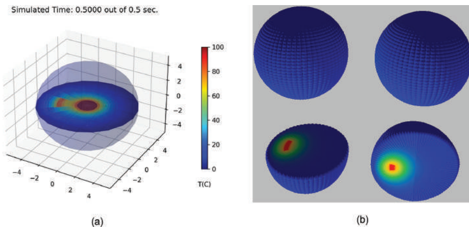
Figure 6.10 Typical results for a 3D spherical symmetry thermal conduction IBVP visualized using a frame taken from an animation generated by native Python graphics (a) and a POV-rendered representation (b). In the latter figure we show the outer boundary (upper left), active cells (upper right), and various slices (bottom). Simulation parameters can be found in the examples in the online appendix.
