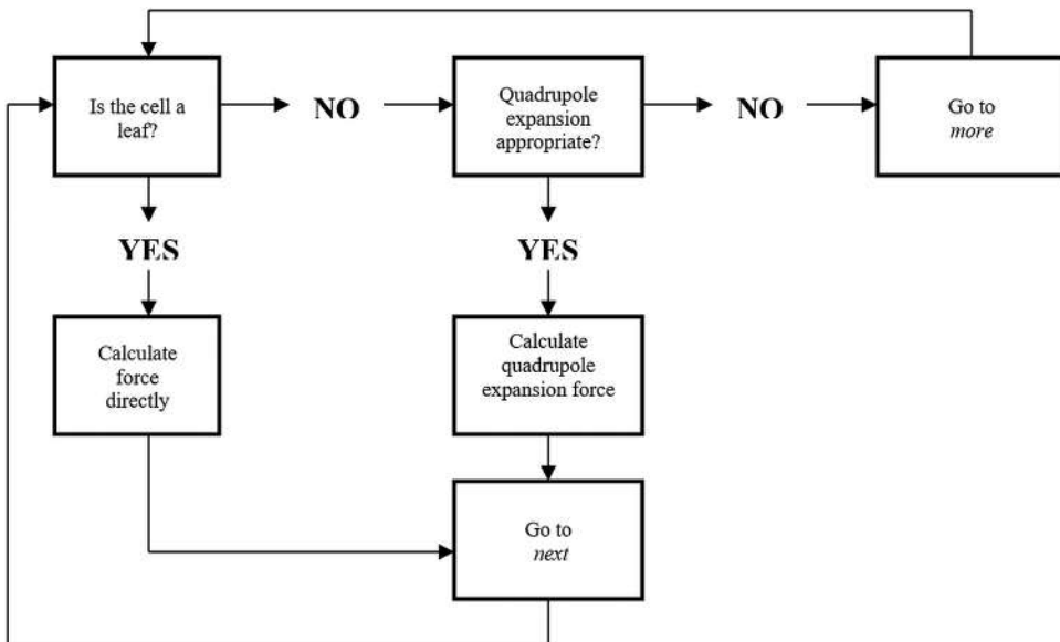
Figure 9.3 Procedure for sweeping through the tree and calculating forces [15]. (Courtesy Christopher Stark.)
