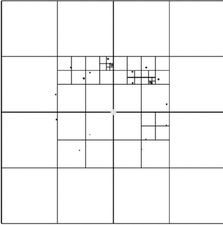
Figure 9.2 A graphical representation of the cell structure with N=20 particles. The outermost square is the root cell. Notice that each particle has its own unique cell and that only the necessary cells are subdivided. (Courtesy Christopher Stark.)
