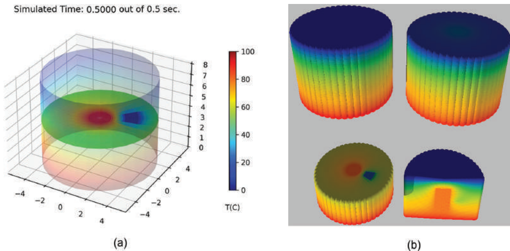
Figure 6.8 Typical results for a 3D cylindrical symmetry thermal conduction IBVP visualized using a frame taken from an animation generated by native Python graphics (a) and a POV-rendered representation (b). In the latter figure we show the outer boundary (upper left), active cells (upper right), and various slices (bottom). Simulation parameters can be found in the examples in the online appendix.
