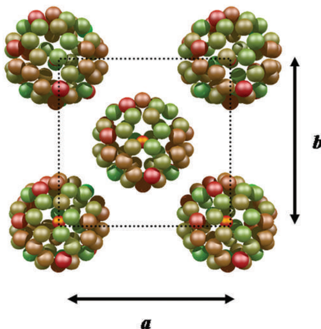
Figure 3.10 Initial conditions utilized for the Molecular Dynamics caged noble gas/fullerene simulations. The fullerene molecules are one layer of a fullerite crystal with a=b=14.4\text{\AA} . Grayscale as well as color help delineate the following aspects. The carbon atoms in each fullerene are colored green if they are closest to its center of mass, red if they are farthest away, and blend anywhere in between. The orange atoms inside the fullerene cages are encapsulated Ne atoms. (Tilton et al. [10]).
