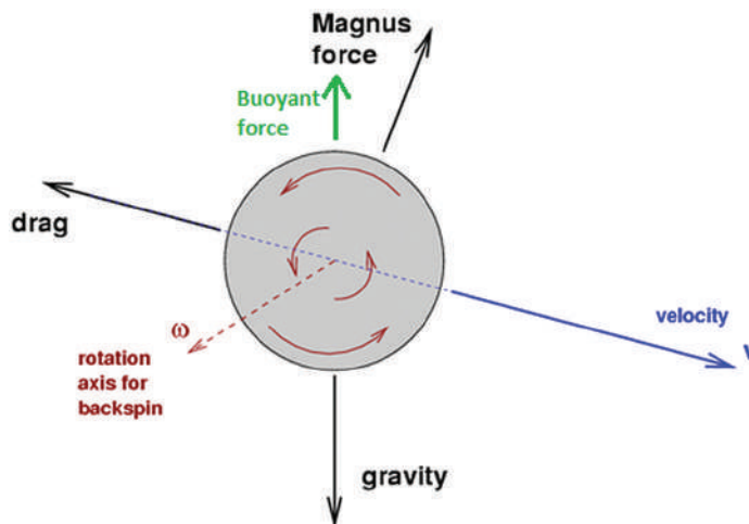
Figure 4.1 Diagram of all the forces acting on the baseball in our model. (Adapted from http://spiff.rit.edu/richmond/baseball/traj/traj.html .) The effect of air on spinning objects was noticed centuries ago and there is some very interesting reading I refer you to such as Isaac Newton [24], the work by Magnus himself, [25], and Lord Rayleigh [26].
