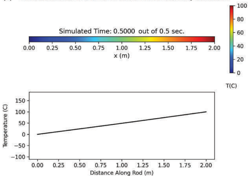
Figure 6.5 (a–b) Visualizing a conducting bar transitioning from initial conditions (a) to equilibrium (b) as visualized from frames from an animation created with native Python graphics. Simulation parameters can be found in the examples in the online appendix and POV renderings (not shown here) for the bar are similar.
