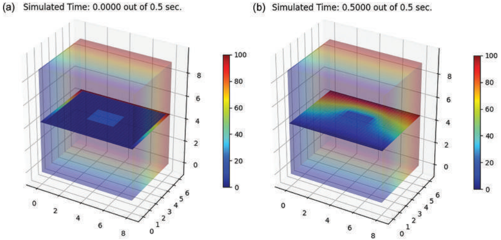
Figure 10.1 Initial (a) and end-run (b) snapshots of the Cartesian Dirichlet heat transfer problem using OOP to implement different types of spatial derivatives. Parameters can be found in the demo program in the online appendix (screenshots by the author).
