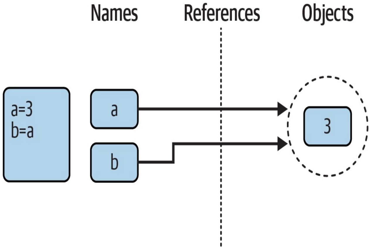
Figure 6-2. Names and objects after next running the assignment b = a
