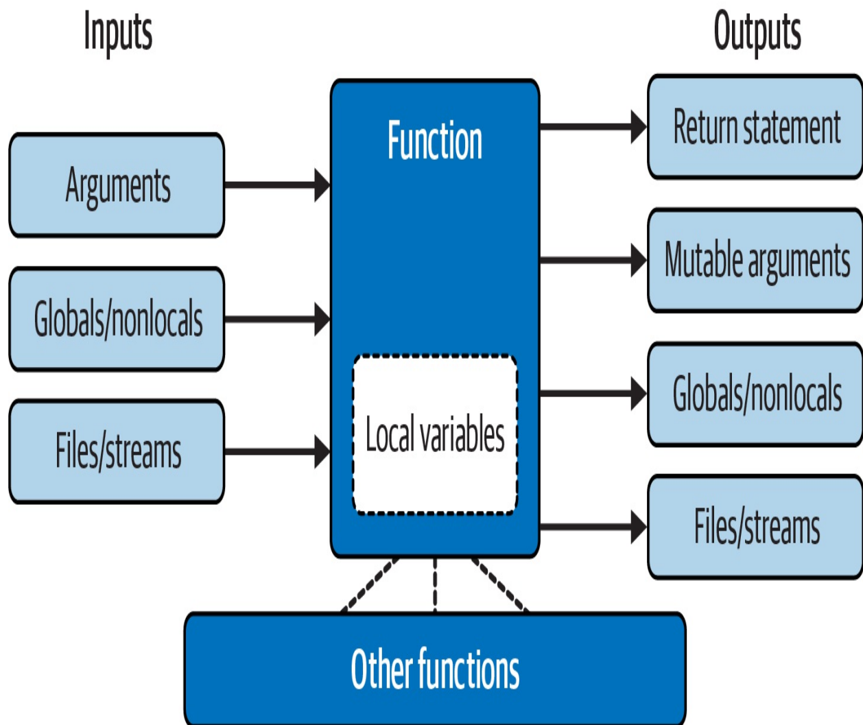
Figure 19-1. Function execution environment
