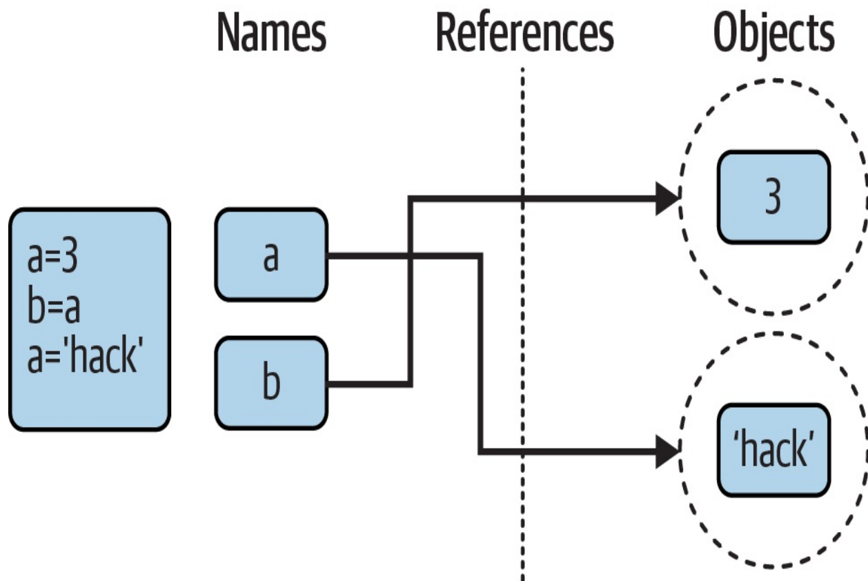
Figure 6-3. Names and objects after finally running the assignment a = 'hack'
