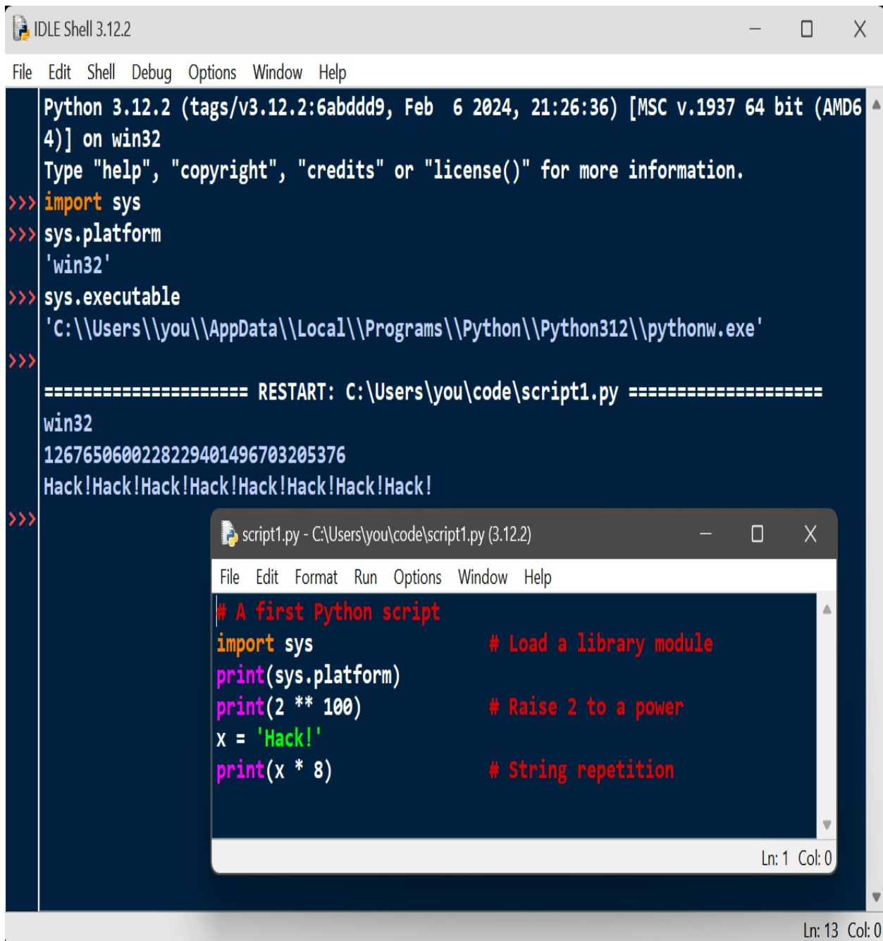
Figure 3-1. IDLE with its dark theme on Windows
