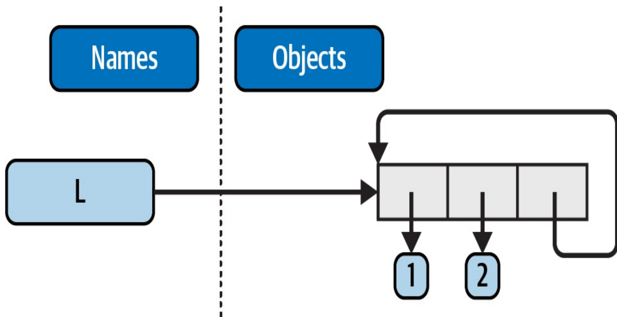
Figure B-1. A cyclic object, created by appending a list to itself
