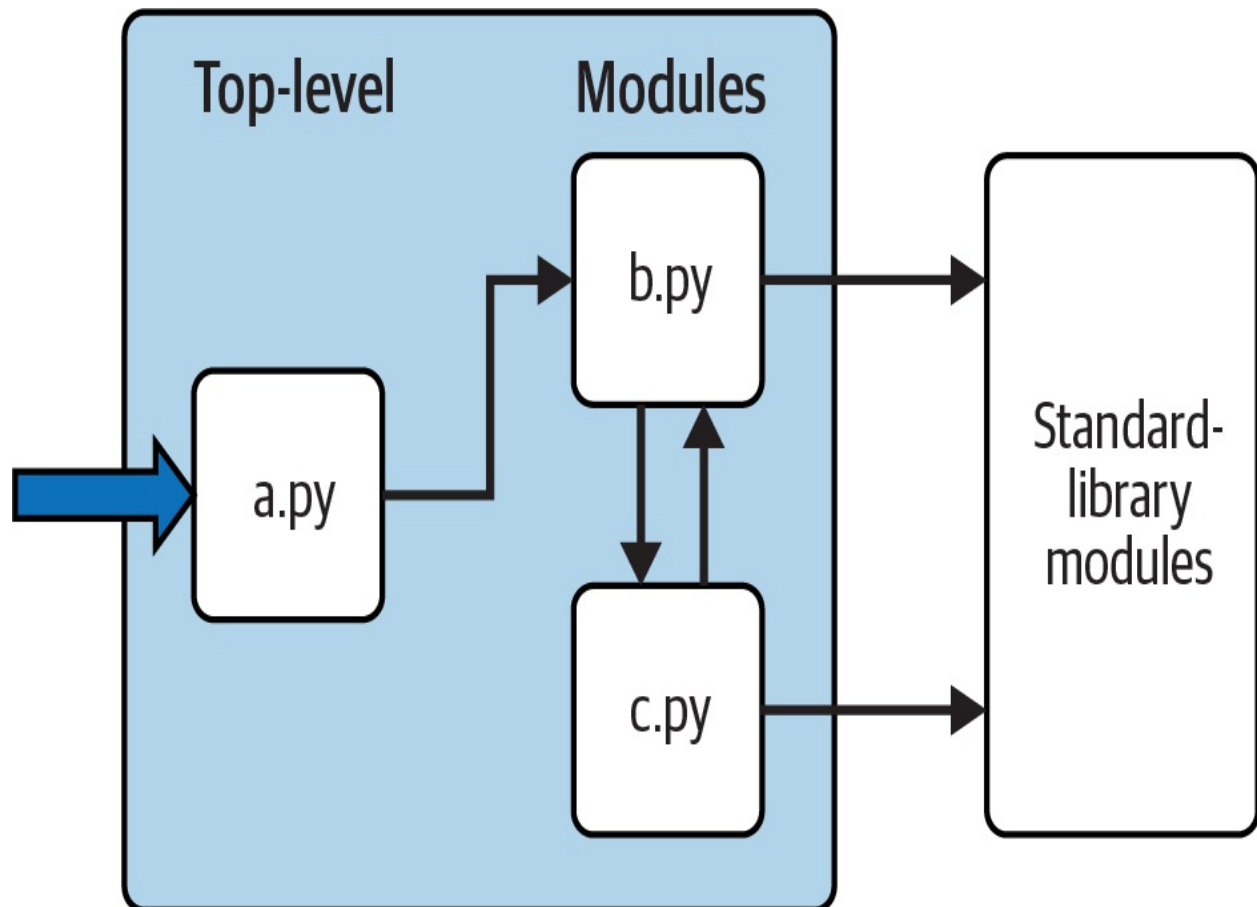
Figure 22-1. Program architecture in Python
