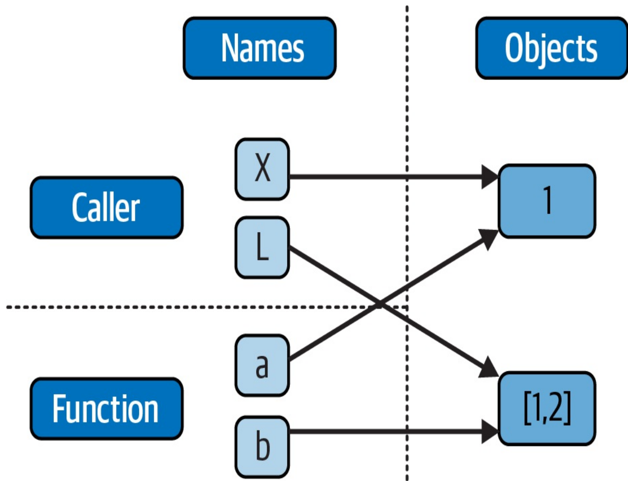
Figure 18-1. Function arguments and shared object references
