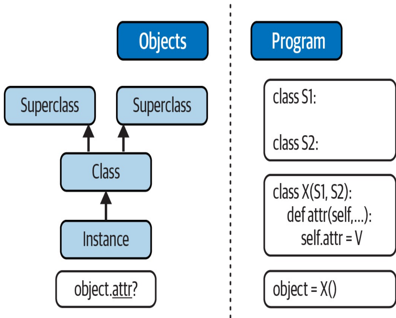
Figure 29-1. Program code creates a tree of objects searched by attribute inheritance
