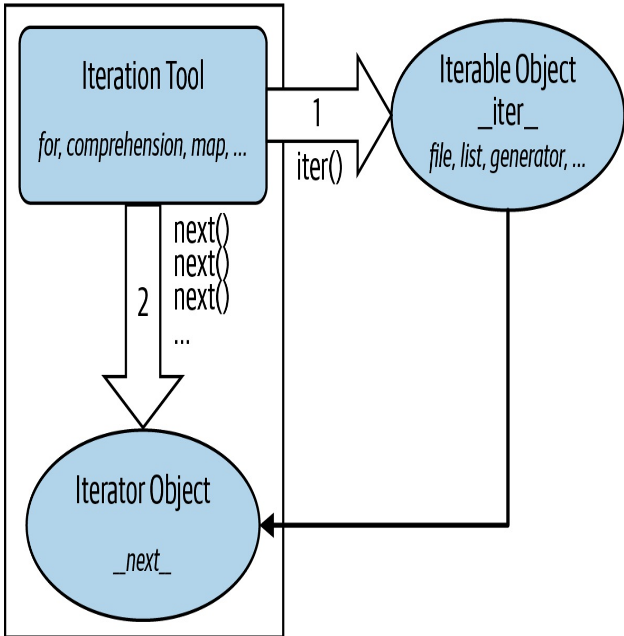
Figure 14-1. The iteration protocol, used by for loops, comprehensions, maps, and more
