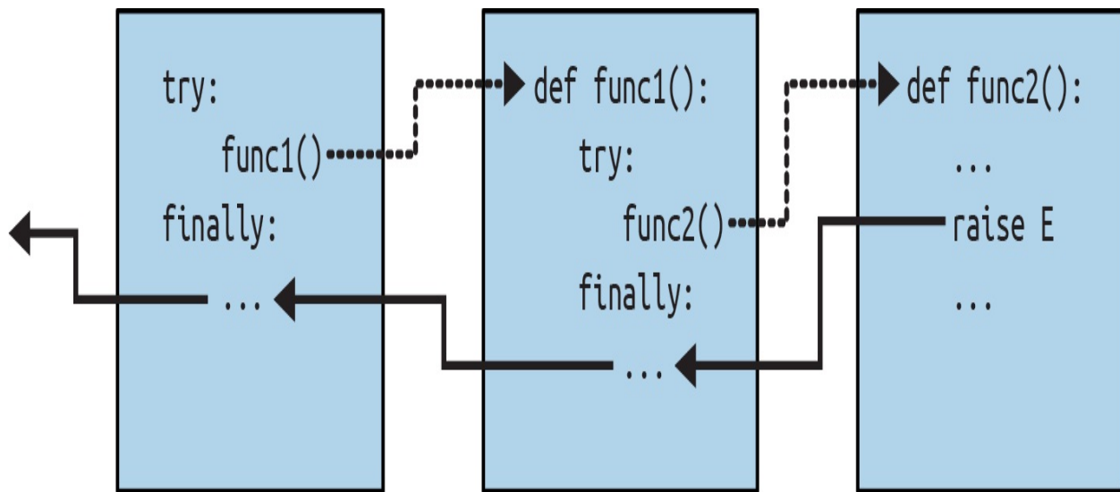
Figure 36-2. Nested try/finally combinations
