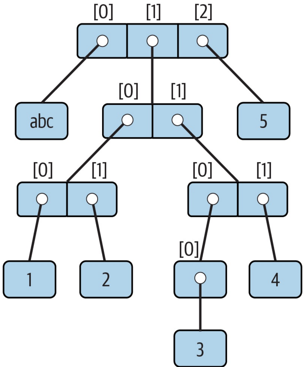
Figure 9-1. A nested object tree with the offsets of its components
