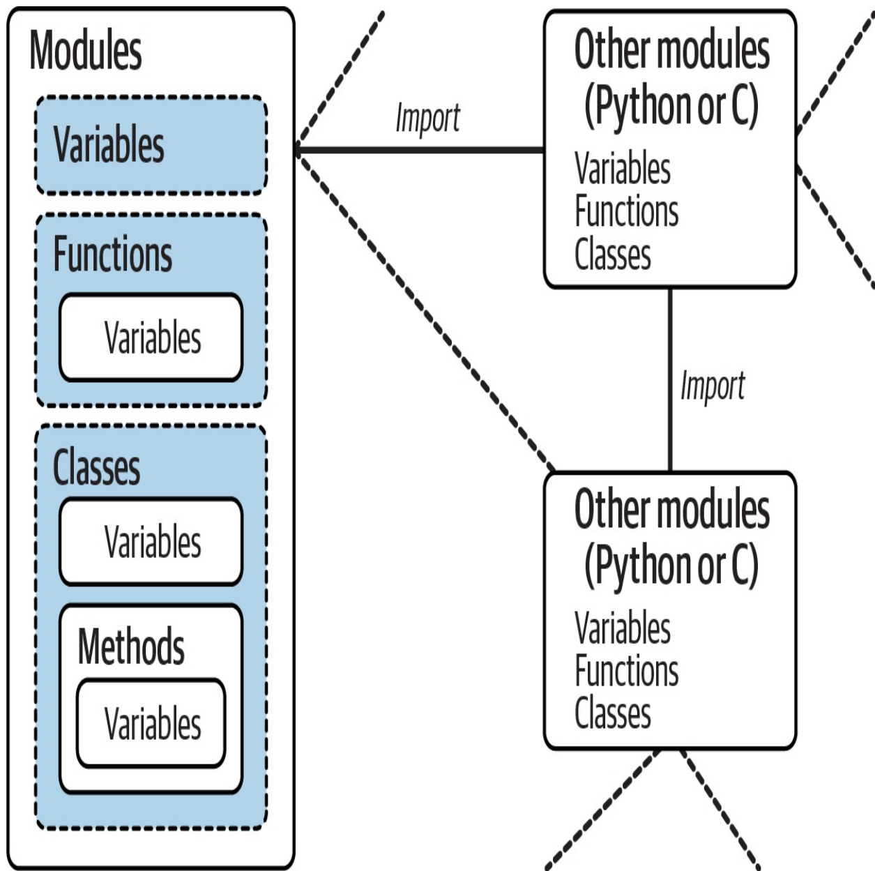
Figure 25-1. Module execution environment
