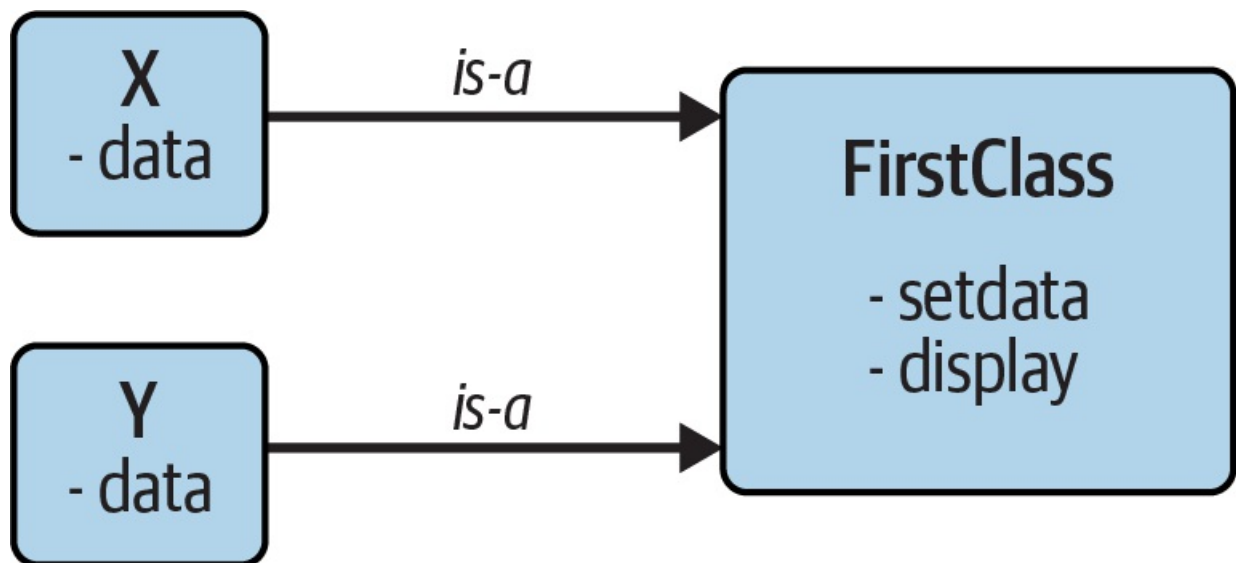
Figure 27-1. Classes and instances: namespaces in a class tree searched by inheritance
