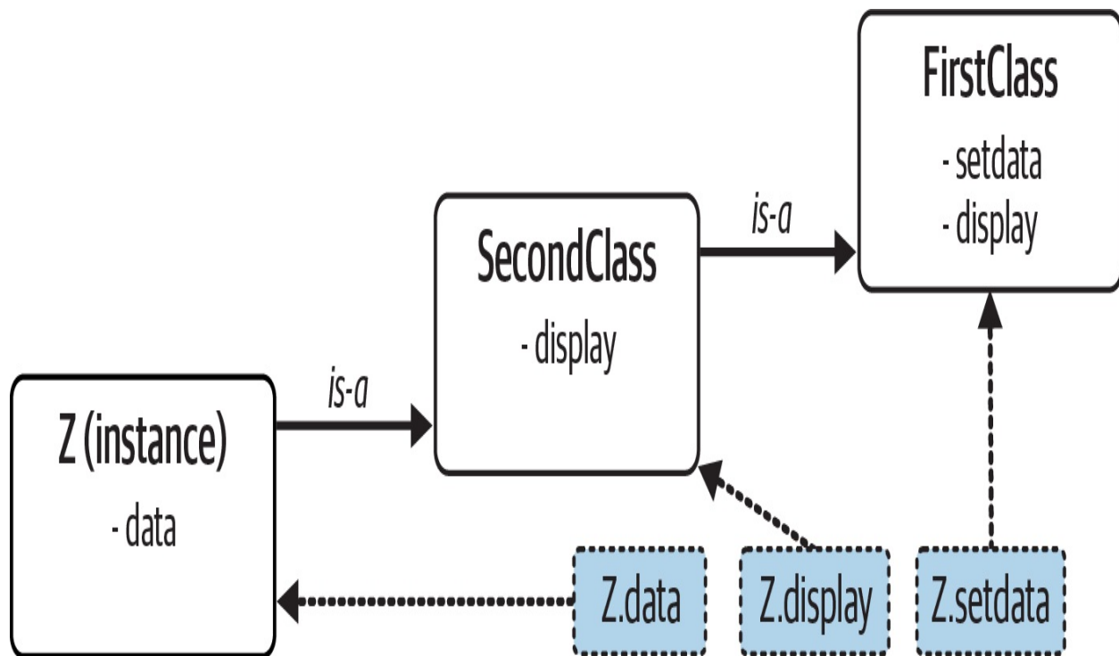
Figure 27-2. Specialization: overriding inherited names by redefining them in subclasses
