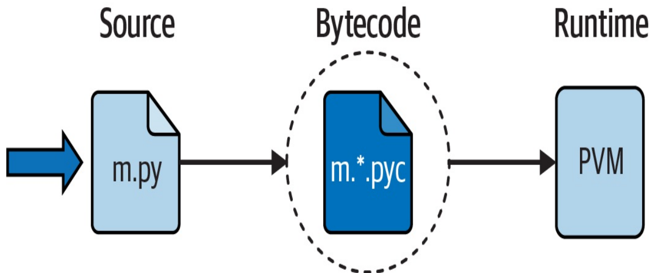
Figure 2-1. Python's traditional execution model: the PVM runs compiled bytecode
