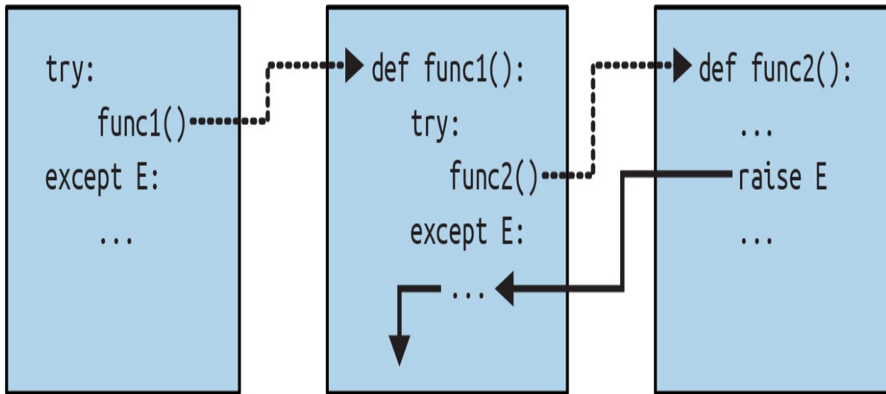
Figure 36-1. Nested try/except combinations
