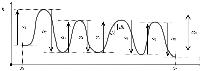
Fig. 3.23 The variation of the function h in the interval [x_1, x_2] is the sum of amplitudes \alpha_1, \alpha_2, \dots, \alpha_8 (Maio & Maltoni, 1998a). If the function is periodic or the function amplitude does not change significantly within the interval of interest, the average amplitude \alpha_m can be used to approximate the individual \alpha values. Then the variation may be expressed as 2\alpha_m multiplied by the number of periods of the function over the interval
