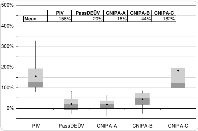
Fig. 2.24 Total accuracy drop for five different IQS specifications. PassDEÜV IQS was defined by German BSI (Federal Office for Information Security) for the German passport project and coincides with IAFIS IQS except for the area that can be smaller ( 20 \times 16 \text{ mm}^2 ). CNIPA-A/B/C specifications are being suggested by CNIPA (the Italian National Center for Information and Communication Technology in the Public Administration, now called AGID)
