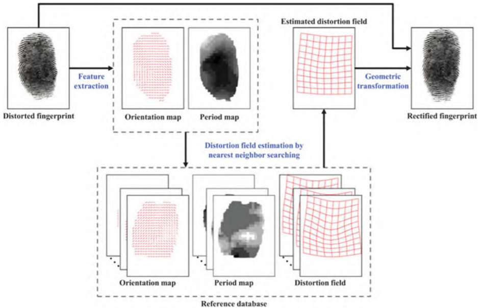
Fig. 4.23 Learning-based distortion rectification in the approach by Si et al. (2015). © IEEE. Reprinted, with permission, from Si et al. (2015)
