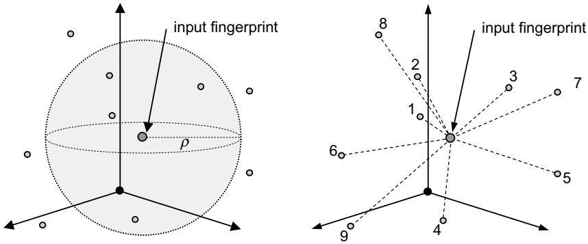
Fig. 5.13 Retrieval strategies for indexing based on global features (a.k.a. continuous classification). On the left: a hypersphere is considered with center on the query and radius determined by the penetration rate ( fixed value of PR ). On the right: the fingerprints are incrementally retrieved according to the distance of the corresponding vectors from the input point ( incremental search )
