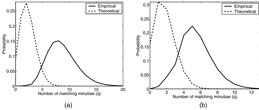
Fig. 8.6 Comparison of experimental and theoretical probabilities of random correspondence: a. MSU_DBI database, b. MSU_VERIDICOM database
