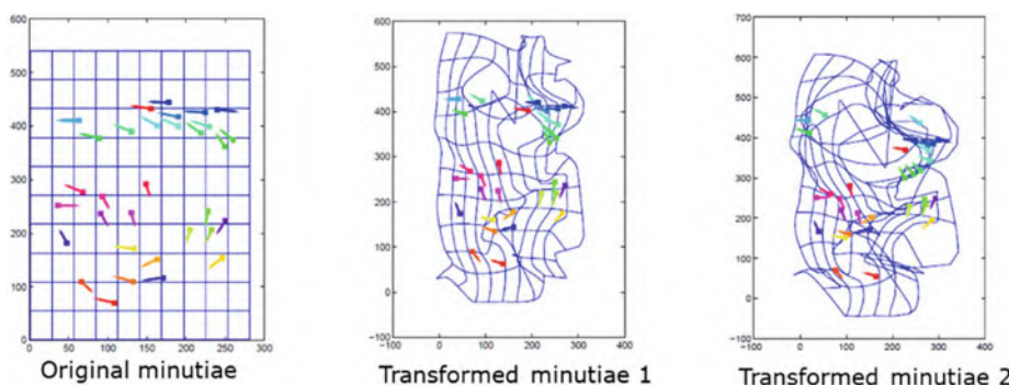
Fig. 9.24 In the feature transformation function proposed by Ratha et al. (2007), both the position and the orientation of the minutiae are changed by a surface folding function. Conceptually, the minutiae are embedded in a sheet, which is then crumpled. This function is locally smooth, but not globally smooth. As the transformation parameter is increased (as we move from the middle image to the right image), the irreversibility increases, but the matching accuracy decreases. This demonstrates the non-invertibility versus accuracy tradeoff in this approach
