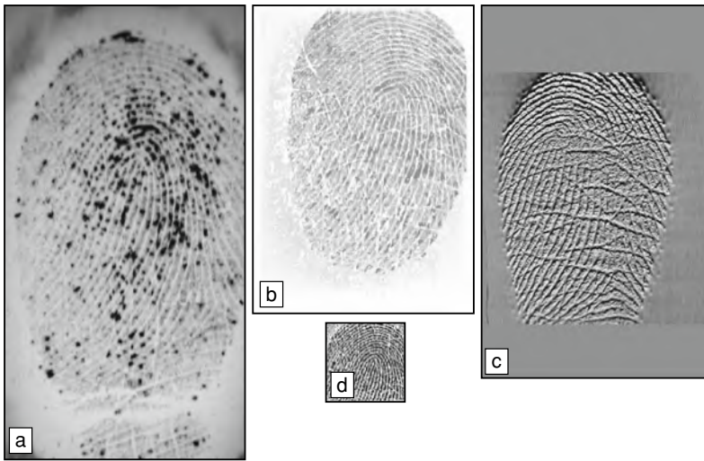
Fig. 2.28 Fingerprint images of the same poor-quality finger acquired with scanners based on four different sensing technologies: a Optical FTIR, b Capacitive, c Thermal, and d Capacitive (Active)
