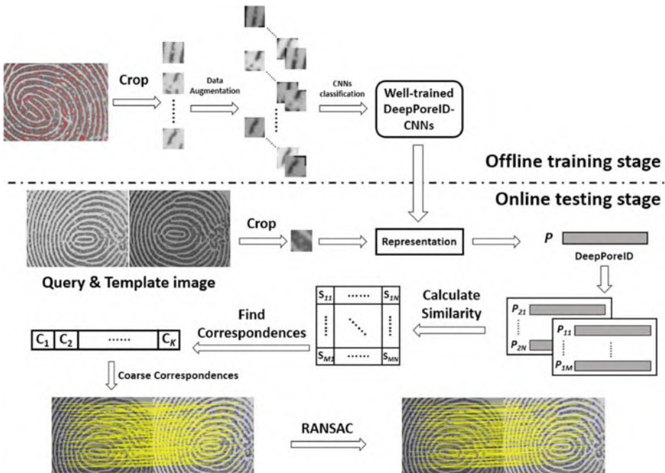
Fig. 4.26 An overview of the pore matching approach by Liu et al. (2020). © Elsevier. Reprinted, with permission, from Liu et al. (2020)
