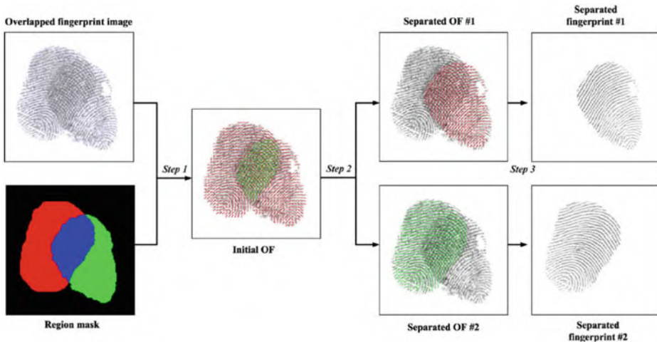
Fig. 6.22 Flowchart of separating overlapped fingerprints (Chen et al., 2011). © IEEE. Reprinted, with permission, from Chen et al. (2011)
