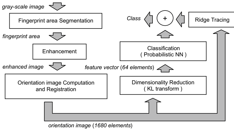
Fig. 5.7 A functional scheme of PCASYS (Candela et al., 1995). © IEEE. Reprinted, with permission, from Cappelli et al. (1999a)
