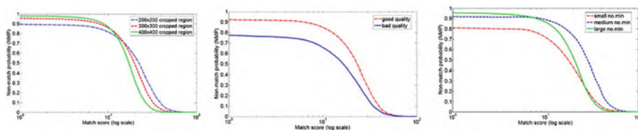
Fig. 8.8 NMP-curves for partial fingerprints of different sizes, quality levels, and numbers of minutiae (Nagar et al., 2012). © IEEE. Reprinted, with permission, from Nagar et al. (2012)
