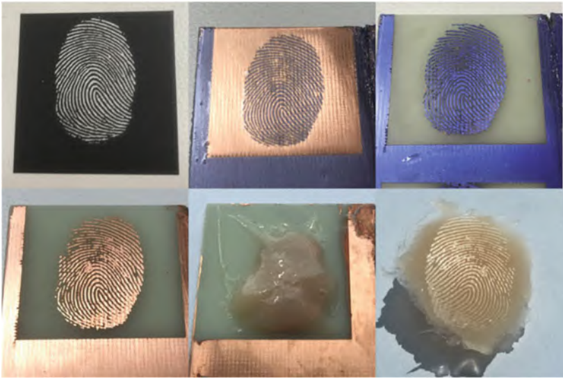
Fig. 9.9 Illustration of the non-cooperative process to create a fake replica using a residual fingerprint on printed circuit board (PCB)
