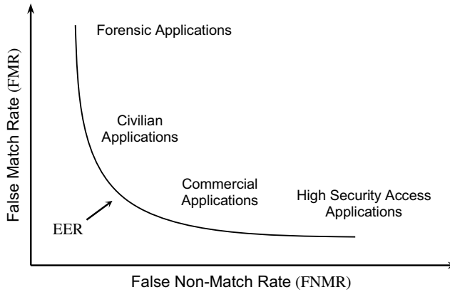
Fig. 1.6 Typical operating points of different applications displayed on an ROC curve
