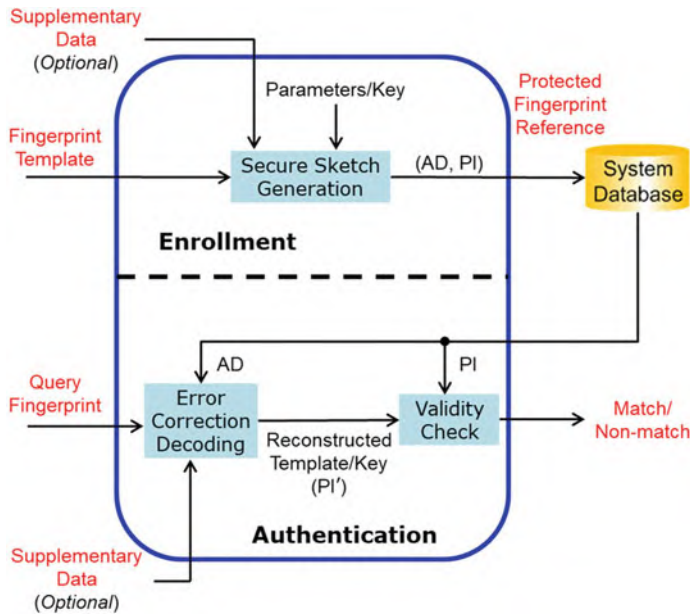
Fig. 9.21 Typical workflow of a fingerprint cryptosystem used for fingerprint template protection. © IEEE. Reprinted, with permission, from Nandakumar and Jain (2015)
