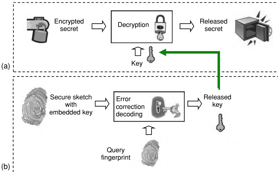
Fig. 9.22 Leveraging a fingerprint cryptosystem to alleviate the key management problem in cryptographic systems. a Typical workflow of a cryptographic system and b illustration of how a fingerprint cryptosystem can be used as a secure key release mechanism
