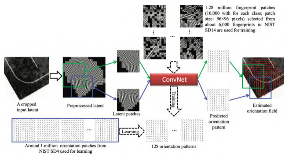
Fig. 6.21 The flowchart of ConvNet based orientation field estimation algorithm (Cao & Jain, 2015). © IEEE. Reprinted, with permission, from Cao and Jain (2015)
