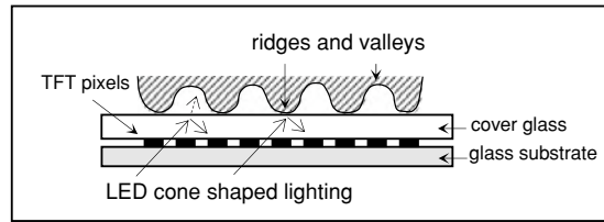
Fig. 2.9 A lensless optical sensor based on TFT technology. In the Hidden Optical Touch configuration proposed by Bae et al. (2018), the LED light source is placed under the TFT glass substrate and is partially masked by the pixel array. A cone shape light with a proper incidence angle reaches the cover glass surface and is reflected back to the photodetectors without crosstalk between pixels
