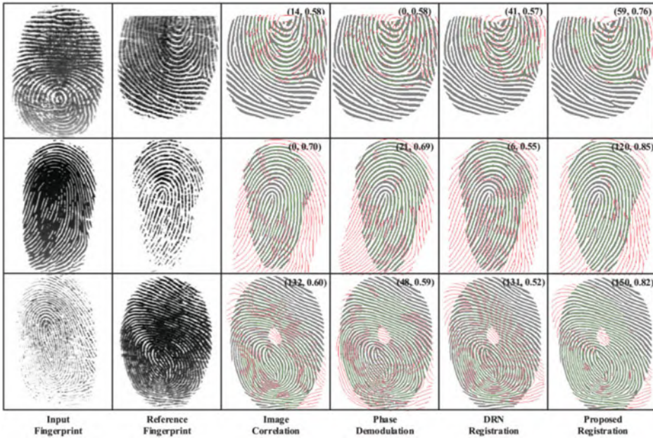
Fig. 4.21 Dense registration of 3 fingerprint pairs according to Si et al. (2017) (3rd column), Cui et al. (2018) (4th column), Cui et al. (2019) (5th column) and Cui et al. (2021) (6th column). A larger “green coverage” denotes better registration. © IEEE. Reprinted, with permission, from Cui et al. (2021)
