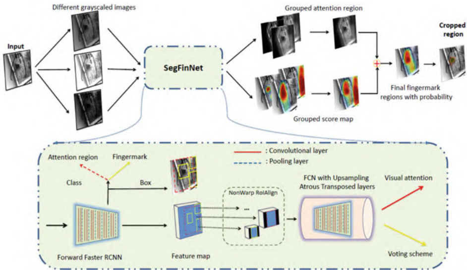
Fig. 6.13 Network architecture of SegFinNet (Nguyen et al., 2018). © IEEE. Reprinted, with permission, from Nguyen et al. (2018)
