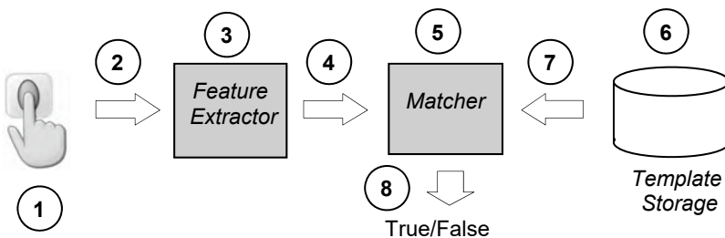
Fig. 9.3 High-level architecture of a fingerprint recognition system that illustrates the eight possible attack points identified by Ratha et al. (2001). These eight attack points can, in turn, be grouped into four broad categories: attacks at the user interface (1), attacks on the software modules (3 and 5), attacks on the communication links (2, 4, 7, and 8), and attacks on the template database (6)
