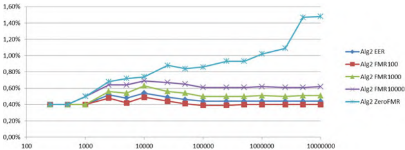
Fig. 7.34 Fingerprint verification results on a synthetic database generated by Cappelli et al. (2018), as a function of the number of fingers in the database (note that the horizontal axis uses a logarithmic scale). © IET. Reprinted, with permission, from Cappelli et al. (2018)
