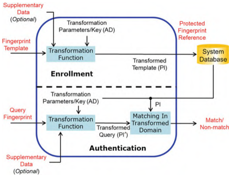
Fig. 9.20 Typical workflow of the feature transformation approach for fingerprint template protection. © IEEE. Reprinted, with permission, from Nandakumar and Jain (2015)
