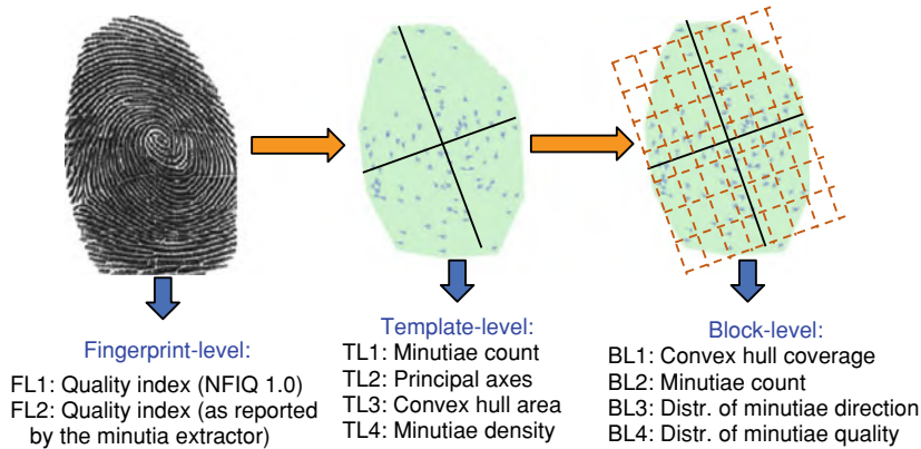
Fig. 7.33 The ten metrics in Cappelli et al. (2018). © IET. Reprinted, with permission, from Cappelli et al. (2018)
