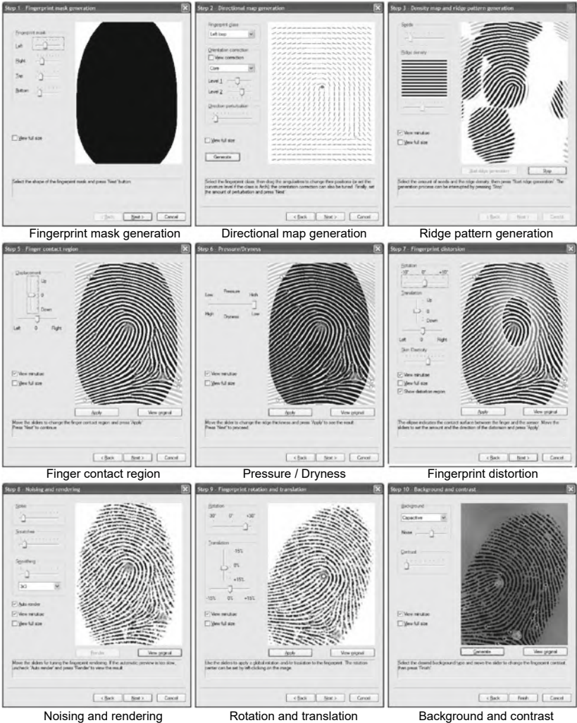
Fig. 7.43 Main steps in fingerprint generation, using the SFInGe software tool
