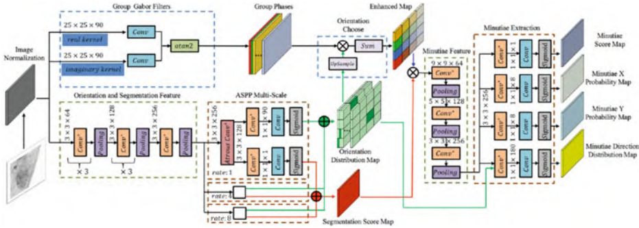
Fig. 6.24 The detailed FingerNet architecture (Tang et al., 2017). Expanded from the plain FingerNet, it can be trained end-to-end. © IEEE. Reprinted, with permission, from Tang et al. (2017)
