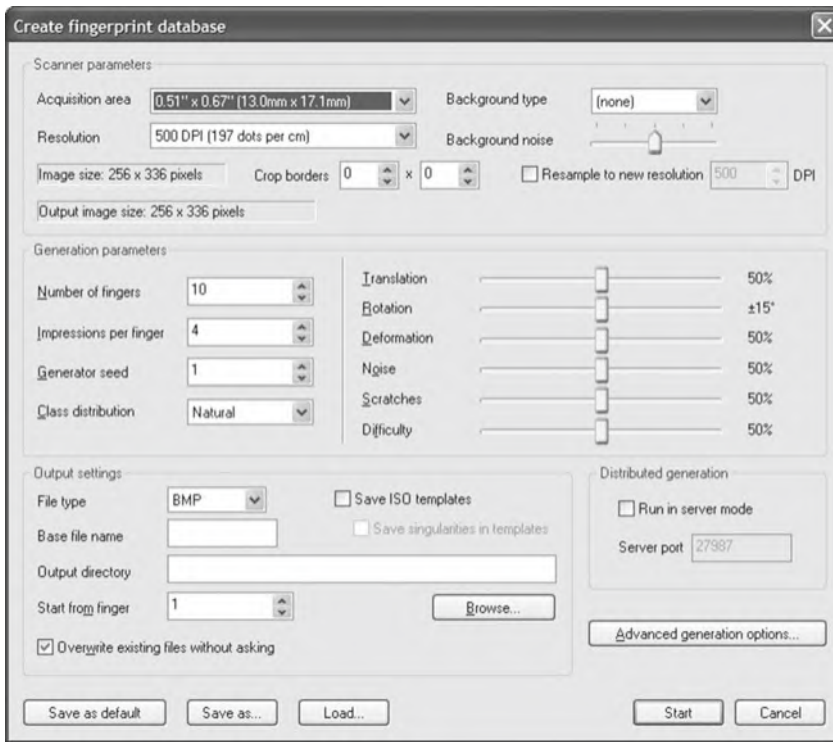
Fig. 7.42 Batch generation options of the SFinGe software
