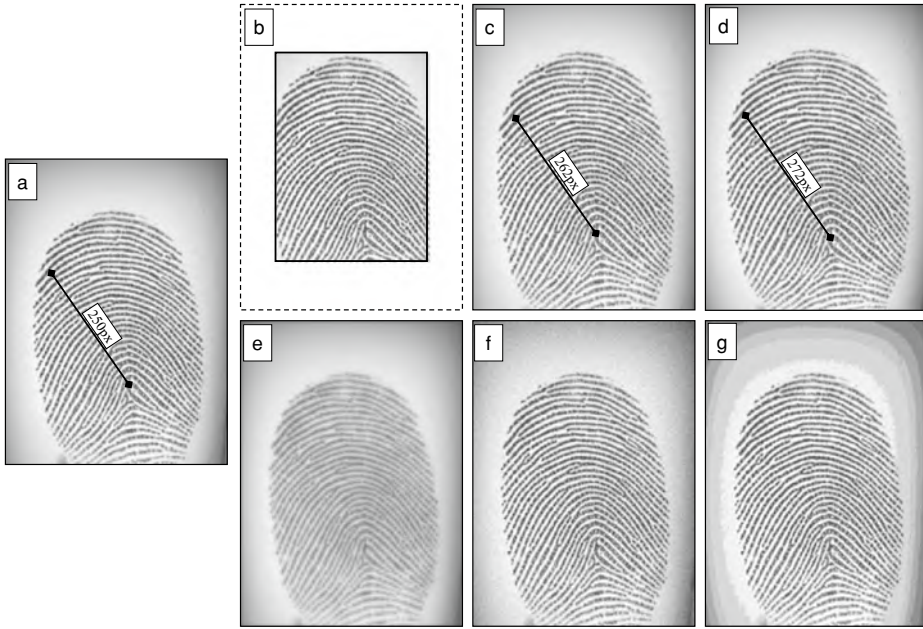
Fig. 2.22 Some examples of image degradations: a original image; b reduction of area; c change of resolution; d barrel distortion; e reduction of spatial frequency response; f reduction of SNR; g reduction of gray range
