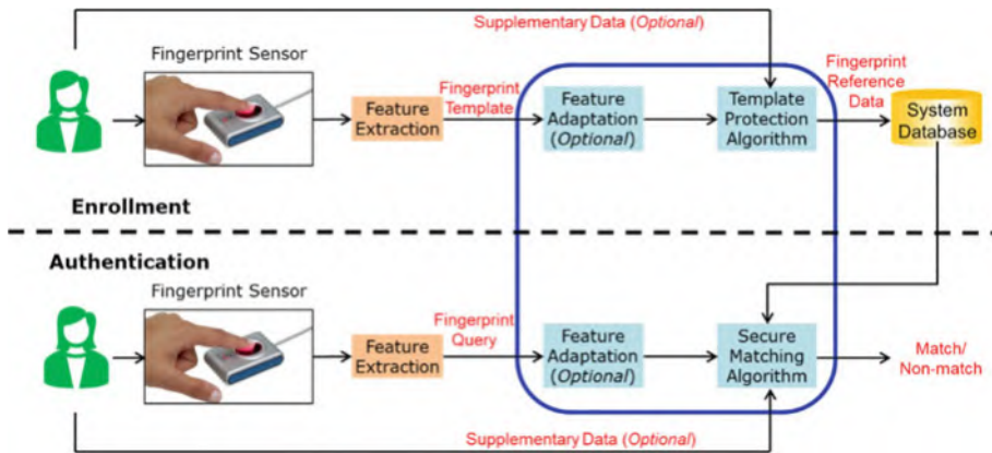
Fig. 9.19 General framework of a fingerprint system with template protection. © IEEE. Reprinted, with permission, from Nandakumar and Jain (2015)
