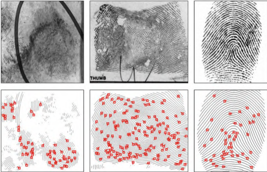
Fig. 6.6 Ridge and minutiae extraction from (left to right) a latent fingerprint and an inked rolled fingerprint in NIST DB27 and a plain fingerprint in FVC2002 DB1 by a COTS fingerprint algorithm (VeriFinger SDK 12.0)
