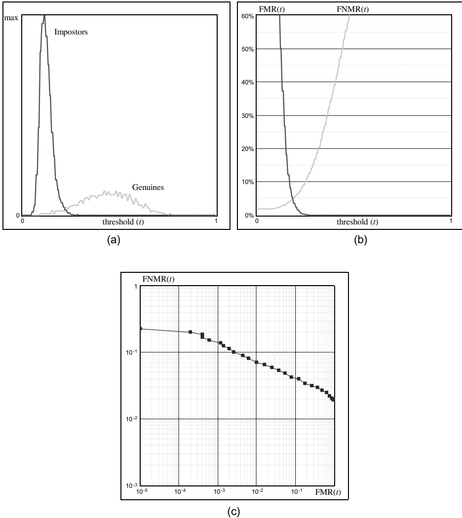
Fig. 1.4 Evaluation of a fingerprint verification algorithm over FVC2002 database DB1 (Maio et al., 2002): a genuine and impostor distributions were computed from 2800 genuine pairs and 4950 impostor pairs, respectively; b FMR(t) and FNMR(t) are derived from the score distributions in a ; c DET curve is derived from the FMR(t) and FNMR(t) curves in b
