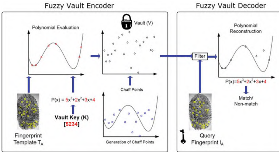
Fig. 9.25 Securing a fingerprint minutiae template using fuzzy vault
