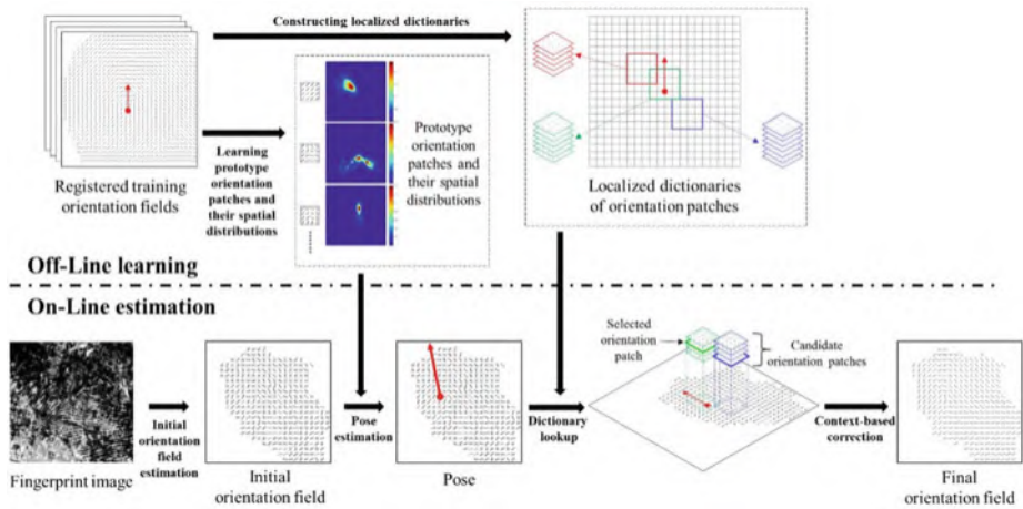
Fig. 6.16 The flowchart of orientation field estimation using localized dictionaries (Yang et al., 2014). © IEEE. Reprinted, with permission, from Yang et al. (2014)
