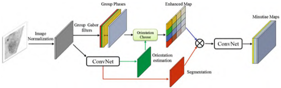
Fig. 6.23 Pipeline of plain FingerNet (Tang et al., 2017). Traditional methods consisting of orientation estimation, segmentation, Gabor enhancement, and extraction are transformed into convolutional manners and integrated as a network. © IEEE. Reprinted, with permission, from Tang et al. (2017)
