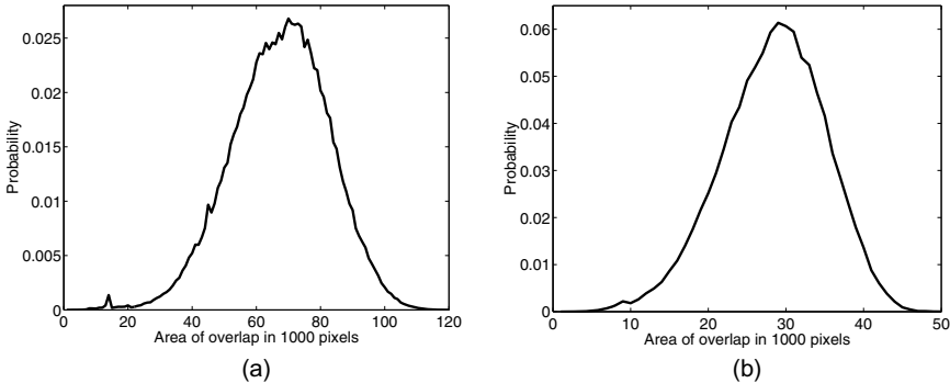
Fig. 8.5 Area of overlap between the two fingerprints that are matched based on the bounding boxes of the minutiae features for a. MSU_DBI database, b. MSU_VERIDICOM database
