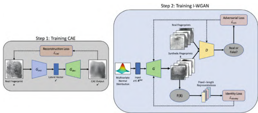
Fig. 7.27 Schema of the fingerprint synthesis approach proposed by Mistry et al. (2020). Step 1 shows the training flow of the convolutional autoencoder (as in Cao & Jain, 2018); step 2 illustrates the training of the I-WGAN ( G is the generator, whose weights are initialized using the trained weights of G_{enc} , D is the discriminator) along with the new identity loss function. Solid black arrows show the forward pass of the networks, while dotted black lines show the propagation of the losses. © IEEE. Reprinted, with permission, from Mistry et al. (2020)
