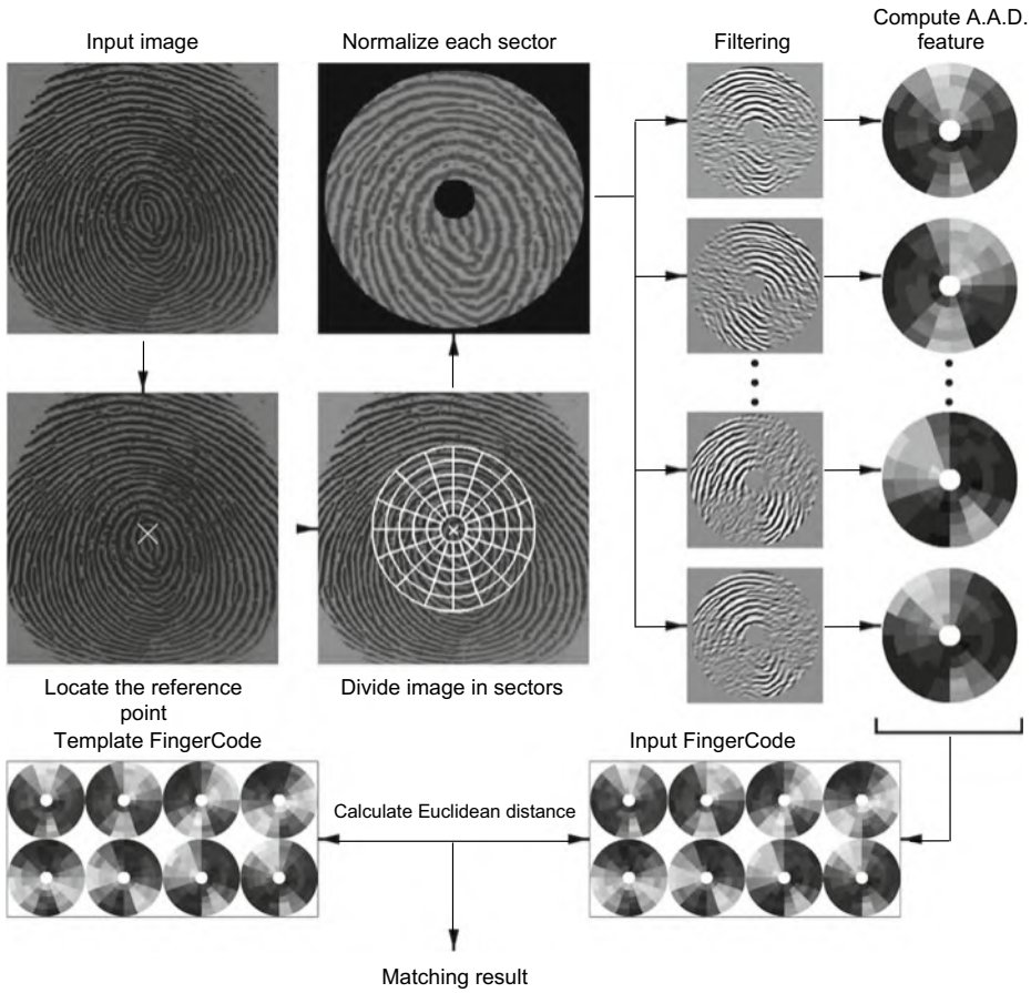
Fig. 4.24 Diagram of Jain et al.'s (2000) FingerCode approach. © IEEE. Reprinted, with permission, from Jain et al. (2000)
