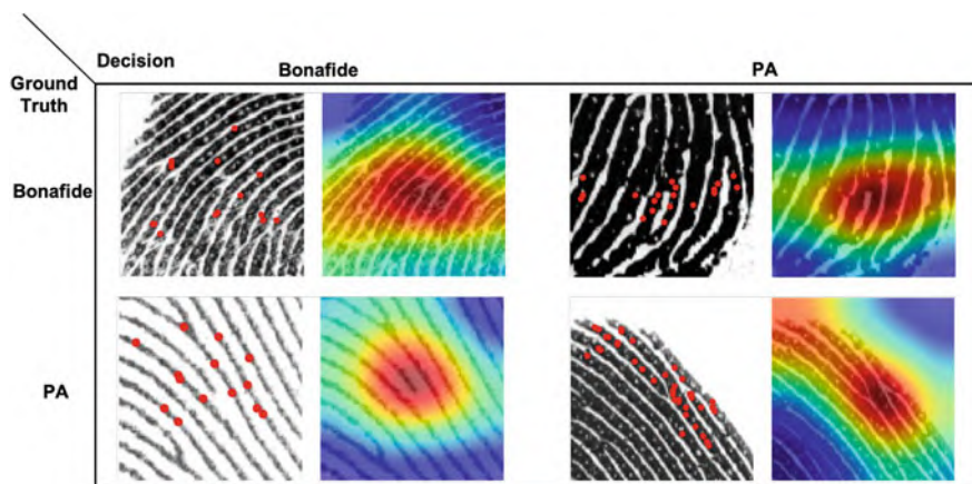
Fig. 9.18 Salient fingerprint patches that are responsible for the prediction made by a convolutional neural network (CNN)-based fingerprint PAD. These regions are identified using a visual exploration technique called CNN-Fixations (Mopuri et al., 2018). Image courtesy of Tarang Chung (Chugh, 2020)
