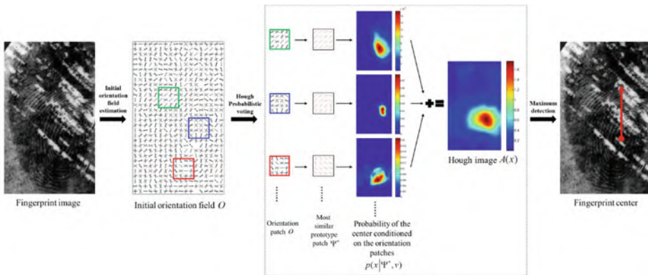
Fig. 6.10 Flowchart of estimating the finger center of an upright latent fingerprint (Yang et al., 2014). © IEEE. Reprinted, with permission, from Yang et al. (2014)
