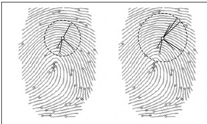
Fig. 4.12 The stars of a given minutia for d_{\max} = 70 (left) and d_{\max} = 100 (right) (Ratha et al., 2000)
