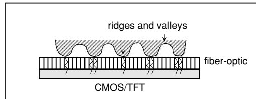
Fig. 2.8 A sensor based on optical fibers. Residual light emitted by the finger is conveyed through micro-optical guides to the array of photodetectors that constitute the CMOS or TFT backplane
