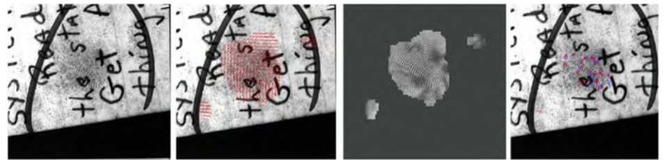
Fig. 6.26 Orientation field, foreground area, and minutiae extracted by FingerNet from a latent fingerprint (Tang et al., 2017). © IEEE. Reprinted, with permission, from Tang et al. (2017)
