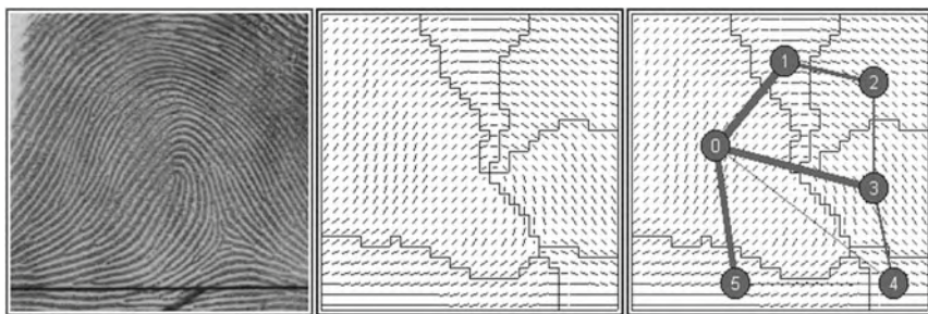
Fig. 5.5 Classification approach of Maio and Maltoni (1996): from left to right: a fingerprint image, the partitioning of its orientation image, and the corresponding relational graph. © IEEE. Reprinted, with permission, from Cappelli et al. (1999a)
