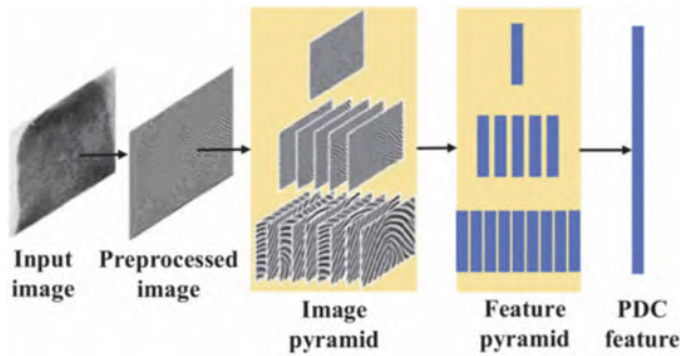
Fig. 5.12 The Pyramidal deep convolutional feature proposed by Song and Feng (2017). © IEEE. Reprinted, with permission, from Song and Feng (2017)
