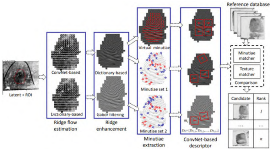
Fig. 6.36 Flowchart of the latent fingerprint recognition approach in Cao and Jain (2019). © IEEE. Reprinted, with permission, from Cao and Jain (2019)
