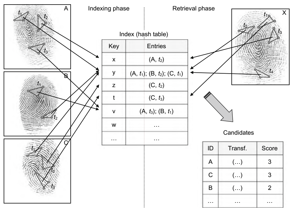
Fig. 5.11 An example of the approach proposed by Germain et al. (1997). During the indexing phase (on the left), the extracted features from each fingerprint in the database are used to generate the key values (x, y, z, ... in the figure) for the hash table; for each key value, the index maintains the list of fingerprint IDs (A, B, C) and the corresponding triplets ( t_1, t_2, \dots ). During the retrieval phase, the triplets of the input fingerprint X are computed and the list of fingerprint IDs in which that triplet is present is retrieved, together with the coordinate transformations that best map X into the database fingerprints
