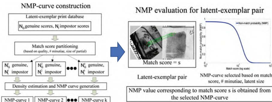
Fig. 8.7 Schematic diagram for computing the NMP value for a latent-exemplar fingerprint pair of interest based on NMP-curves obtained from a training database of latent-exemplar pairs (Nagar et al., 2012). © IEEE. Reprinted, with permission, from Nagar et al. (2012)
