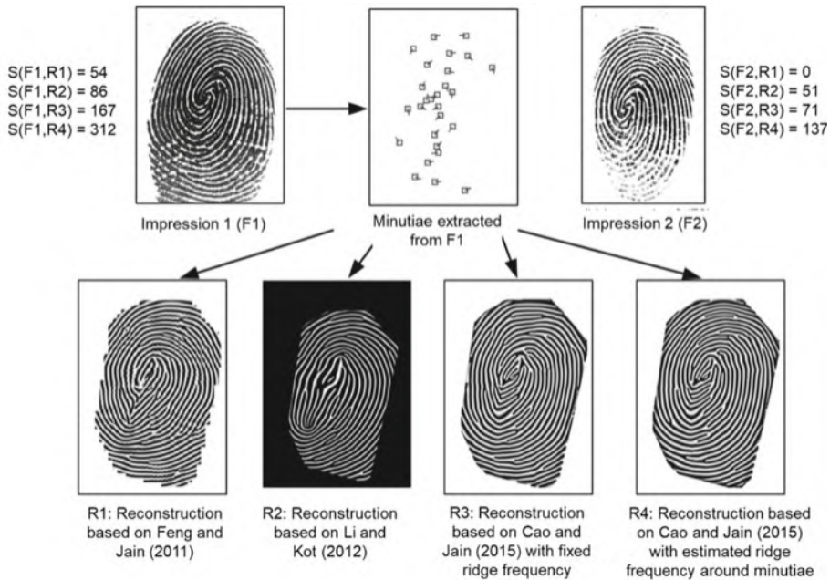
Fig. 9.5 Four examples of fingerprint image reconstruction from minutiae template. It can be observed that the reconstructed images (bottom row) match well not only with the original impression (F1) from which the minutiae template is obtained but also with a different impression (F2) of the same finger. Here, S(x,y) represents the similarity between fingerprint impressions x and y estimated by a commercial fingerprint recognition software, where match scores greater than 50 indicate a very high-confidence match. © IEEE. Reprinted, with permission, from Cao and Jain (2015)
