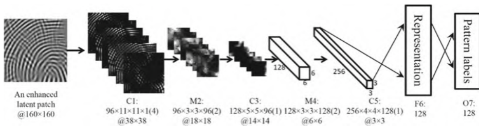
Fig. 6.20 Outline of the ConvNet architecture (Cao & Jain, 2015). There are three convolutional layers (C1, C3, and C5), two max-pooling layers (M2 and M4), a fully-connected layer (F6), and an output layer (O7). The ReLU activation function is used for each layer except the output layer. Dropout regularization is used in F6 to encourage sparsity of the neurons and to avoid overfitting. © IEEE. Reprinted, with permission, from Cao and Jain (2015)
