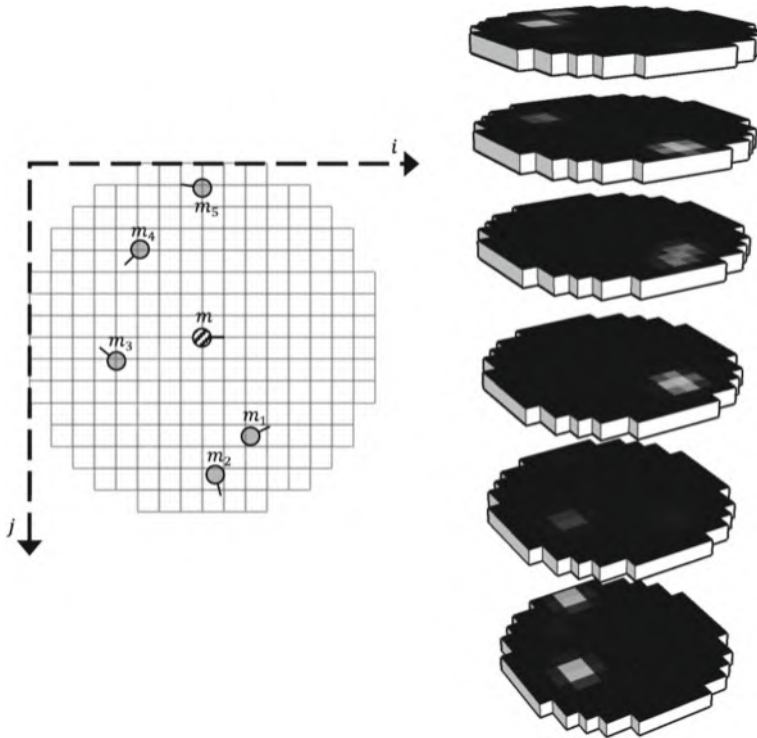
Fig. 4.15 In this example the cells of a minutia cylinder (with 6 sections) are lightened according to the position and angles of the 5 minutiae falling in the neighborhood of \mathbf{m} . Note that each neighboring minutia contribution is not limited to a single cell but is maximum in a given cell and smoothly fades along both the spatial and angular dimension: this increases robustness against small inaccuracies in the minutiae locations and angles
