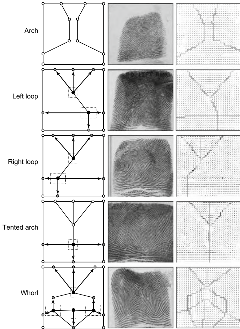
Fig. 5.6 Classification scheme of Cappelli et al. (1999a): the templates corresponding to the five classes and an example of application of each template to the orientation image of a fingerprint belonging to the corresponding class. © IEEE. Reprinted, with permission, from Cappelli et al. (1999a)
