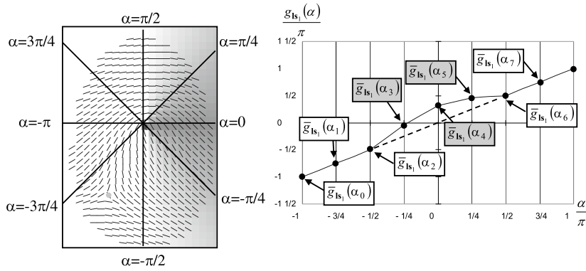
Fig. 7.10 The effects of modifying the parameters that control a mapping function g_k(\alpha) are highlighted in the corresponding orientation image (Vizcaya & Gerhardt, 1996)
