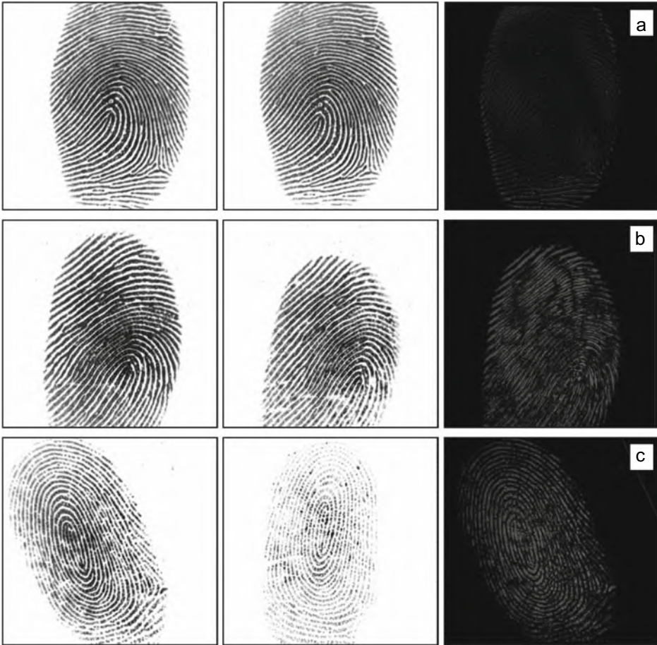
Fig. 4.3 Each row shows two impressions of the same finger and the absolute value of their difference (residual) for the best alignment (i.e., that maximizes correlation). In the first row, a the two impressions are very similar and the corresponding images correlate well (the residual is very small). In the second row, b , and third row, c , due to high distortion and skin condition, respectively, the residuals are high and the global correlation methods fail
