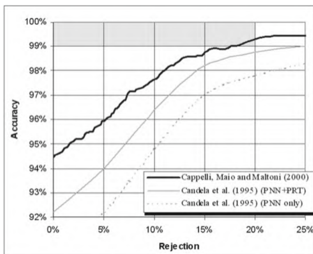
Fig. 5.9 Accuracy versus rejection curves. PCASYS performance was manually sampled from the graph reported by Candela et al. (1995). The gray area denotes the target accuracy of automatic classification set by the FBI. Probabilistic Neural Network alone (PNN only) and combined with the auxiliary Pseudo Ridge Tracing module (PNN + PRT)
