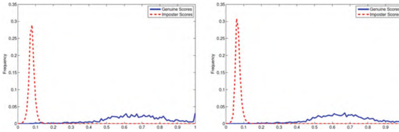
Fig. 7.29 Genuine and imposter match score distributions (Zhao et al., 2012): on a synthetic database (on the left) and a real database (on the right). © IEEE. Reprinted, with permission, from Zhao et al. (2012)
