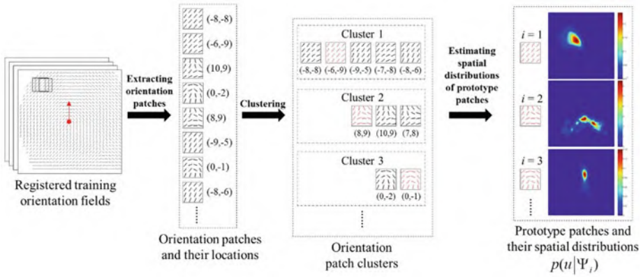
Fig. 6.9 In the offline stage, the prototype orientation patches and their spatial distributions are learnt from a set of registered training orientation fields (Yang et al., 2014). © IEEE. Reprinted, with permission, from Yang et al. (2014)
