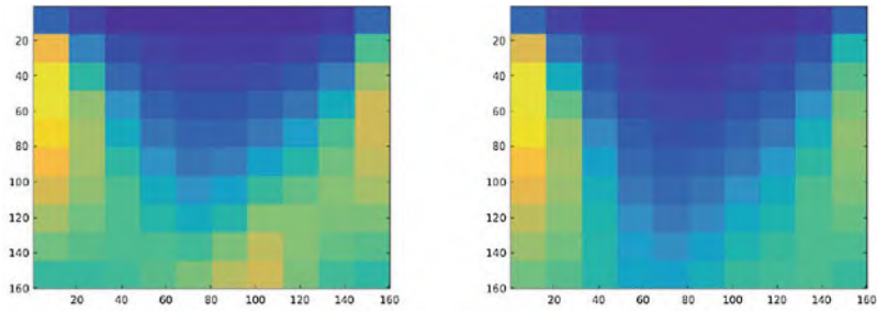
Fig. 7.32 Average 2D minutiae histograms: on the left the histogram was computed over a real database (NIST DB4), on the right over a database generated by the synthesis approach proposed in Cao and Jain (2018). © IEEE. Reprinted, with permission, from Cao and Jain (2018)
