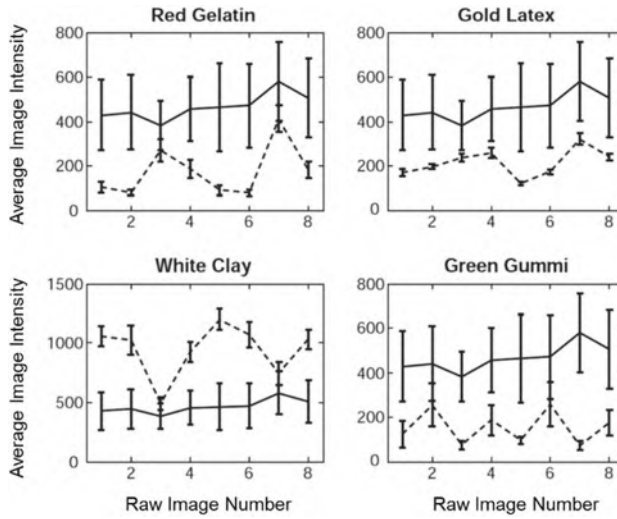
Fig. 9.12 Spectral differences between bonafide fingers and various fingerprint spoof types captured using a multi-spectral fingerprint scanner. The average image intensity for each of the eight direct-illumination images obtained by the scanner is plotted for bonafide fingers (solid lines, repeated in the four plots) and spoofs (dotted lines, different for each plot). Error bounds represent three standard deviations of the measured population for each sample class. It can be observed that all the selected spoof types are separable from bonafide fingers based on their average spectral properties. © Springer Nature. Reprinted, with permission, from Rowe et al. (2008)
