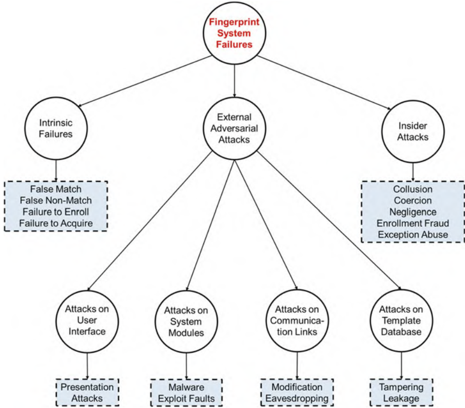
Fig. 9.2 A taxonomy of attacks that can be mounted on fingerprint systems
