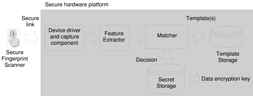
Fig. 9.28 In System-on-a-chip architecture, all the processing is done within the confines of a secure chip. Even if the scanner is physically separated from the chip, the communication channel can be protected by embedding the cryptographic keys into both the hardware (the scanner and the chip)
