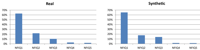
Fig. 7.31 Distribution (histogram) of NFIQ classes: on the left from a real database, on the right from a synthetic database generated by the improved technique described in Cappelli et al. (2018)
