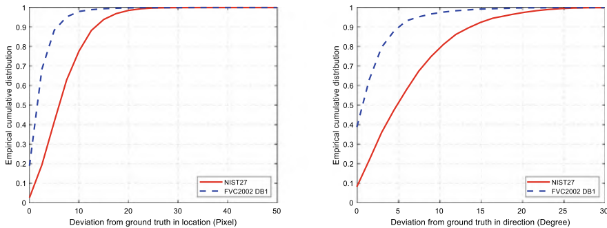
Fig. 6.32 Cumulative error distribution of the distance and angle difference between mated minutiae point pairs after rigid registration. To ensure that the deformation is calculated according to the correct minutiae pairing, latent-to-rolled registration on NIST DB27 is based on manually matched minutiae by latent examiners. Fingerprint registration on FVC2002 DB1 is performed based on automatically matched minutiae
