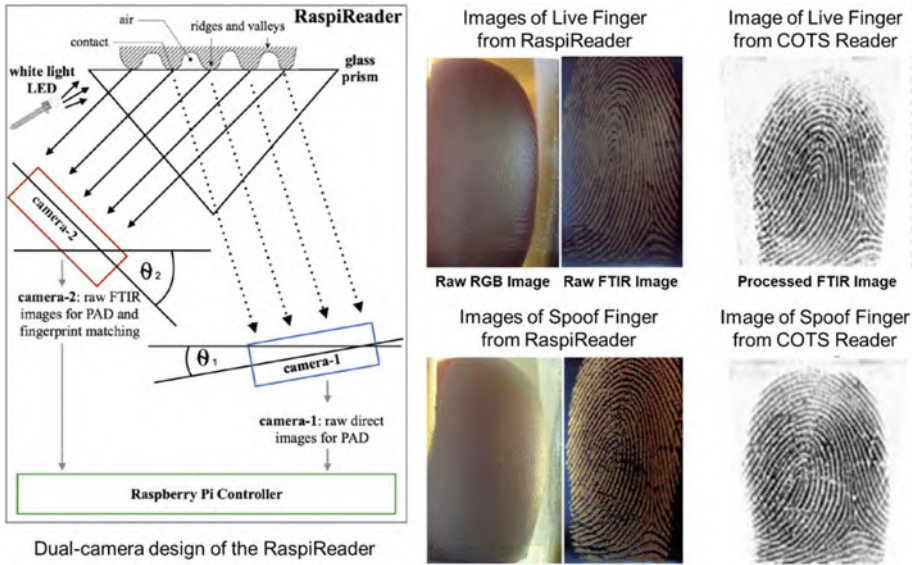
Fig. 9.13 Illustration of the open-source fingerprint reader called RaspReader, which uses a dual-camera setup to provide two complementary streams of information useful for spoof detection (left column). While the raw images captured by the RaspReader (middle column) are significantly different for live and spoof fingers, no such distinction can be observed in the images captured by a commercial-off-the-shelf (COTS) optical fingerprint reader (right column). © IEEE. Reprinted, with permission, from Engelsma et al. (2019)
