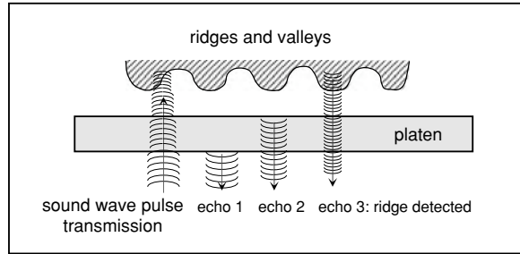
Fig. 2.17 The basic principle of the ultrasound technique. A characteristic of sound waves is their ability to penetrate materials, giving a partial echo at each impedance change
