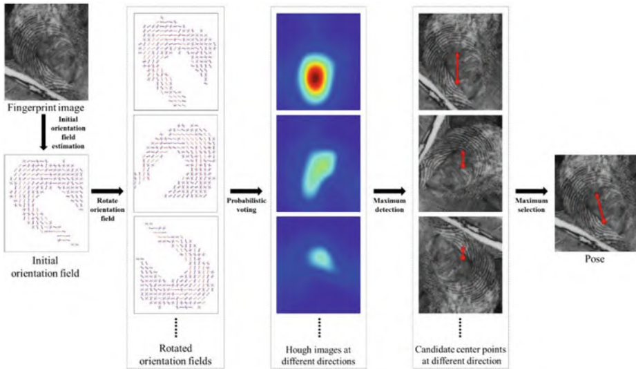
Fig. 6.11 Pose estimation of a latent fingerprint with unknown direction (Yang et al., 2014). The initial orientation field is rotated by a set of possible angles; the finger center estimation procedure is then applied to detect the center at each angle; and finally, the one with the largest confidence value is chosen. © IEEE. Reprinted, with permission, from Yang et al. (2014)
