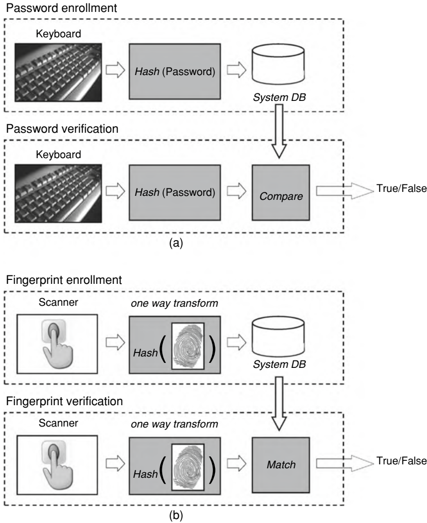
Fig. 9.23 Hashing approach for fingerprint template protection. a Passwords are typically stored in the database after they are hashed; when a new password is received, it is hashed and compared with the hashed enrollment. If a person has access to the database of hashed passwords, a password is not compromised. In b , a similar analogy is applied to fingerprint recognition. Only a robust hash of the original fingerprint template is stored and thus, if an adversary has access to the database, the fingerprint information is not compromised
