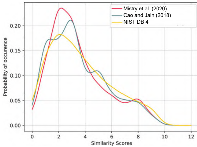
Fig. 7.30 Imposter match score distributions on a synthetic database generated by Mistry et al. (2020), a synthetic database generated by Cao and Jain (2018), and a real database. © IEEE. Reprinted, with permission, from Mistry et al. (2020)
