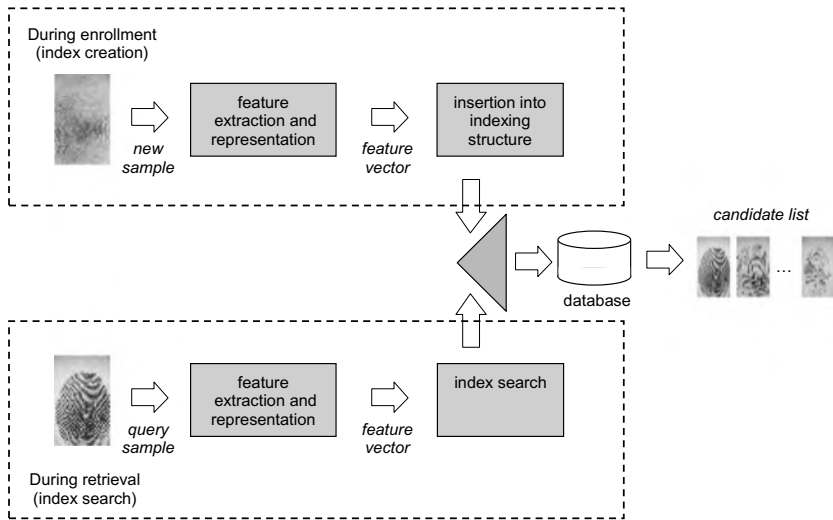
Fig. 5.10 Conceptual schema of indexing and retrieval
