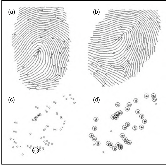
Fig. 4.9 Minutiae matching by the Chang et al. (1997) approach. Figures a and b show the minutiae extracted from the template and the input fingerprint, respectively; c the minutiae are coarsely superimposed and the principal pair is marked with an ellipse; d each circle denotes a pair of minutiae as mated by the Step 3 of the algorithm
