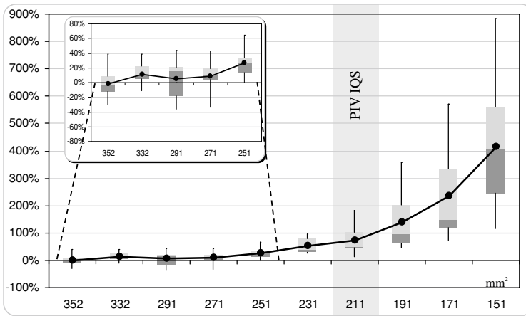
Fig. 2.23 Box-plot of the acquisition area experiment: each box graphically shows the descriptive statistics of the test carried out over the ten algorithms. The first five boxes are expanded in the inset graph to better show their statistics. The horizontal axis reports the minimum acquisition area requirements (in square millimeters) and the vertical axis shows the percentage performance drop. The minimum requirement based on the PIV IQS specification is highlighted (211 mm 2 )
