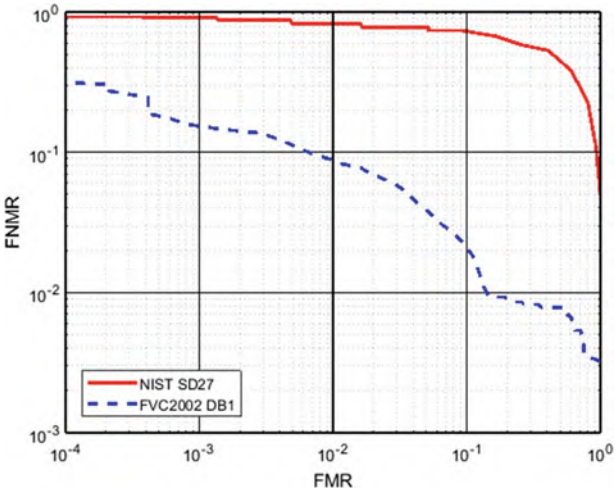
Fig. 6.34 DET curves of VeriFinger SDK 12.0 on NIST DB27 and FVC2002 DB1. Verification mode is used to make the matching performances on two databases comparable
