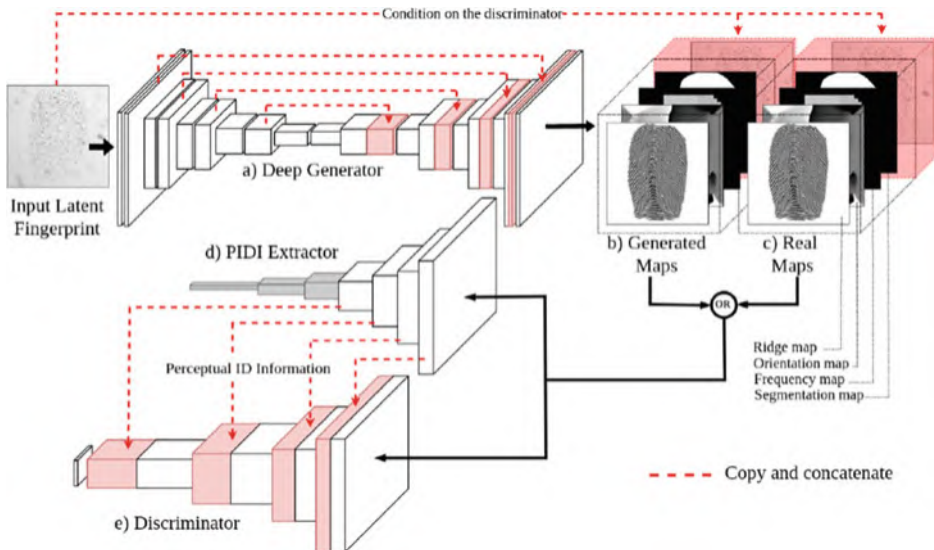
Fig. 6.27 Complete diagram of the cGAN model for latent fingerprint reconstruction (Dabouei et al., 2018). © IEEE. Reprinted, with permission, from Dabouei et al. (2018)
