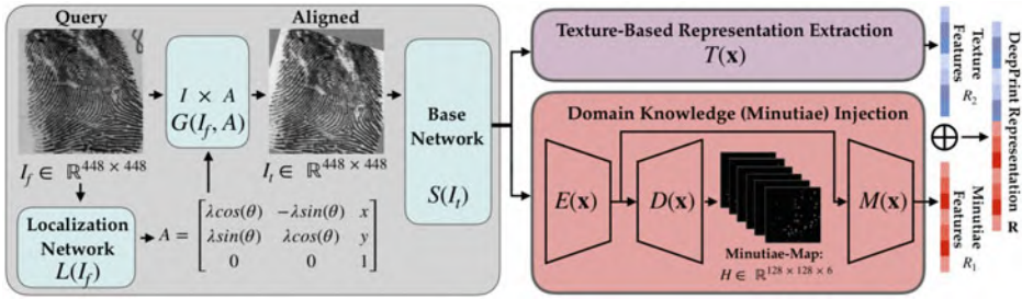
Fig. 4.25 Functional diagram of the DeepPrint approach by Engelsma et al. (2021). © IEEE. Reprinted, with permission, from Engelsma et al. (2021)
