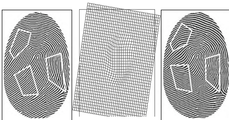
Fig. 7.21 A master fingerprint (on the left) and a distorted impression (on the right); the equivalent distortion of a square mesh is shown in the middle. To better highlight the non-linear deformations, a few corresponding minutiae are connected by white segments in the two images
