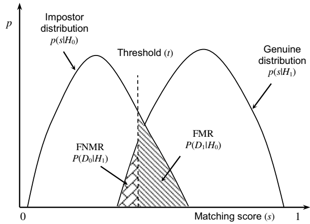
Fig. 1.3 FMR and FNMR for a given threshold t are displayed over the genuine and impostor score distributions. Note that FMR is the percentage of impostor pairs whose comparison score is greater than or equal to t , and FNMR is the percentage of genuine pairs whose comparison score is less than t
