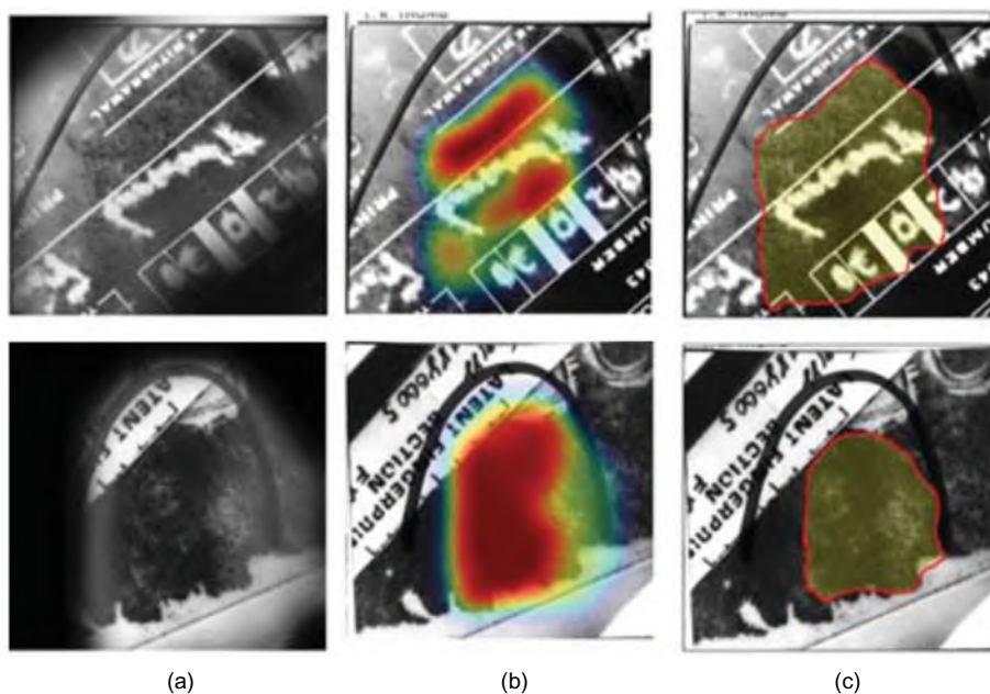
Fig. 6.14 SegFinNet (Nguyen et al., 2018) with visual attention mechanism for two different input latent fingerprints, one per row: a Focused region from visual attention module; b Original latent fingerprints overlaid with a heat map showing the probability of occurrence of friction ridges (from high to low); c Binary mask (boundary marked in red). © IEEE. Reprinted, with permission, from Nguyen et al. (2018)
