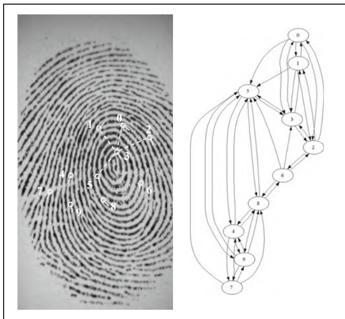
Fig. 4.16 Chikkerur et al. (2006): the graphs built from the K -plets of a fingerprint image; the K -plet of the node 3 is highlighted over the fingerprint image. © Springer Nature. Reprinted, with permission, from Chikkerur et al. (2006).
