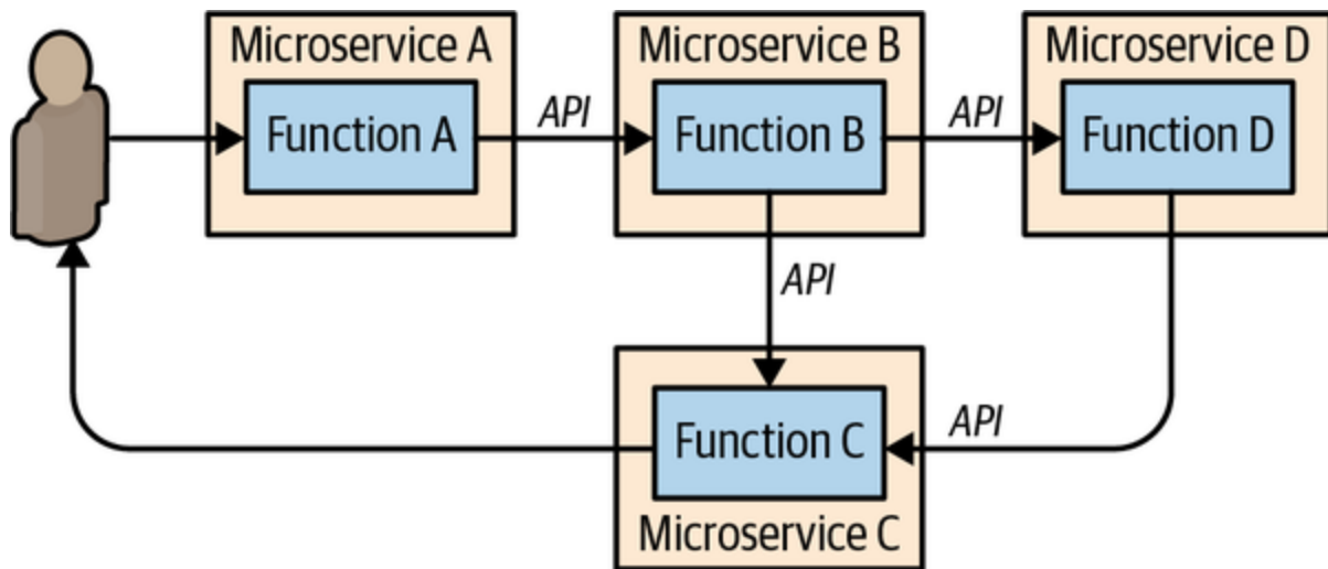
Figure III-2. A microservice architecture with each function broken out as a separate microservice
