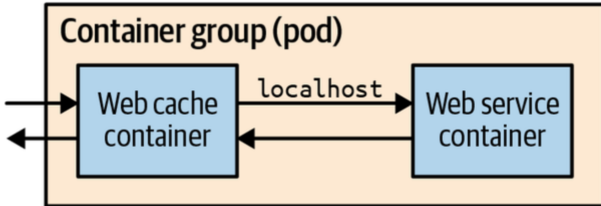
Figure 6-5. Adding the web cache server as a sidecar
