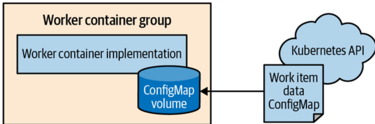
Figure 11-4. The work queue worker API
