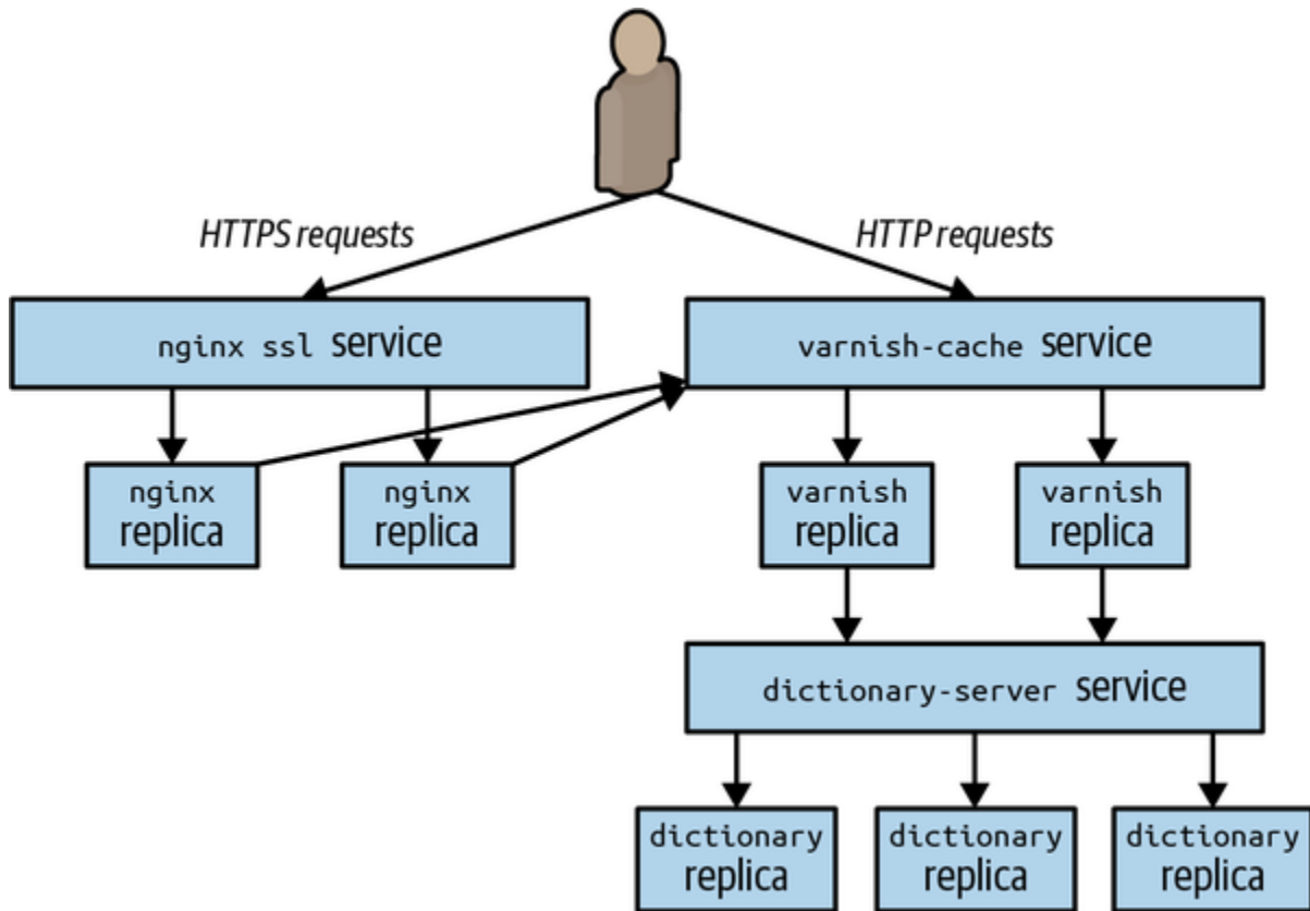
Figure 6-8. Complete replicated stateless serving example
