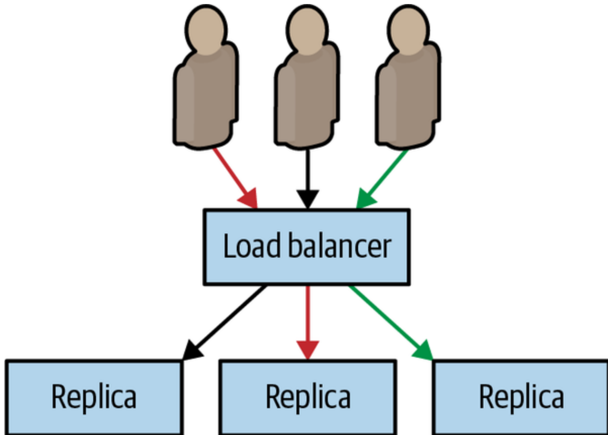
Figure 6-3. A session tracked service where all requests for a specific user are routed to a single instance
