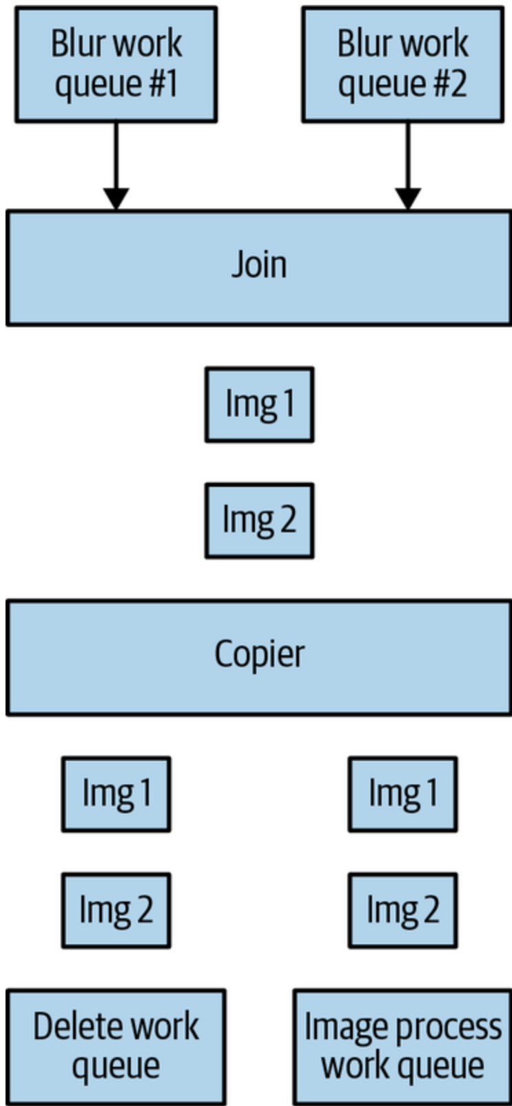
Figure 13-4. The output join, copier, deletion, and image recognition parts of the pipeline
