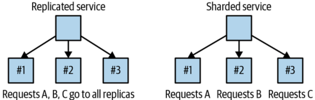
Figure 7-1. Replicated service versus sharded service
