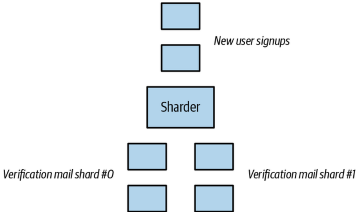
Figure 12-8. The first stage of the workflow for user signup
