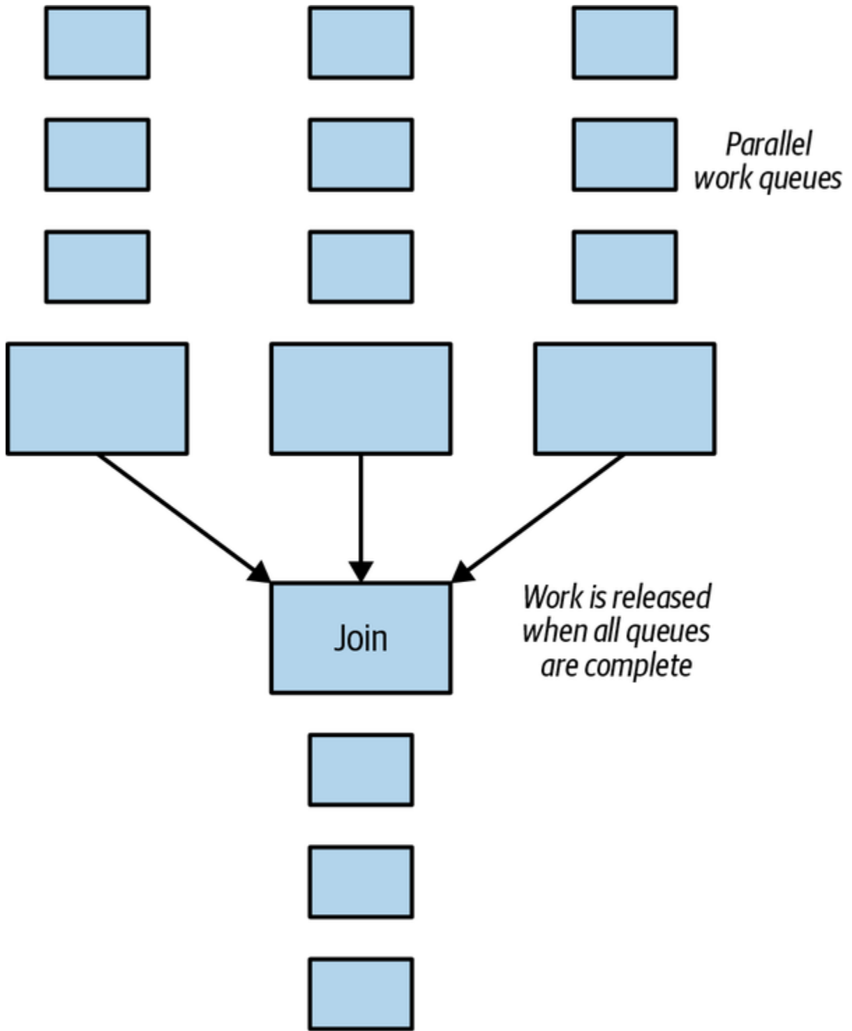
Figure 13-2. The join pattern for batch processing
