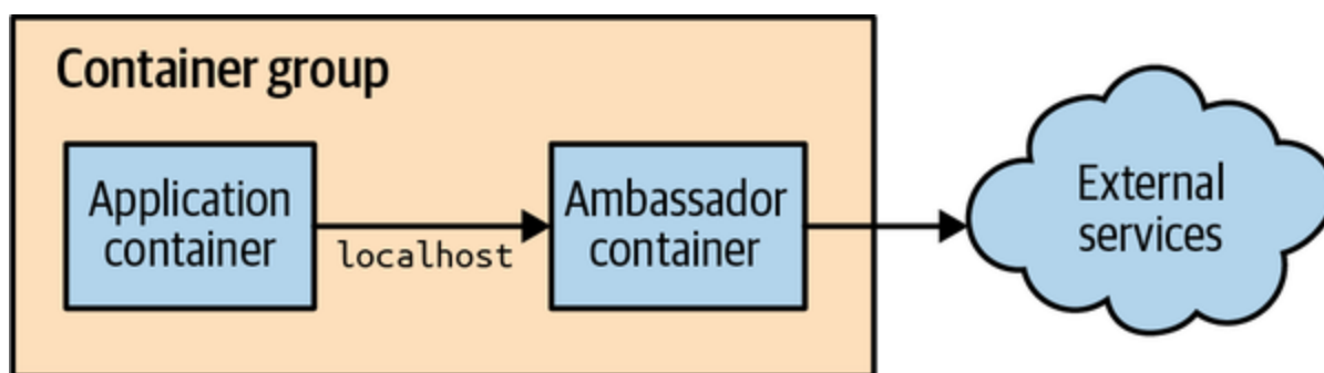
Figure 4-1. Generic ambassador pattern
