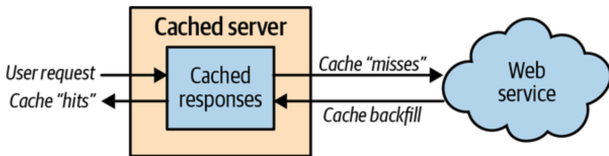
Figure 6-4. The operation of a cache server
