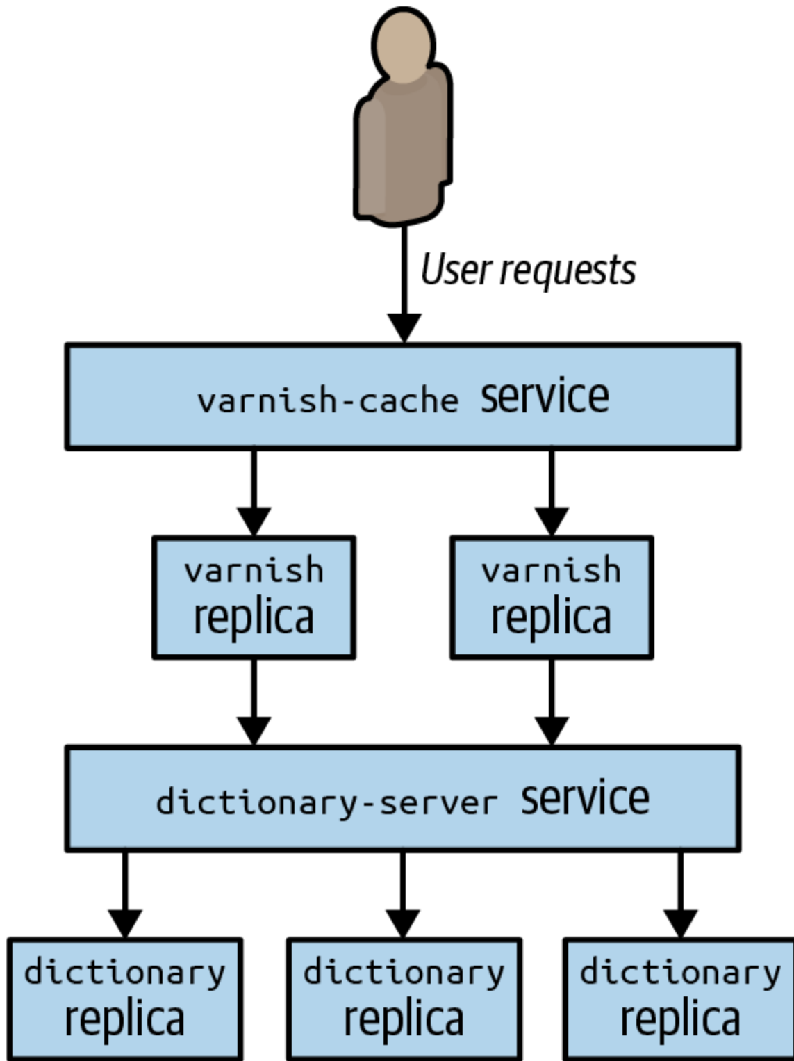
Figure 6-7. Adding a caching layer to the dictionary server
