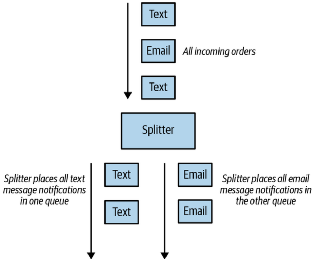
Figure 12-4. An example of the batch splitter pattern splitting shipping notifications into two different queues
