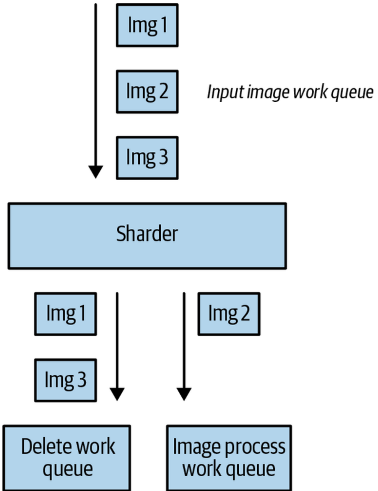
Figure 13-3. The sharded work queue and the multiple blurring shards
