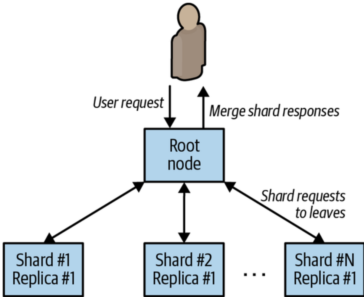
Figure 8-1. A scatter/gather pattern
