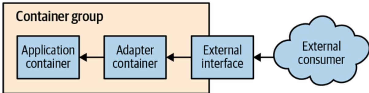
Figure 5-1. The generic adapter pattern
