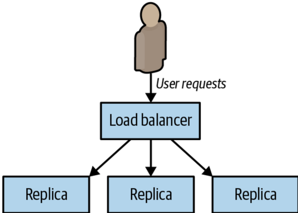
Figure 6-1. Basic replicated stateless service
