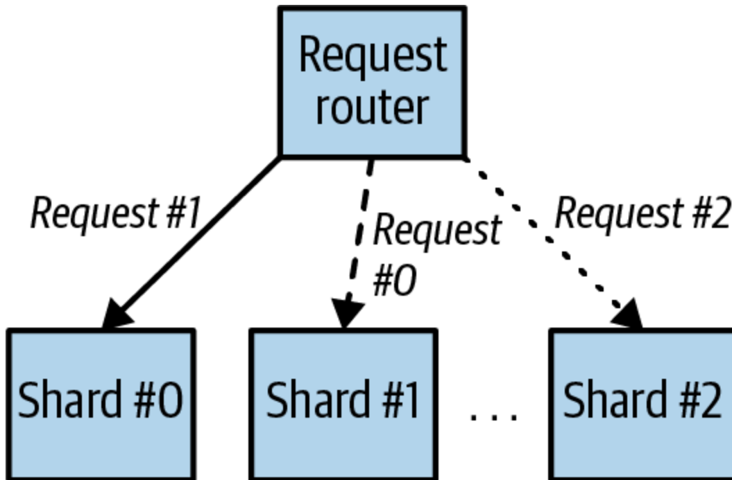
Figure 4-2. A generic sharded service
