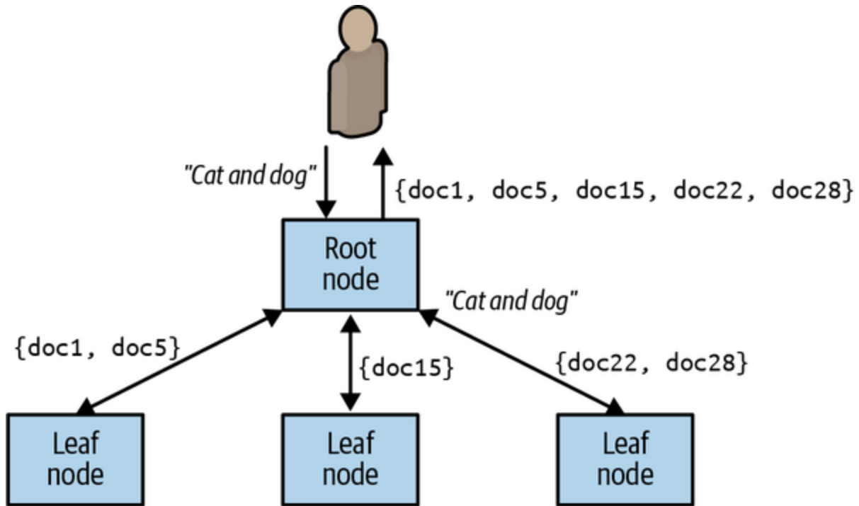
Figure 8-3. Conjunctive query executing in a scatter/gather search system
