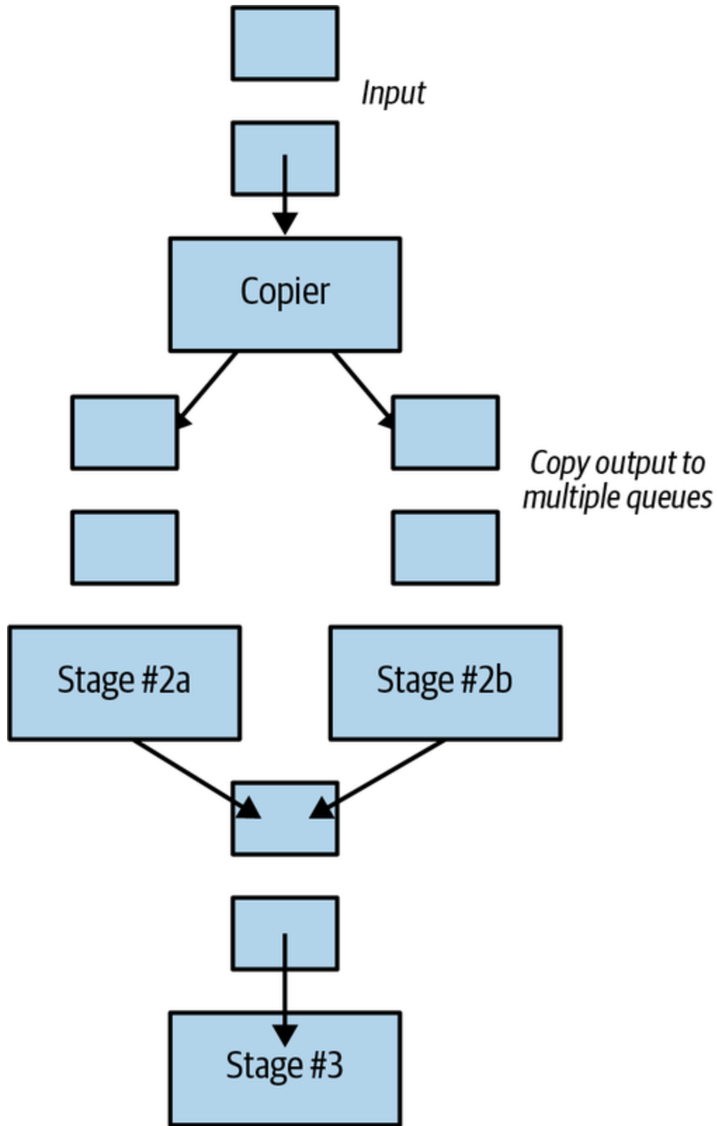
Figure 12-1. This workflow combines copying work into multiple queues (Stage 2a, 2b), parallel processing of those queues, and combining the result back into a single queue (Stage 3)
