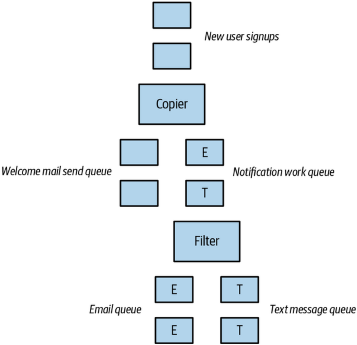
Figure 12-9. The user notification and welcome email work queue
