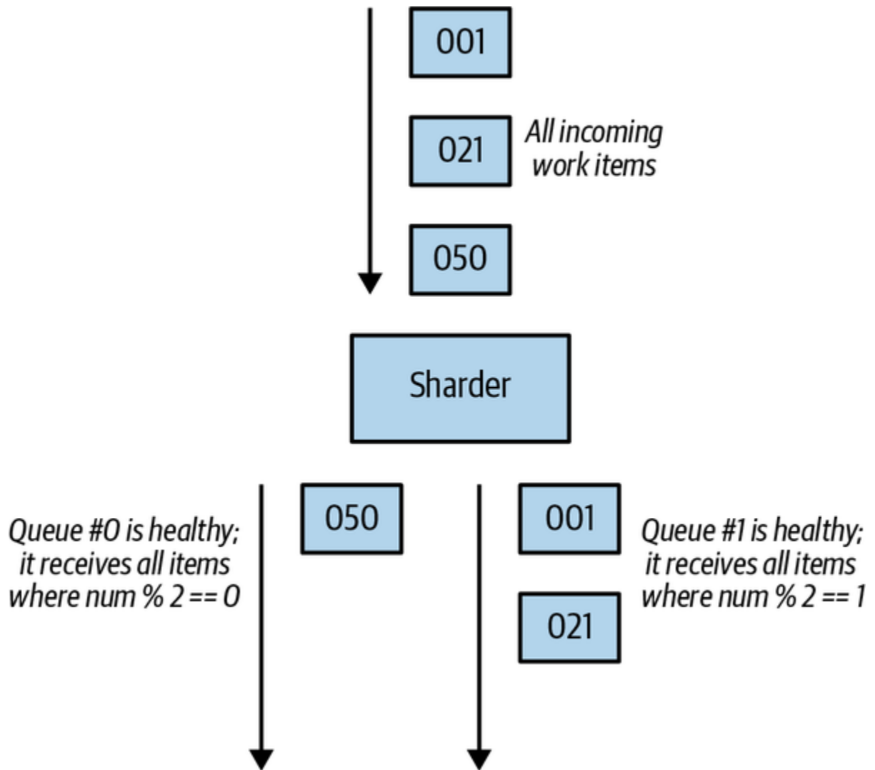
Figure 12-5. An example of the sharding pattern in a healthy operation
