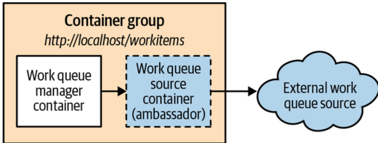
Figure 11-3. The work queue container group
