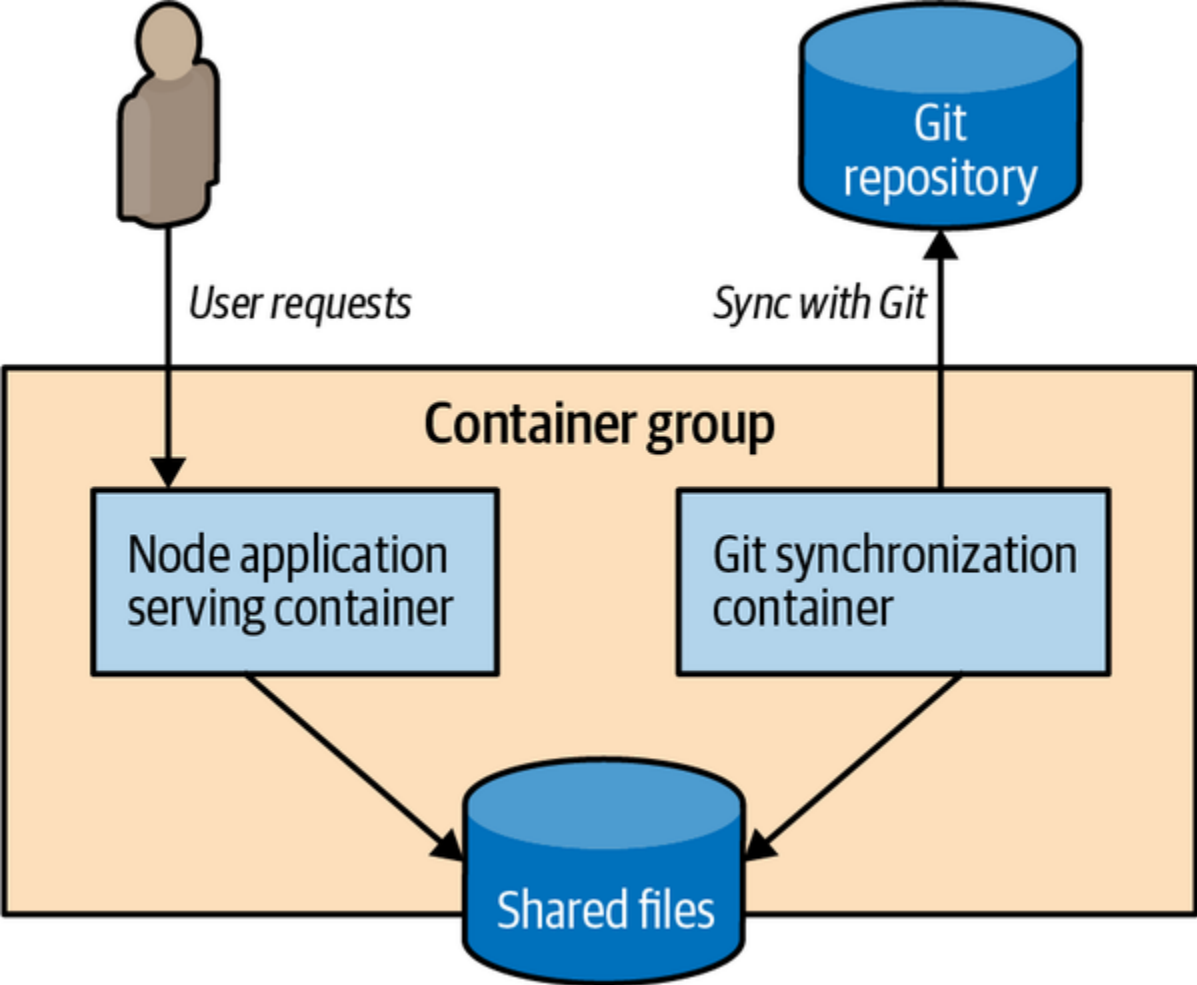
Figure 3-4. A simple sidecar-based PaaS
