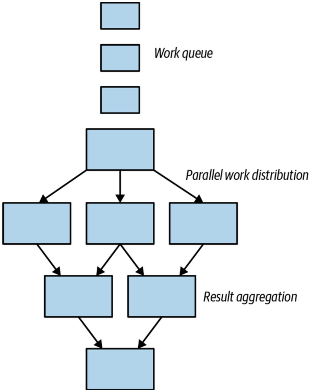
Figure 13-1. A generic parallel work distribution and result aggregation batch system
