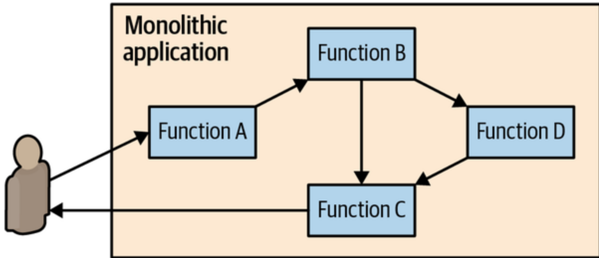
Figure III-1. A monolithic service with all functions in a single container
