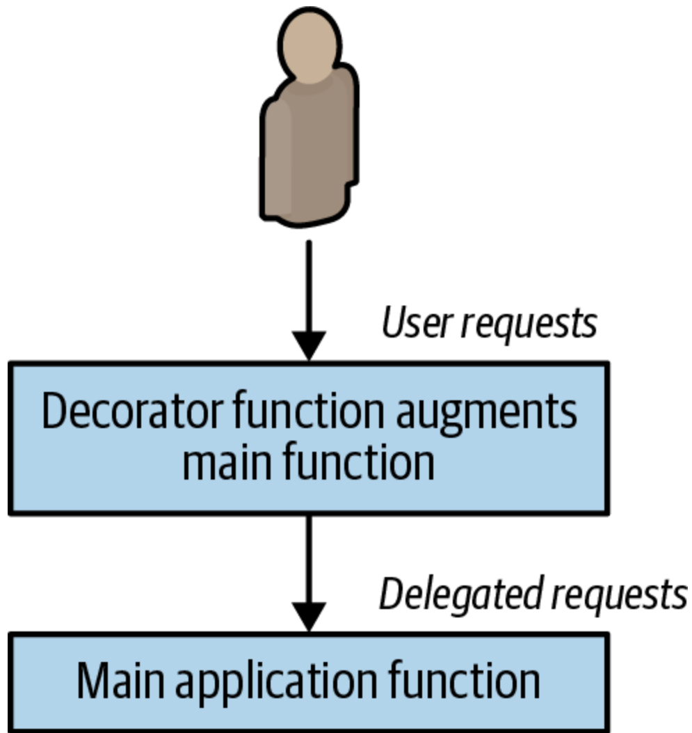
Figure 9-1. The decorator pattern applied to HTTP APIs
