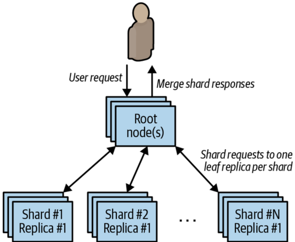
Figure 8-4. A sharded replicated scatter/gather system
