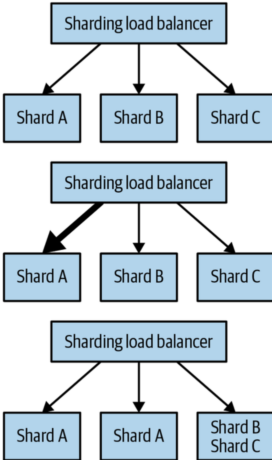
Figure 7-3. An example of a hot sharded system: initially the shards are evenly distributed, but when extra traffic comes to shard A, it is replicated to two machines, and shards B and C are combined on
