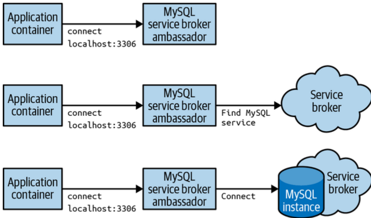
Figure 4-3. A service broker ambassador creating a MySQL service
