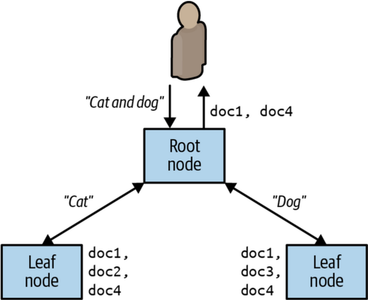
Figure 8-2. Example of a term-sharded scatter/gather system
