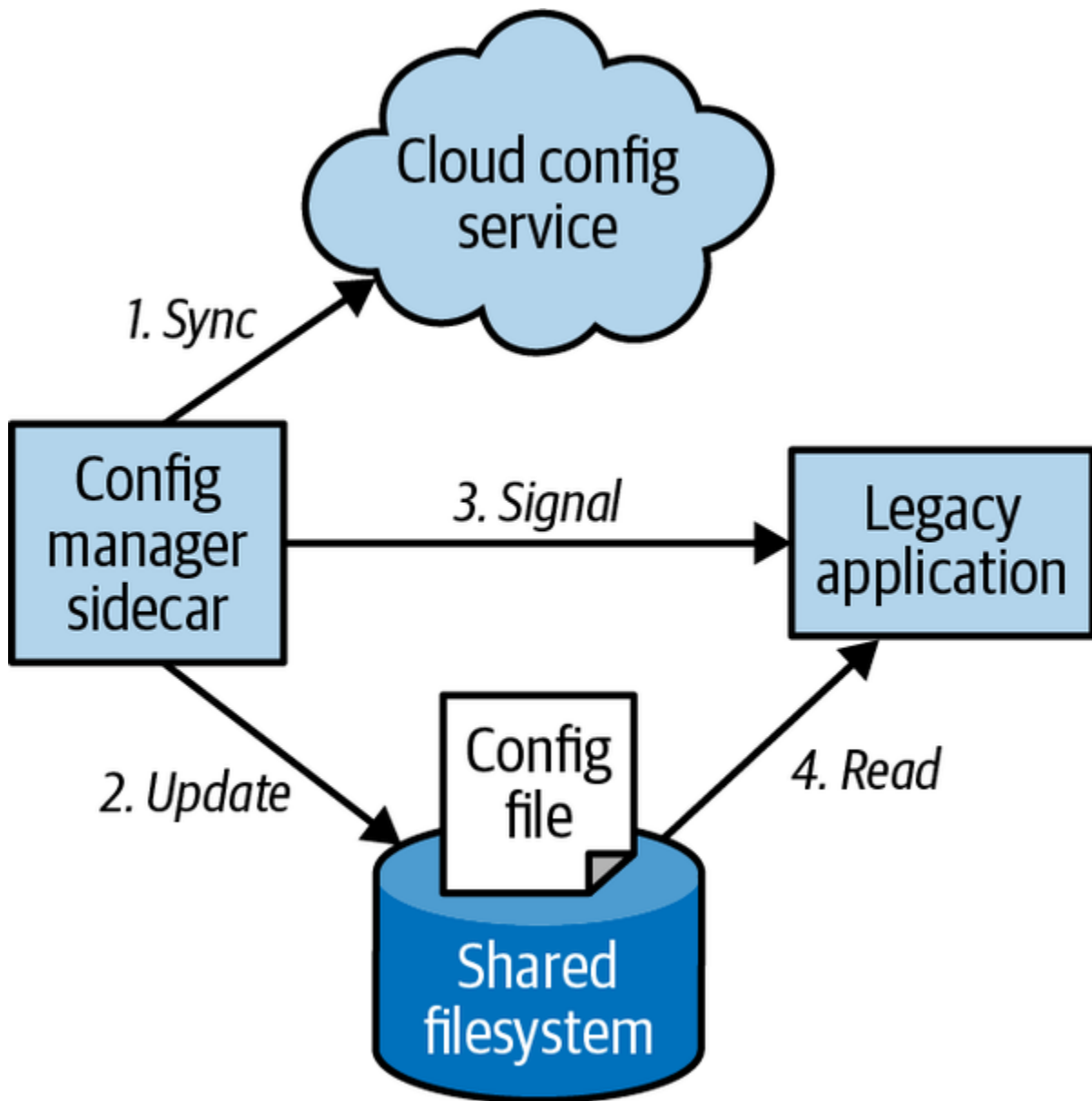
Figure 3-3. A sidecar example of managing a dynamic configuration
