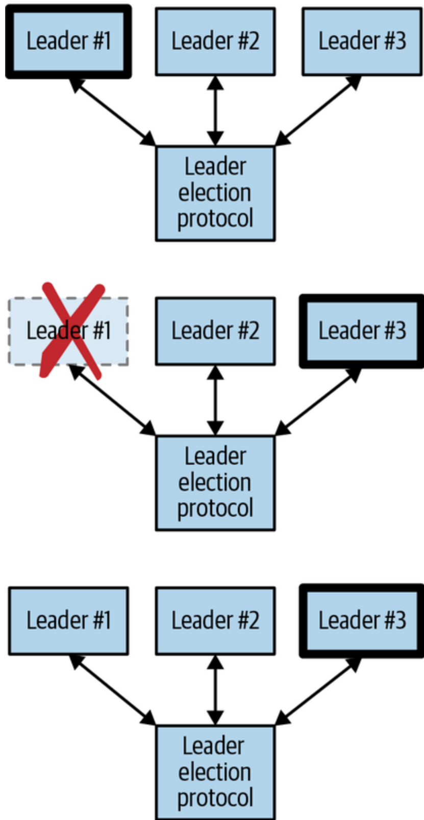
Figure 10-1. A leader election protocol in operation: initially the first leader is selected, but when it fails, the third leader takes over
