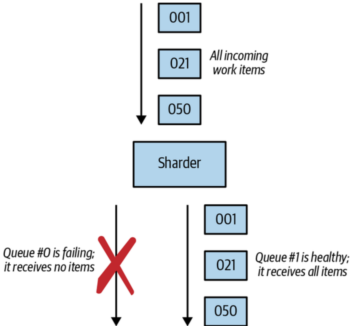
Figure 12-6. When one work queue is unhealthy, the remaining work spills over to a different queue
