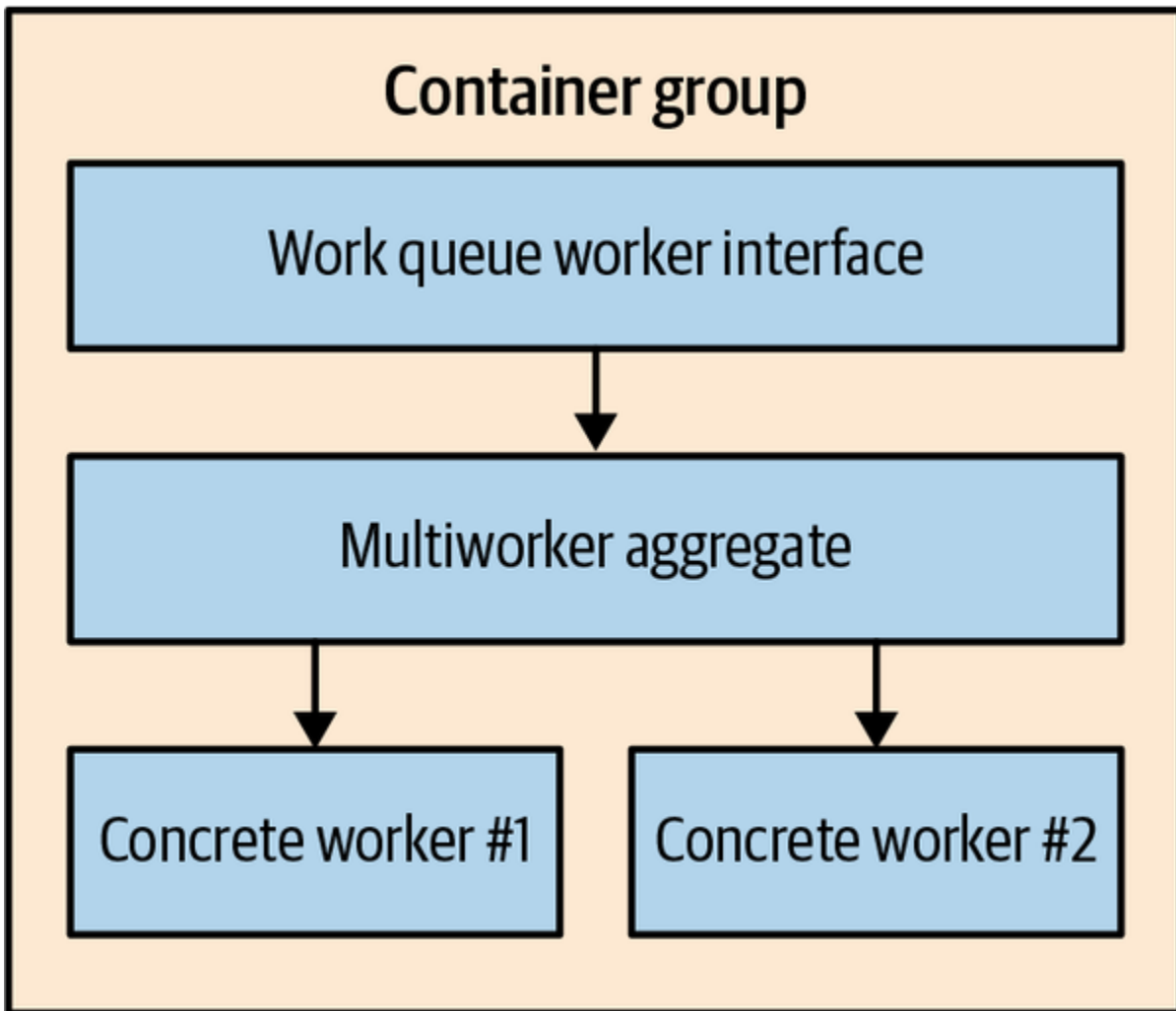
Figure 11-5. The multiworker aggregator pattern as a group of containers
