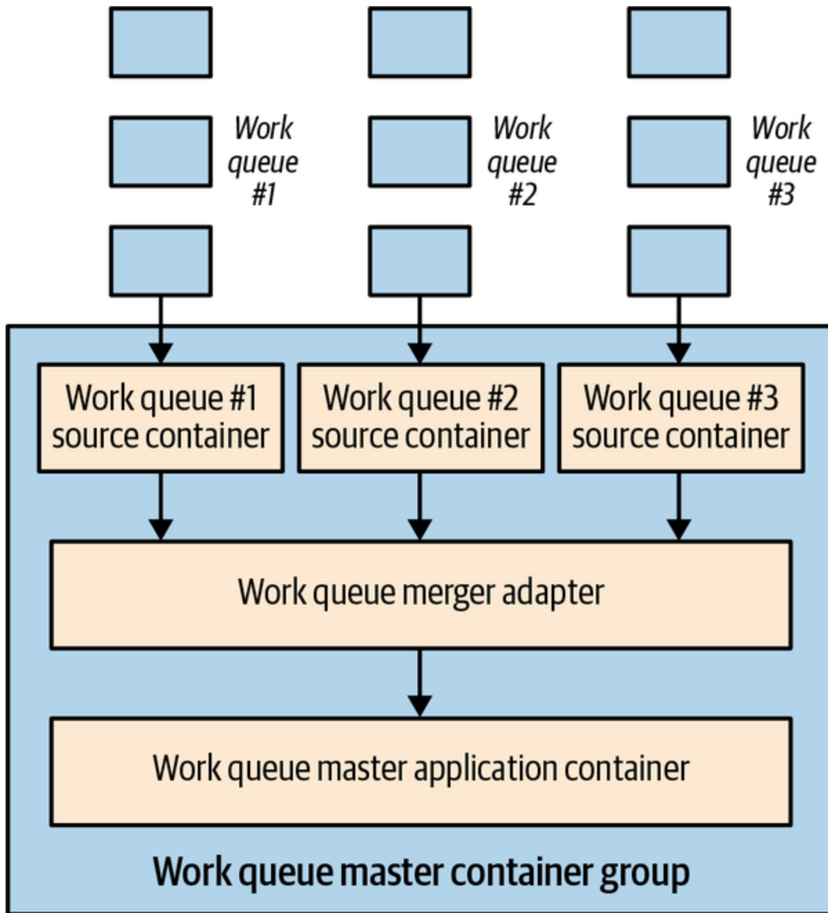
Figure 12-7. Using multiple levels of containers to adapt multiple independent work queues into a single shared queue
