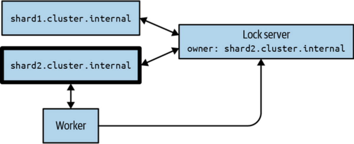
Figure 10-2. A worker double-checking to validate that the requester who sent a message is actually the current owner of the shard
