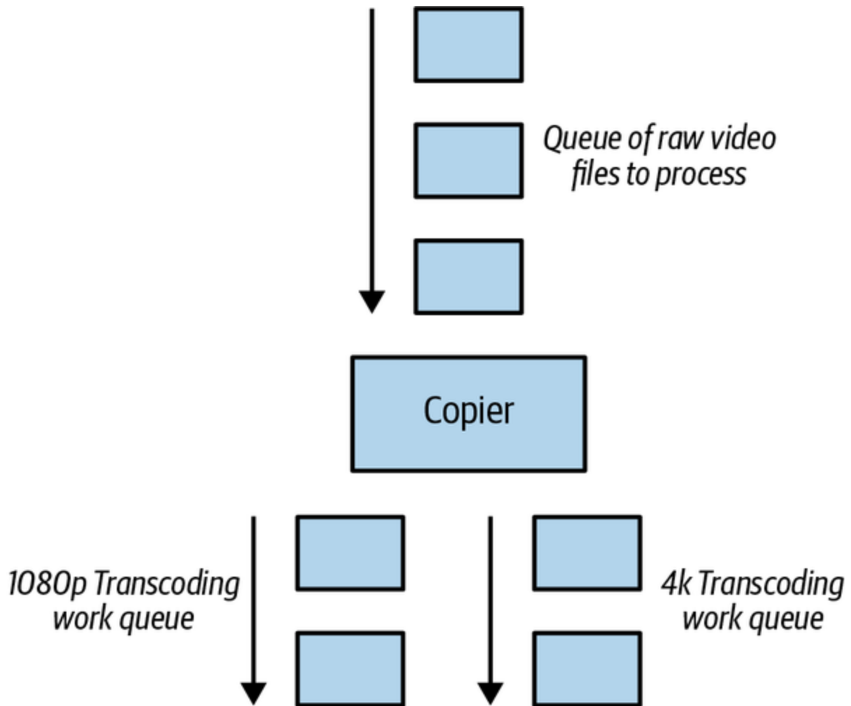
Figure 12-2. The copier batch pattern for transcoding
