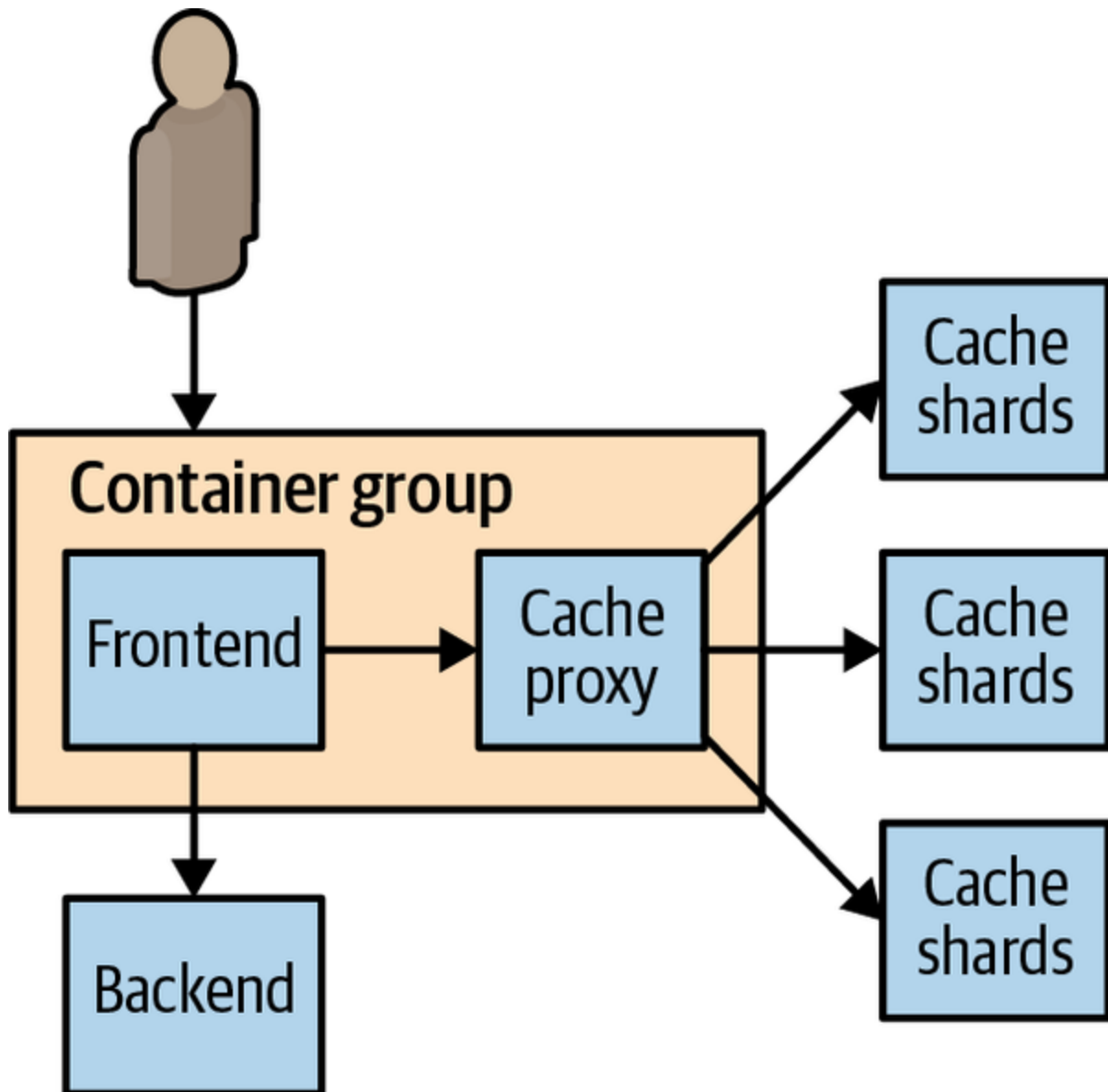
Figure 7-2. A sharded cache
