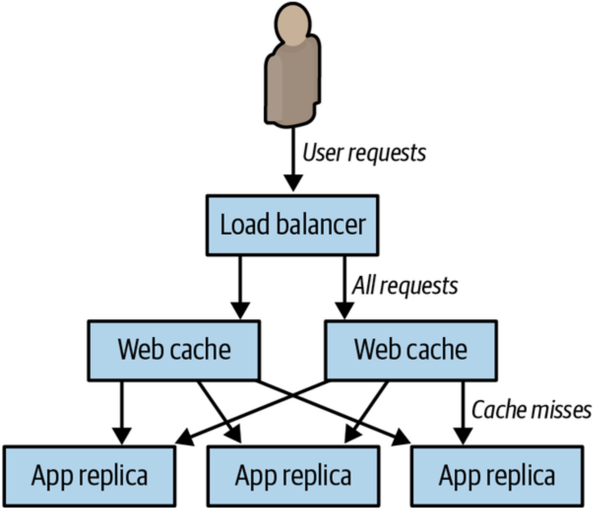
Figure 6-6. Adding the caching layer to our replicated service
