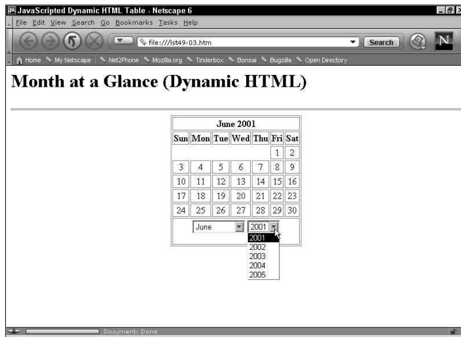
Figure 49-3: DHTML table
