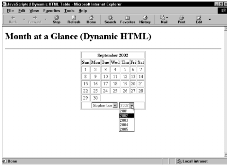
Figure V-2: With IE4+ and NN6, calendar tables can be dynamic.
