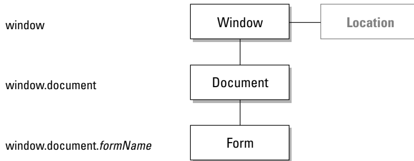
Figure 4-12: Reference to the form object
