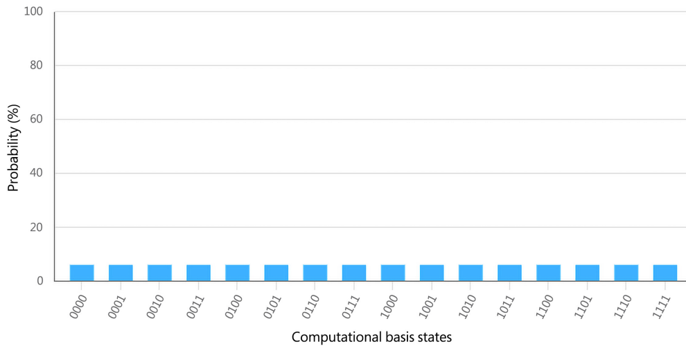
Figure 10.17: Plot showing all 16 states of the basis, each one with an equal probability of 6.25%
