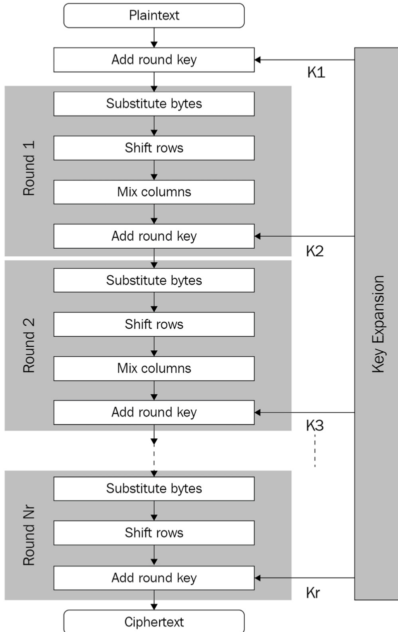
Figure 2.29: Encryption scheme in AES
