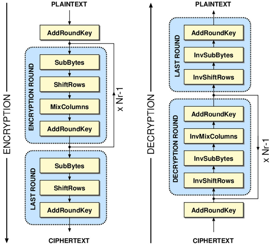
Figure 2.31: Encryption and decryption scheme in AES
