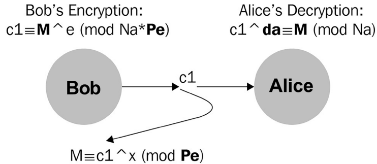
Figure 6.8: A schema of Bob's self-reverse attack
