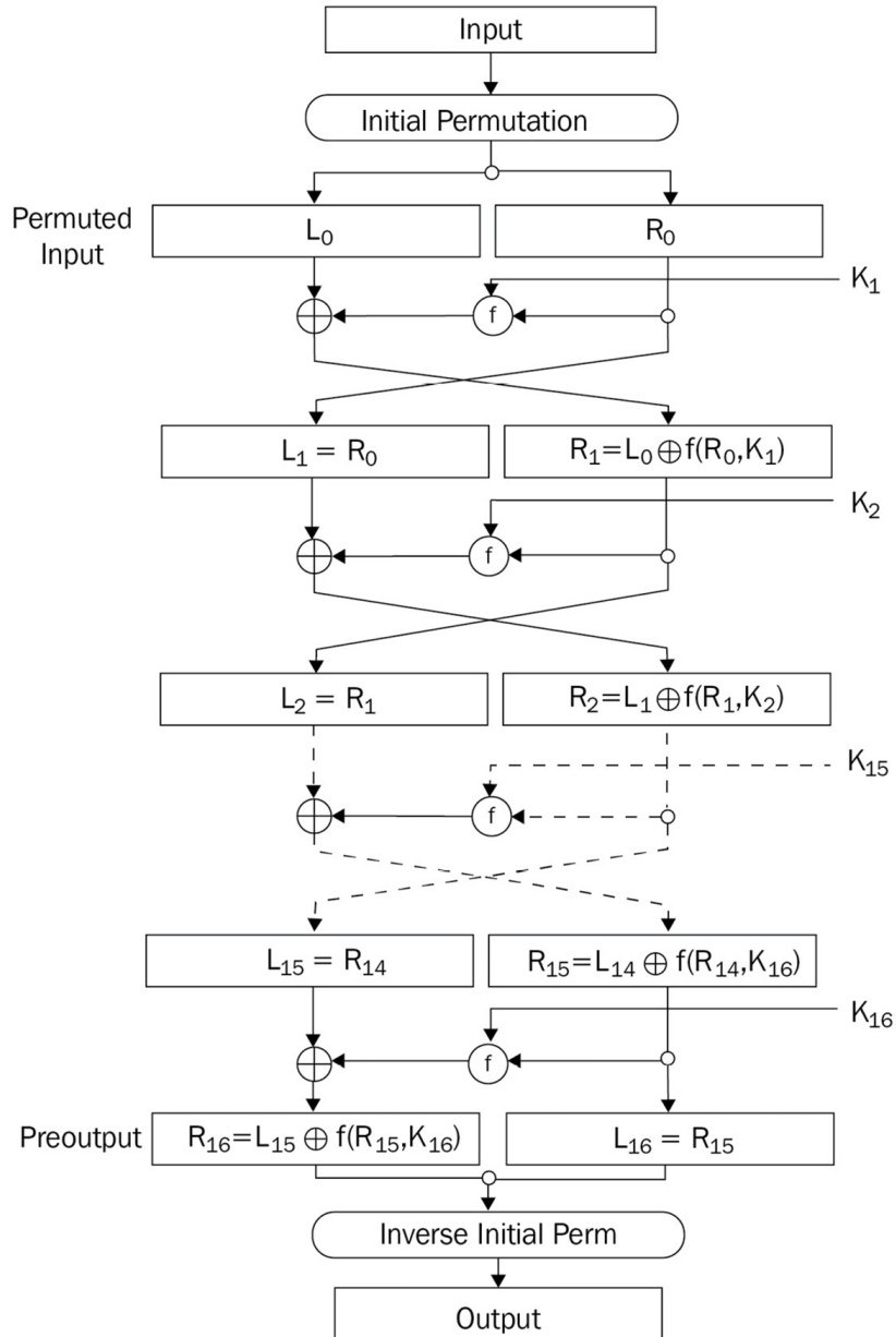
Figure 2.21: DES encryption
