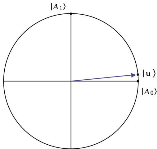
Figure 10.24: State of superposition of |u\rangle
