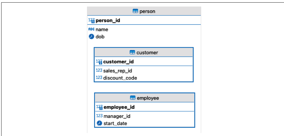
Figure 5-4. Logical model with subtypes
