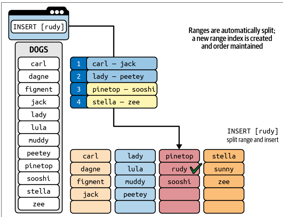
Figure 2-14. Range splits
