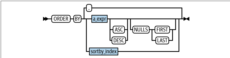
Figure 4-3. ORDER BY
