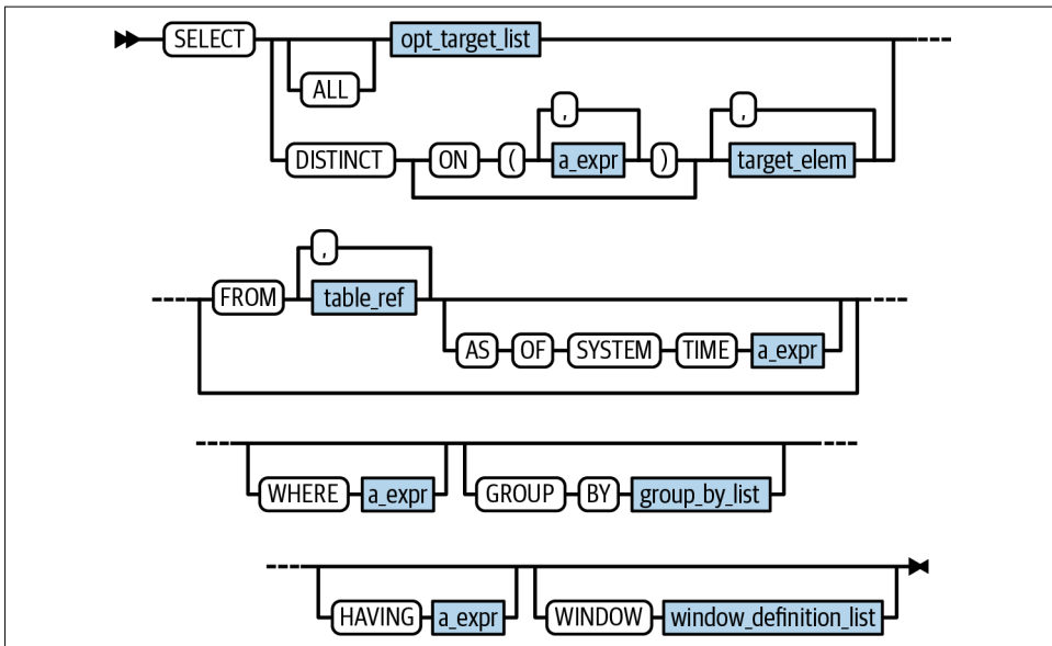
Figure 4-1. SELECT statement
