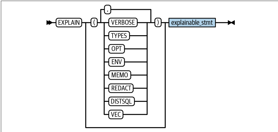
Figure 8-1. EXPLAIN statement syntax
